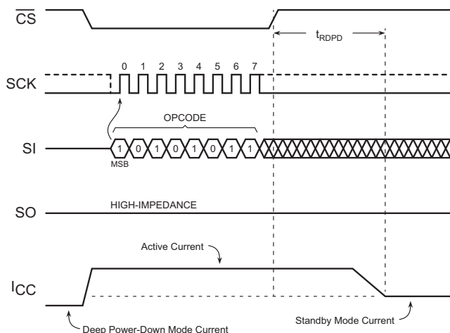
Figure 12-3. Resume from Deep Power-Down
