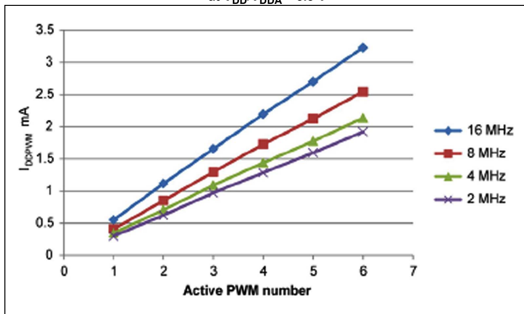
Figure 18. PWM current consumption with f_{\text{SMED}} = \text{HSI } f_{\text{PWM}} = 0.5 \text{ MHz} at V_{\text{DD}}/V_{\text{DDA}} = 5 \text{ V}
