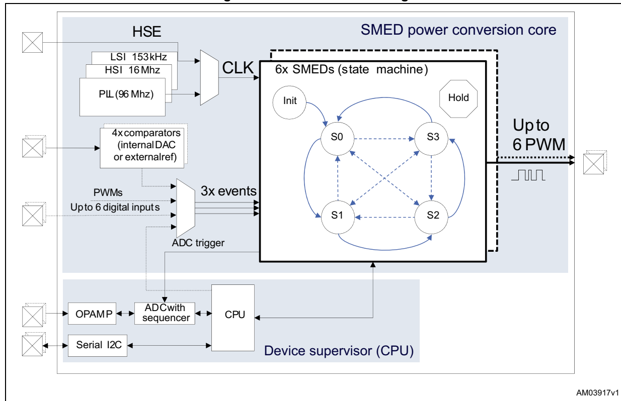
Figure 1. STNRG internal design
