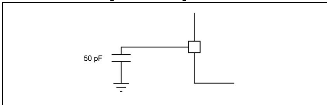
Figure 12. Pin loading conditions
