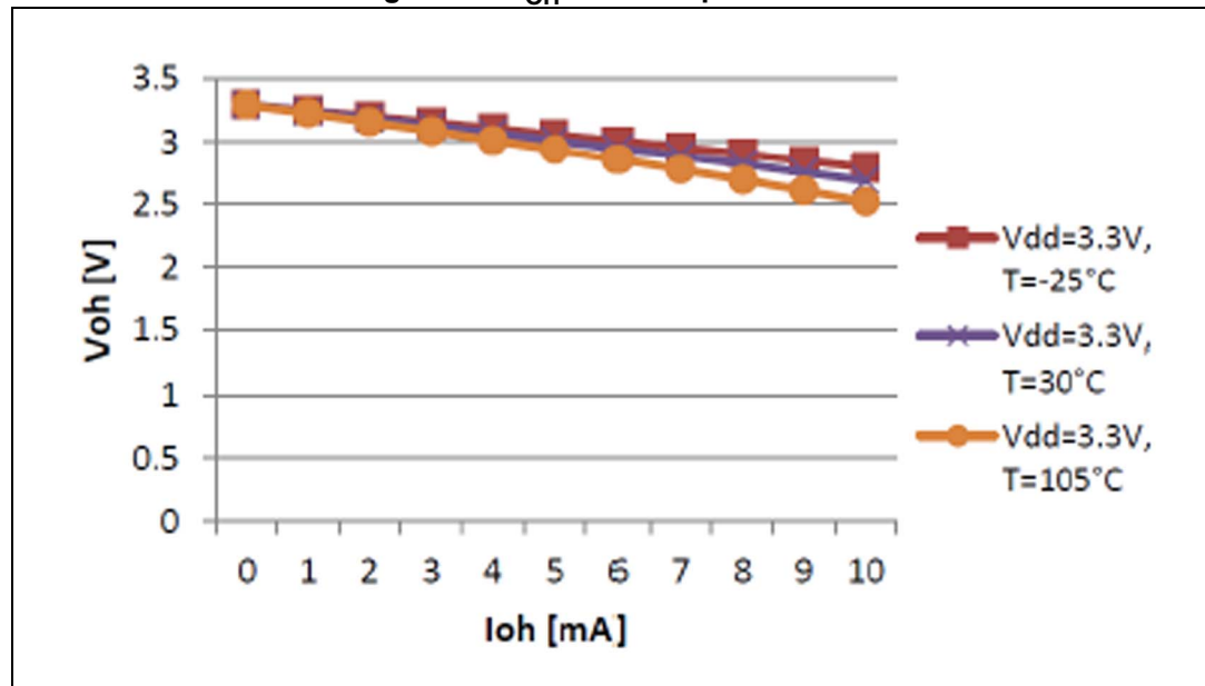
Figure 21. V_{OH} standard pad at 3.3 V
