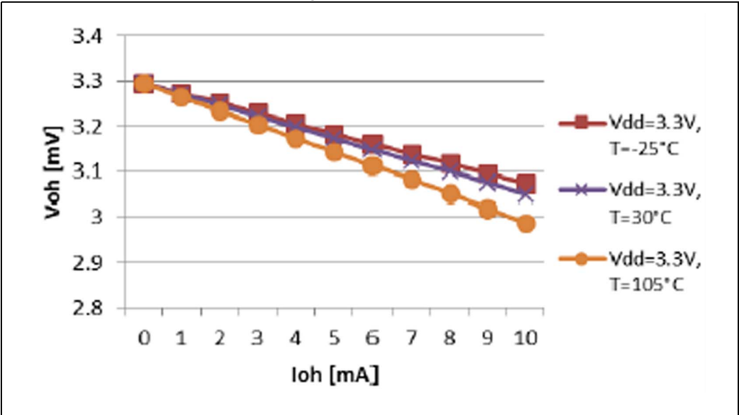
Figure 29. V_{OH} high speed pad at 3.3 V
