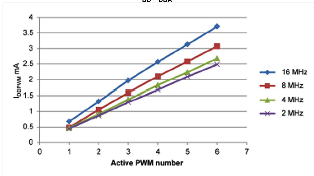
Figure 18. PWM current consumption with f_{\text{SMED}} = \text{HSI } f_{\text{PWM}} = 0.5 \text{ MHz} at V_{\text{DD}}/V_{\text{DDA}} = 5 \text{ V}
