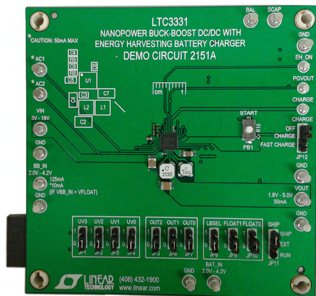
Figure 1. DC2151A Demoboard
