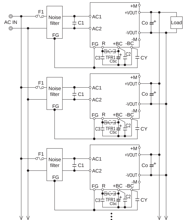
Fig. 5.2 Parallel operation
