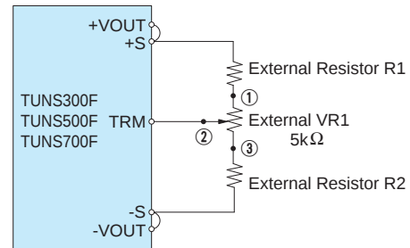
Fig. 4.4 Connecting External Devices (TUNS300F/TUNS500F/TUNS700F)
