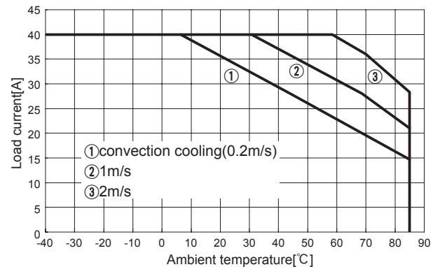
Fig.8.17 Load current vs. ambient temperature(CHS2004805 Vin=48V)
