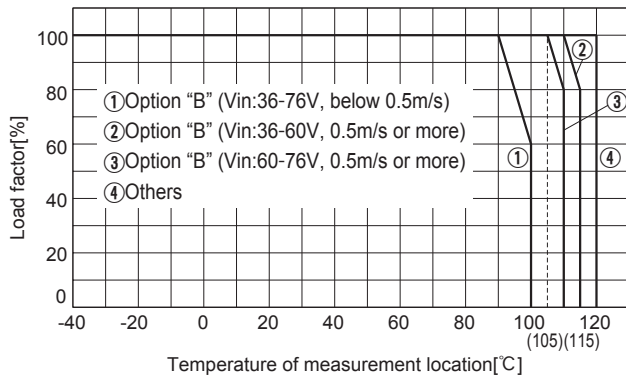
(c) CHS12048
