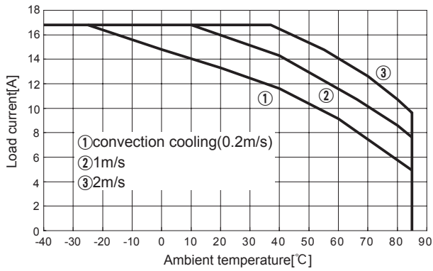
Fig.8.20 Load current vs. ambient temperature(CHS3002412 Vin=24V)
