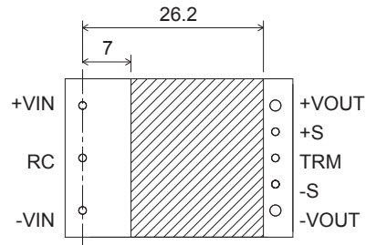
(c) CHS120
