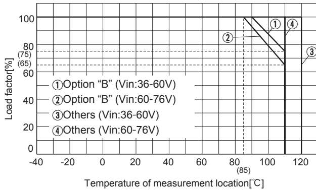
(e) CHS3804810
