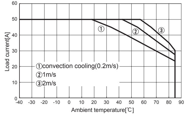
Fig.8.16 Load current vs. ambient temperature(CHS200483R3 Vin=48V)
