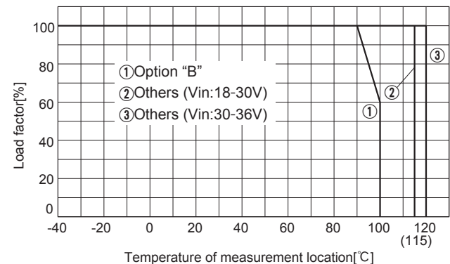
(b) CHS12024
