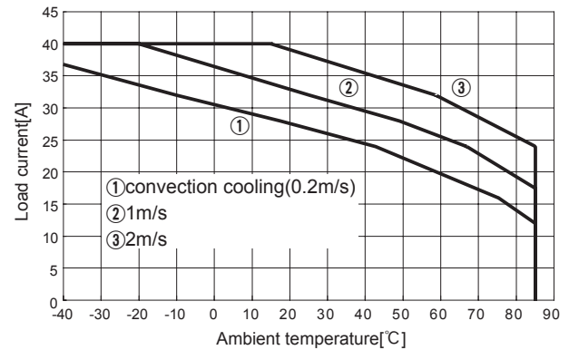
Fig.8.25 Load current vs. ambient temperature(CHS4004810 Vin=48V)
