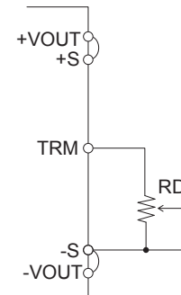
Fig.4.5 Connection to decrease output voltage
