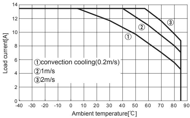
Fig.8.21 Load current vs. ambient temperature(CHS3002415 Vin=24V)
