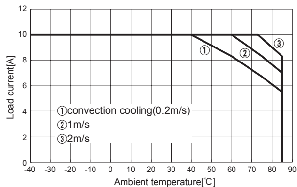
Fig.8.15 Load current vs. ambient temperature(CHS1204812 Vin=48V)
