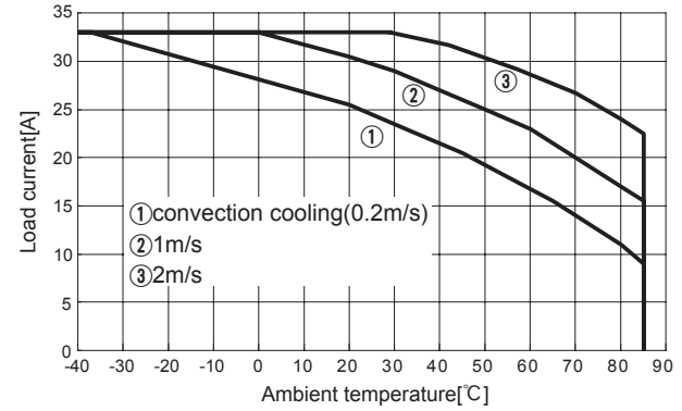
Fig.8.26 Load current vs. ambient temperature(CHS4004812 Vin=48V)
