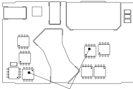
Fig.8.2.7 Temperature measurement location (CHS400)
