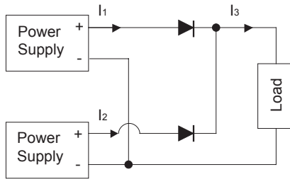
Fig.5.3 Redundancy operation
