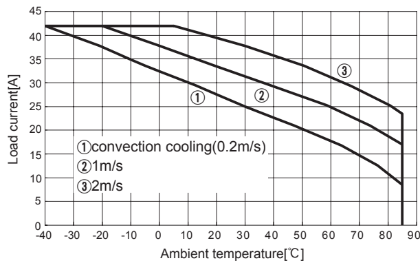
Fig.8.28 Load current vs. ambient temperature(CHS5004812 Vin=48V)
