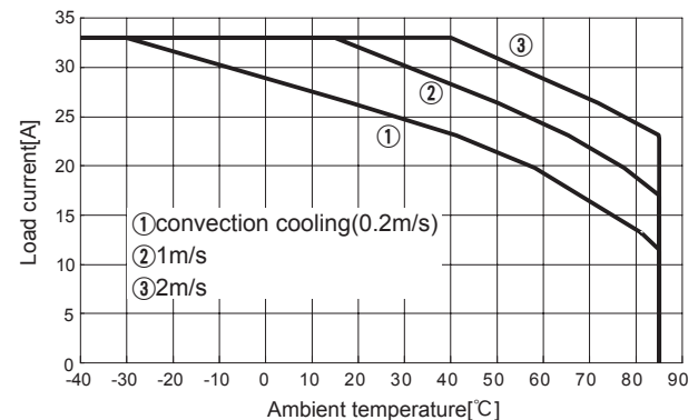
Fig.8.27 Load current vs. ambient temperature(CHS4004812H Vin=48V)
