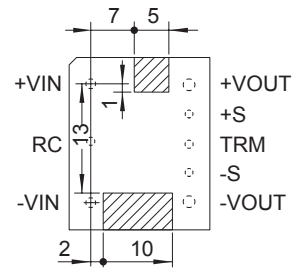
(a) CHS60
