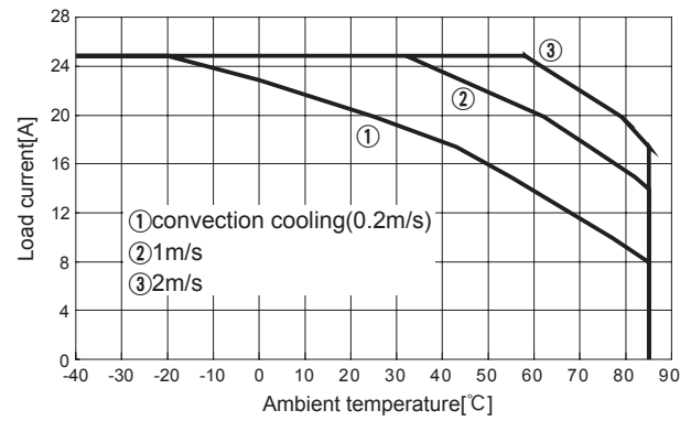
Fig.8.24 Load current vs. ambient temperature(CHS3004812H Vin=48V)
