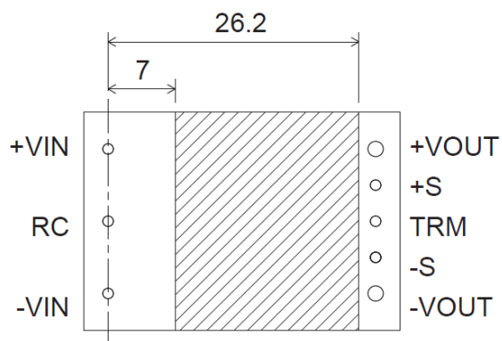
(c) CHS120
