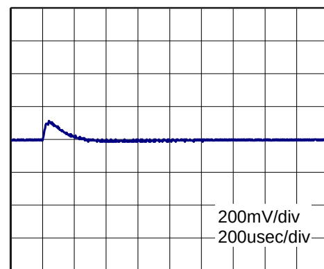
(f) Dynamic Load Response
