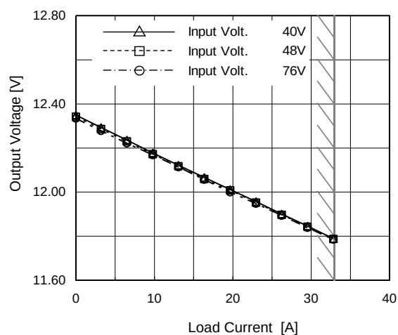
(c) CHS4004812H-P
