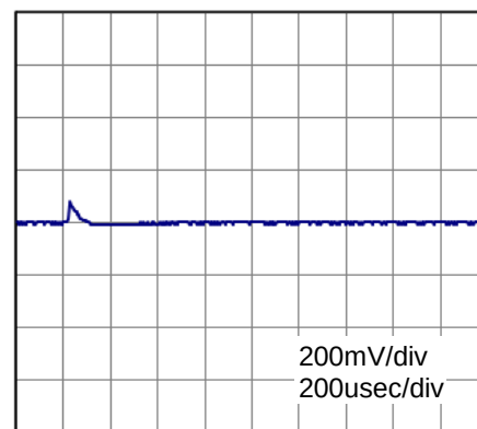
(f) Dynamic Load Response Load 100%(10A)→Load 50%(5A)/50us Vin 48V, Vout 12V
