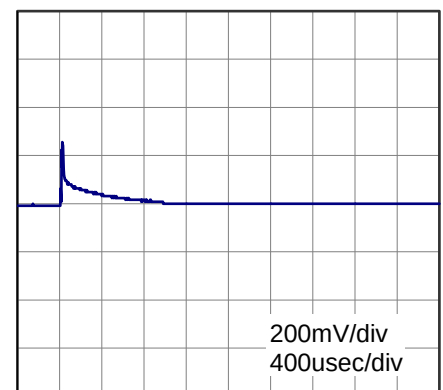
(f) Dynamic Load Response Load 100%(12A)→Load 50%(6A)/50us Vin 48V, Vout 5.0V
