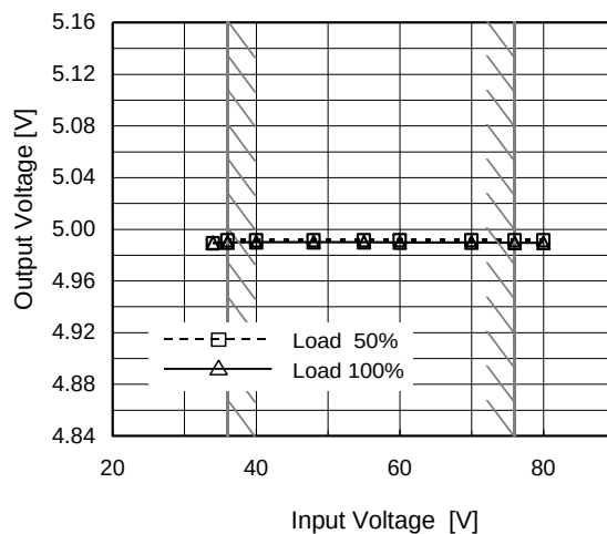
(b) Line Regulation
