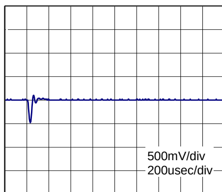
(e) Dynamic Load Response
