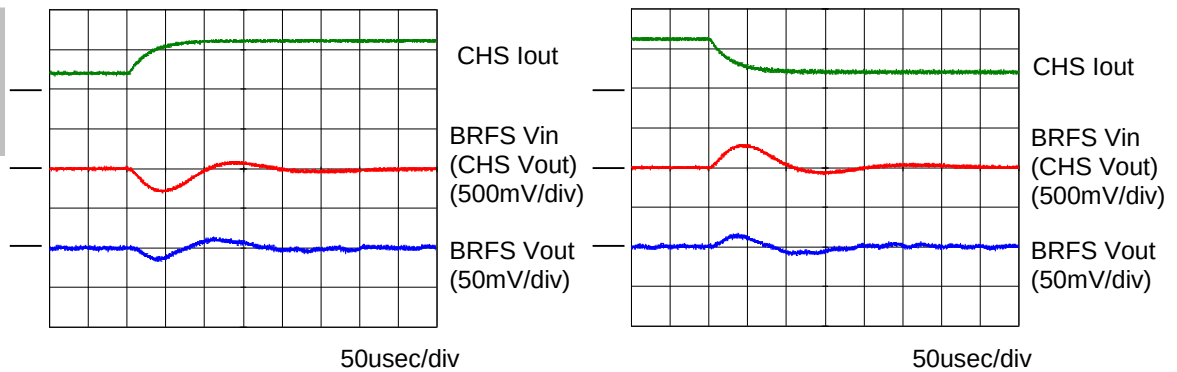
(a) Dynamic Input Response Load 25%(8.25A)→Load 75%(24.75A)/50us
