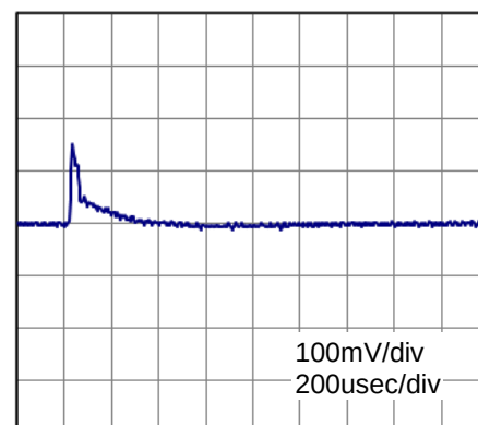
(f) Dynamic Load Response Load 100%(24A)→Load 50%(12A)/50us Vin 48V, Vout 5.0V
