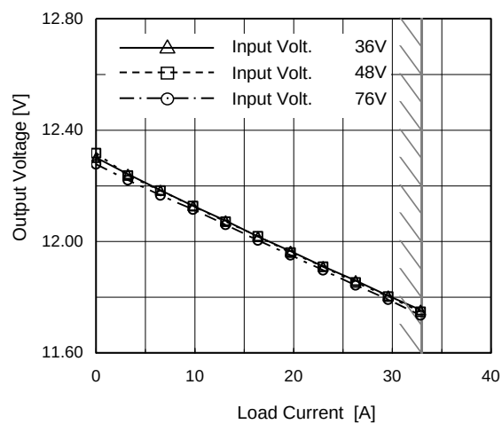
(b) CHS4004812-P
