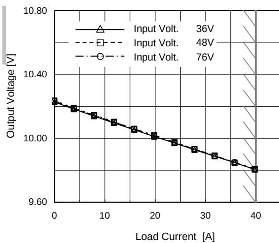
(a) CHS4004810-P
