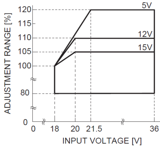
CHS30024
