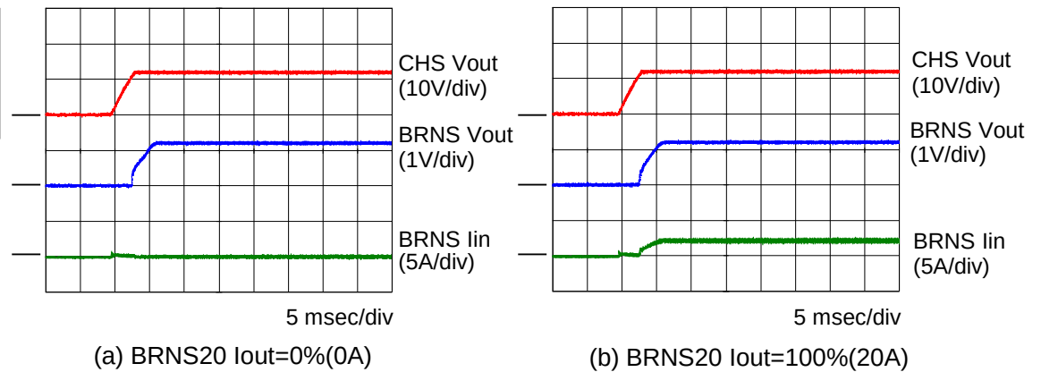
Fig.2.1.1 Startup Sequence of CHS4004812 and BRNS20
