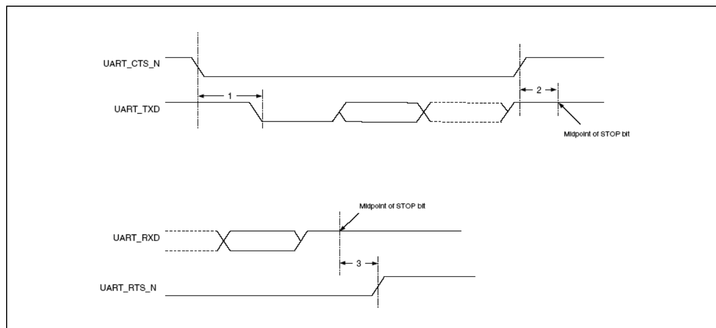
Figure 11. UART Timing
