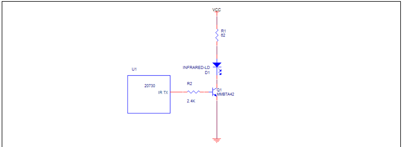
Figure 2. Infrared TX
