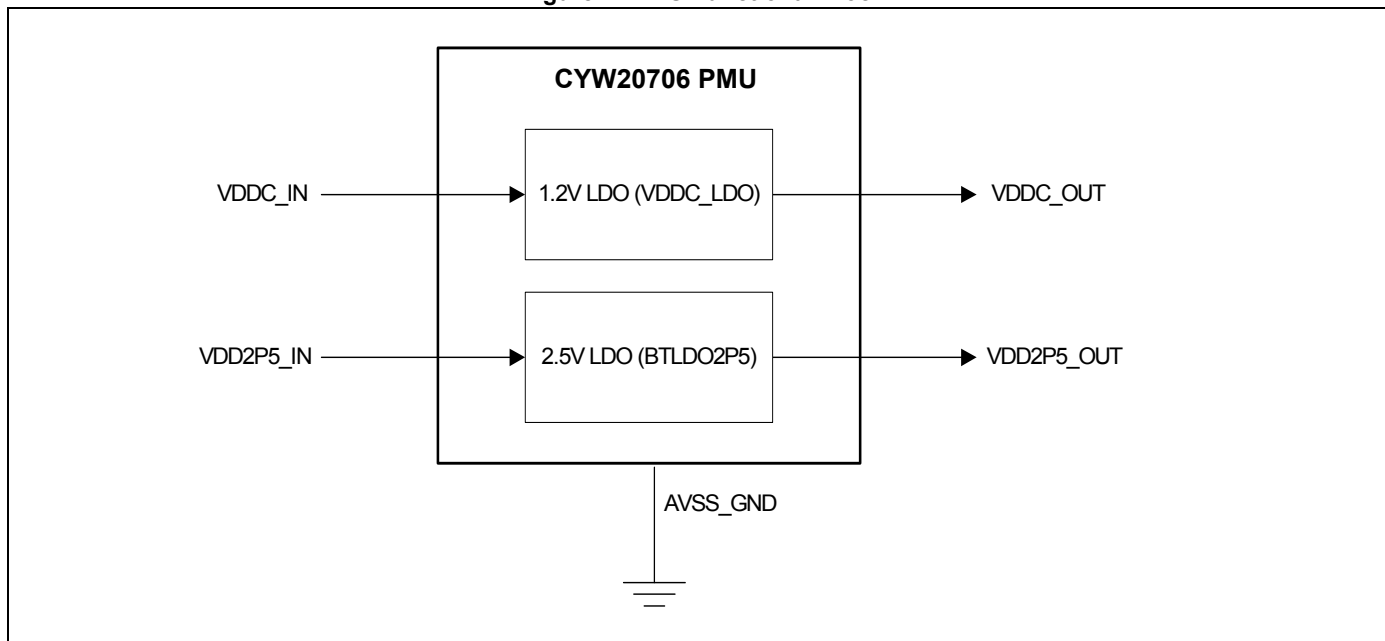
Figure 4. LDO Functional Block
