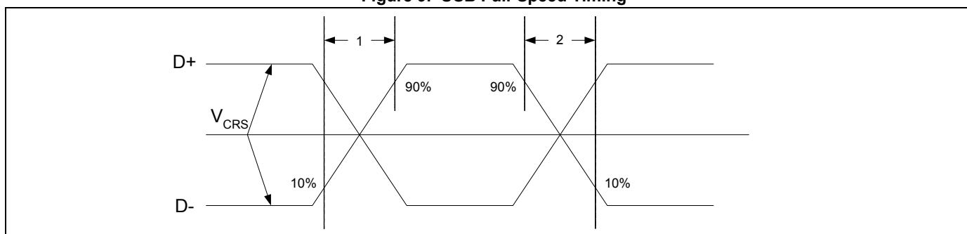
Figure 9. USB Full-Speed Timing
