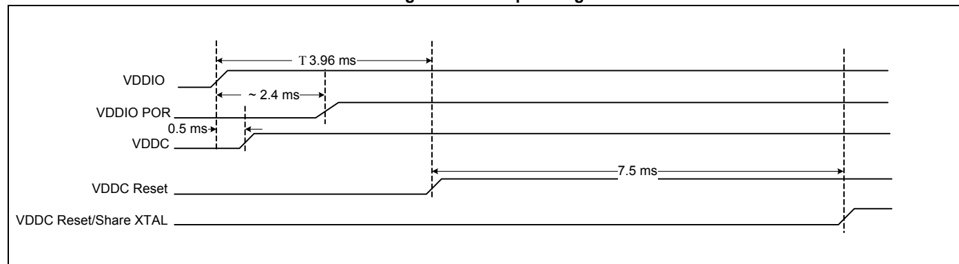
Figure 8. Startup Timing
