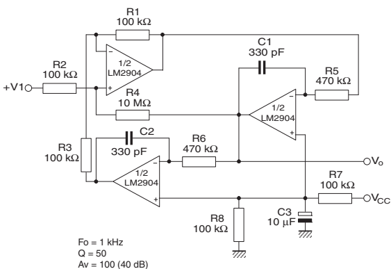
Figure 27. Active bandpass filter
