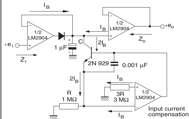
Figure 26. Low drift peak detector
