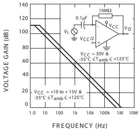
Figure 4. Open-loop frequency response
