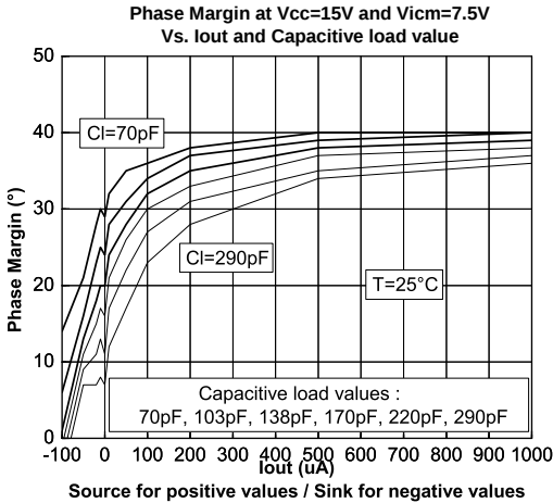
Figure 19. Phase margin vs capacitive load
