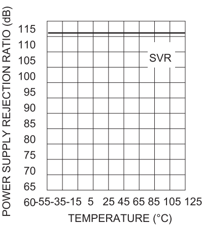
Figure 17. Power supply rejection ratio
