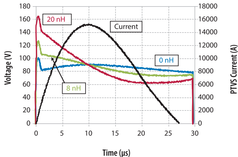
Figure 2. Simulated Effect of Lead Inductance on the Performance of a PTVS Diode
