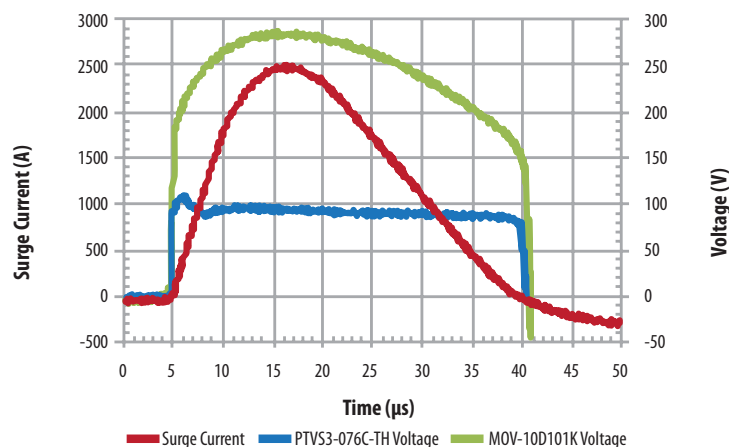
Figure 1. | Comparison of a PTVS Diode and a Metal Oxide Varistor
