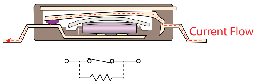
Figure 2. | Mini-breaker in the Normally Closed Position
