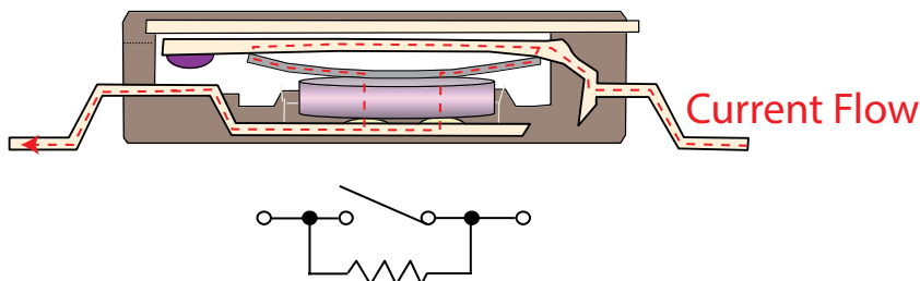
Figure 3. | Mini-breaker Triggered Open
