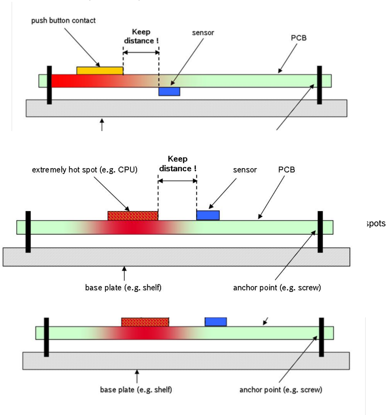
Figure 1: Thermal hot-spots on the PCB
