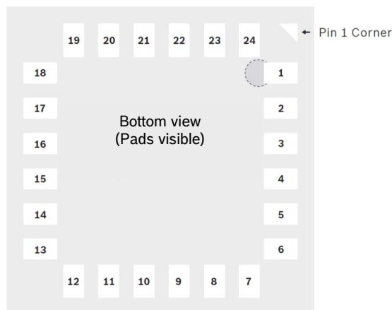
Figure 1: Pin Connections
