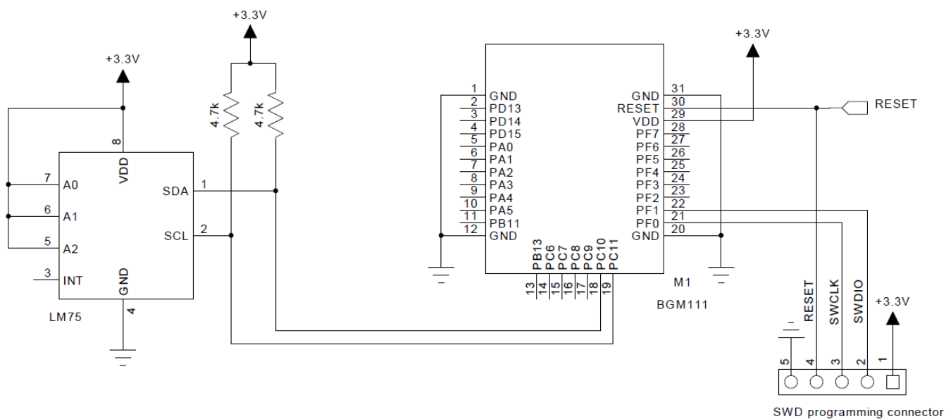
Figure 5.3. BGM111 Module Connected with I2C Device
