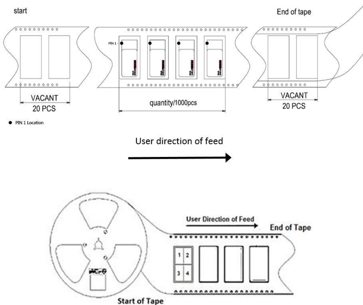
Figure 9.2. Module Orientation and Feed Direction
