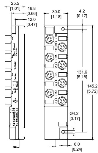
8 Ports 804, 805 Series
