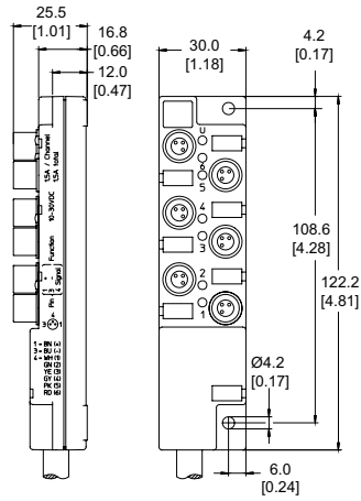
6 Ports 803 Series
