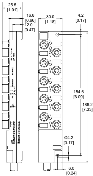
10 Ports 800 Series
