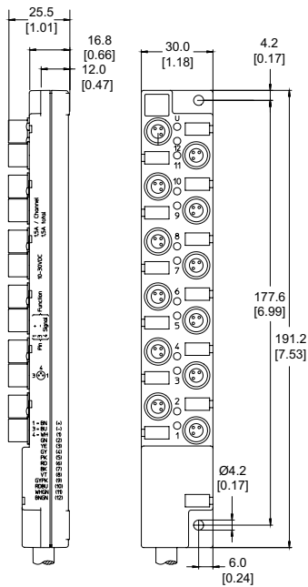
12 Ports 801 Series
