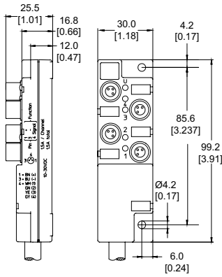
4 Ports 802, 806 Series
