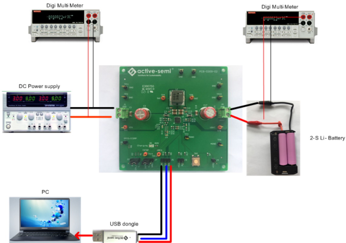
Figure 2 – EVK Setup
