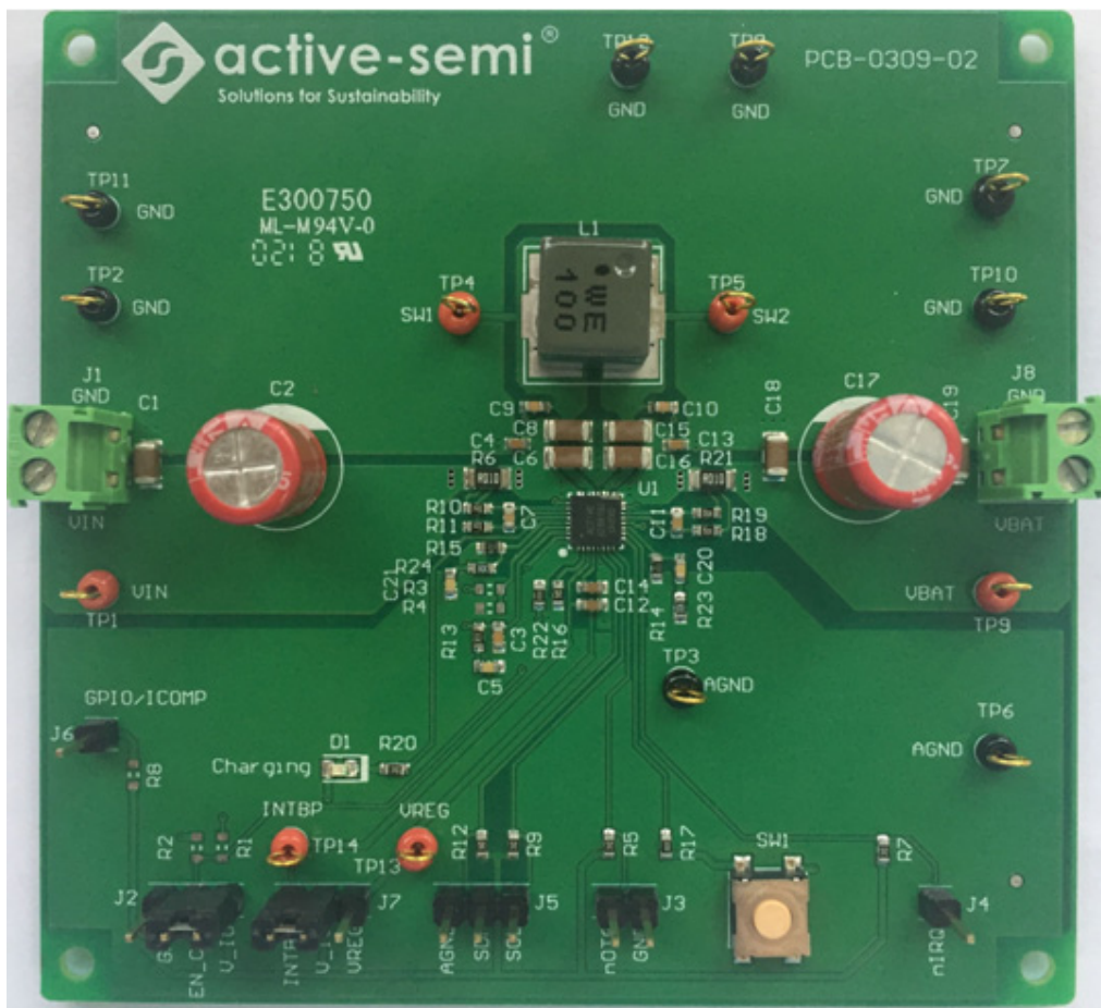
Figure 1 – EVK Picture
