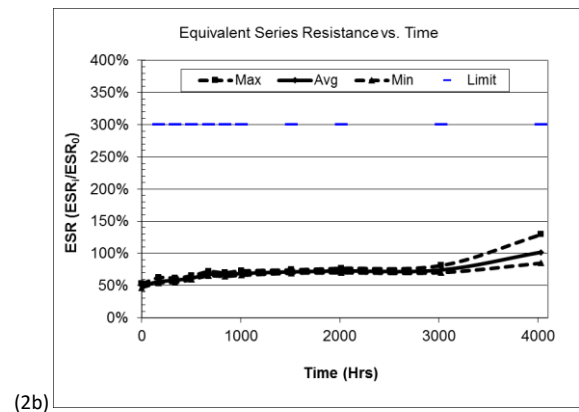
Figures 2a and 2b represent Capacitance vs. Time and Equivalent Series Resistance vs. Time, respectively, for SCMT22C505MRBA0 at 90% rated voltage, otherwise 4.5V, for 4,000 hours at 85°C.
