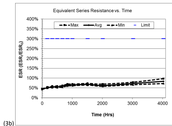
Figures 3a and 3b represent Capacitance vs. Time and Equivalent Series Resistance vs. Time, respectively, for SCMT22C505MRBA0 at 80% rated voltage, otherwise 4.0V, for 4,000 hours at 85°C.
