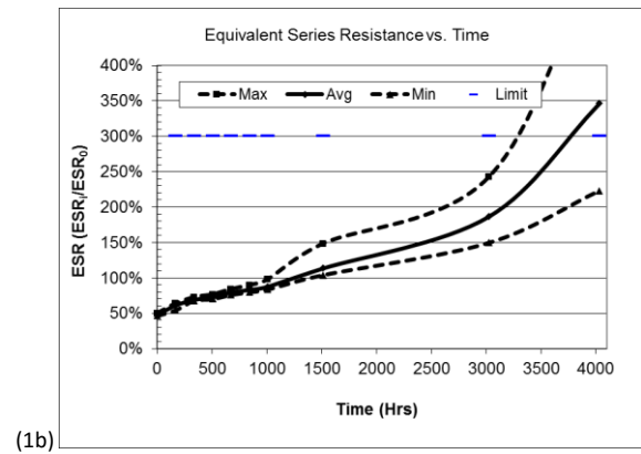
Figures 1a and 1b represent Capacitance vs. Time and Equivalent Series Resistance vs. Time, respectively, for SCMT22C505MRBA0 at rated voltage for 4,000 hours at 85°C.
