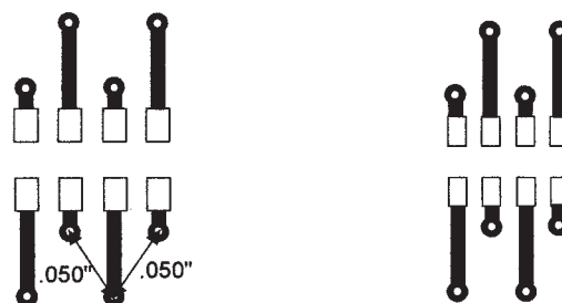
Fig. 6 - IDC connection scheme for 50mil minimum pitch
