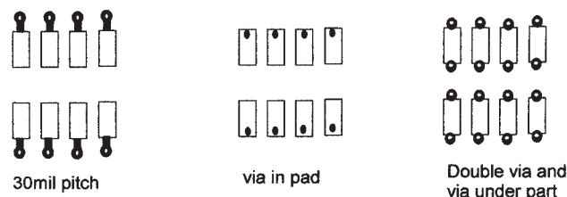
Fig. 7 - Variety of IDC attachment schemes
