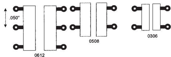
Fig. 4 - Different via schemes for reverse geometry
