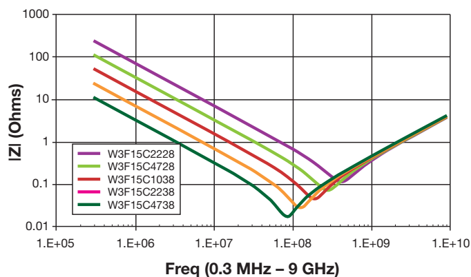
IMPEDANCE 1206 – 50V
