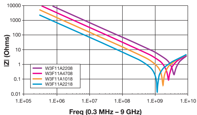
IMPEDANCE 1206 – 100V
