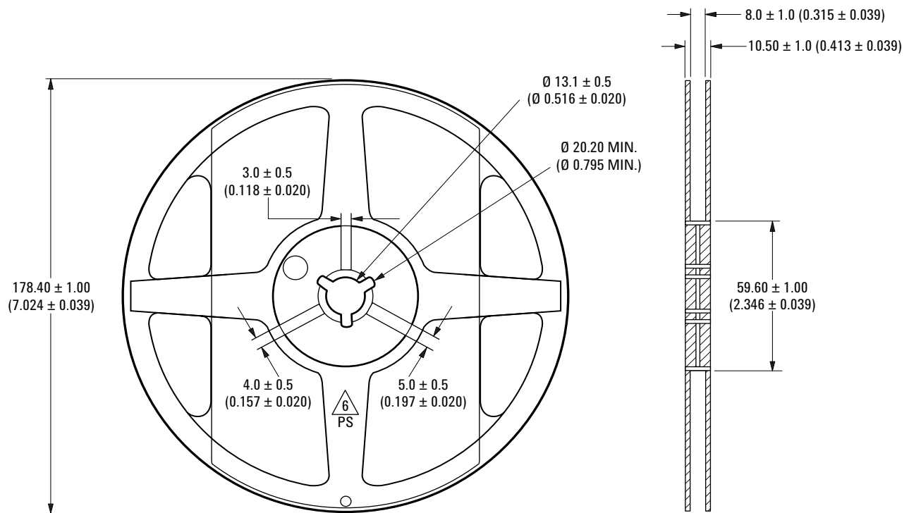
Figure 10. Reel dimensions.
