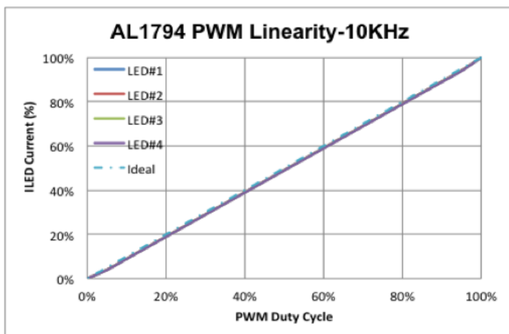
Figure 7: 10KHz PWM Dimming Performance
