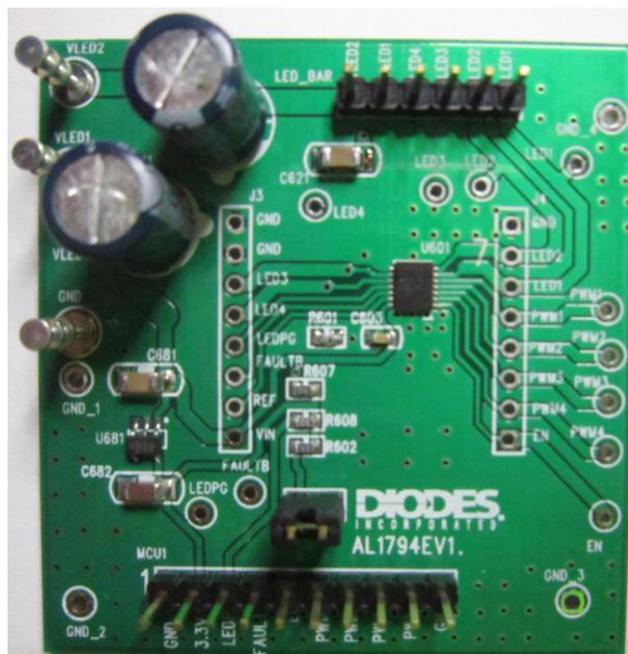
Figure 1: Top View
