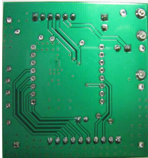
Figure 2: Bottom View
