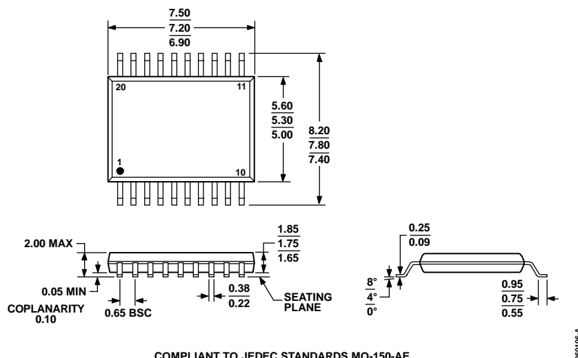
Figure 19. 20-Lead Shrink Small Outline Package [SSOP] (RS-20)
