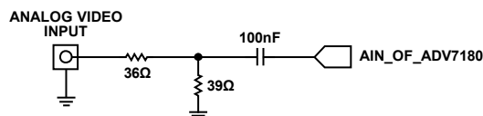
Figure 29. Input Voltage Divider Network
