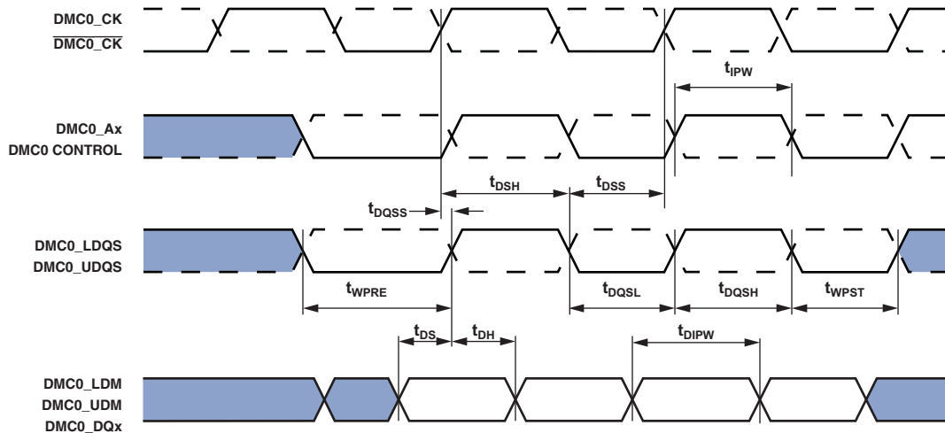
Figure 19. DDR2 SDRAM Controller Output AC Timing
