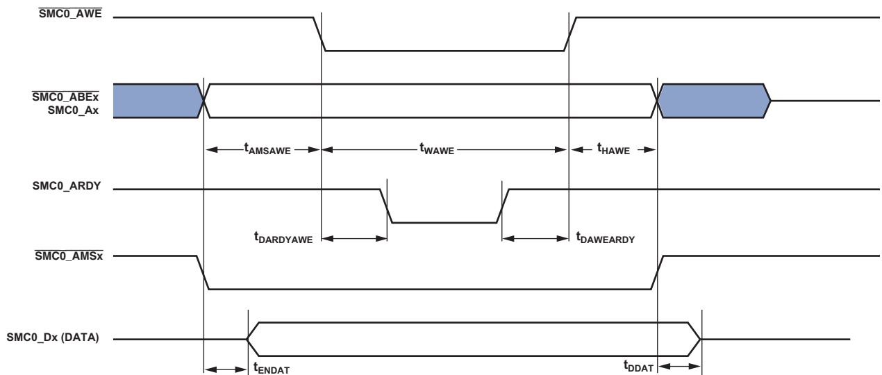
Figure 14. Asynchronous Write
