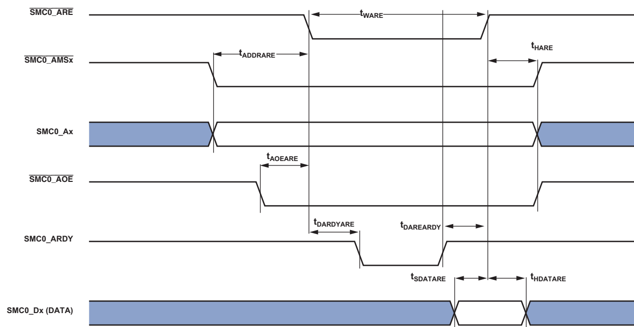
Figure 10. Asynchronous Read
