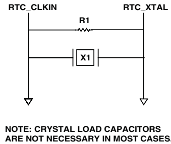
Figure 5. External Components for RTC
