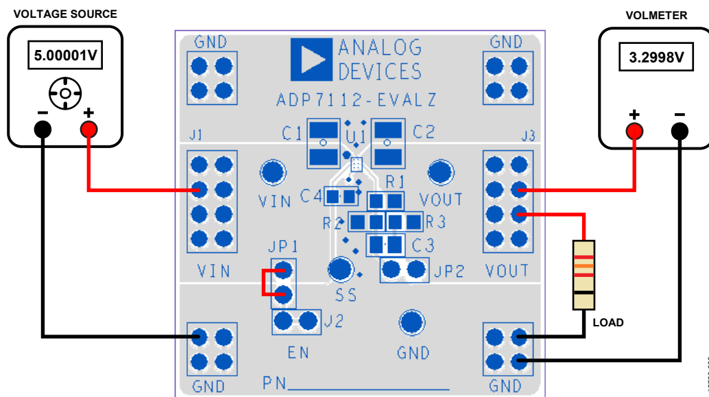
Figure 3. Output Voltage Measurement
