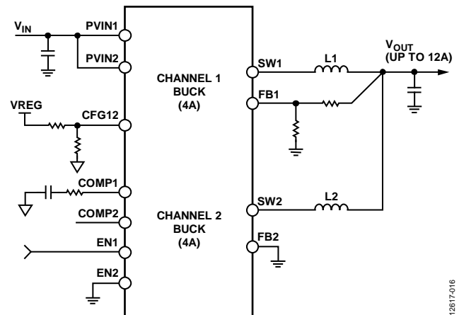
Figure 35. Parallel Operation for Channel 1 and Channel 2
