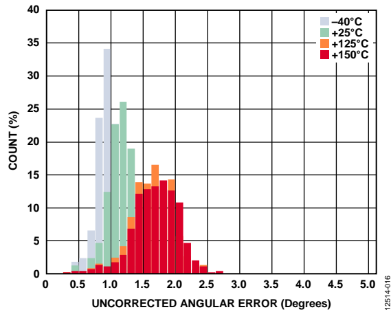
Figure 9. Uncorrected Angular Error, V_{DD} = 5.5\text{ V} , GC = On
