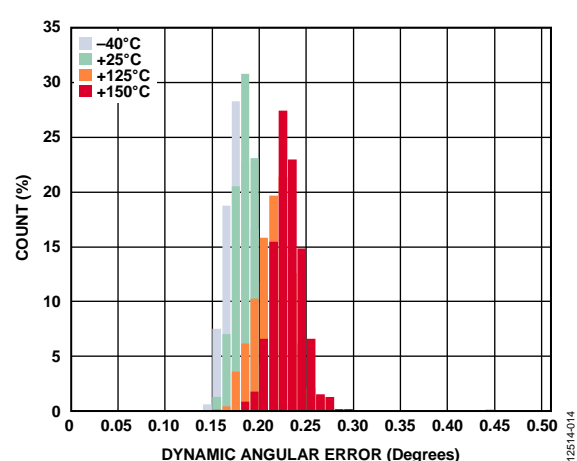
Figure 7. Dynamic Angular Error, V_{DD} = 2.7\text{ V} , GC = \text{On}
