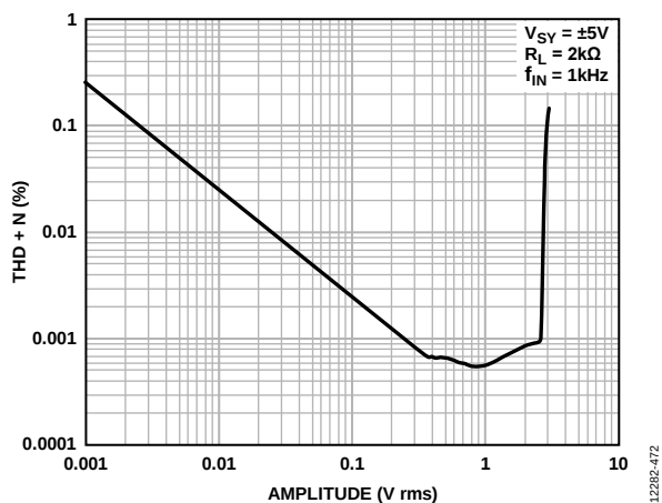
Figure 69. THD + N vs. Amplitude, V_{SV} = \pm 5\text{ V}
