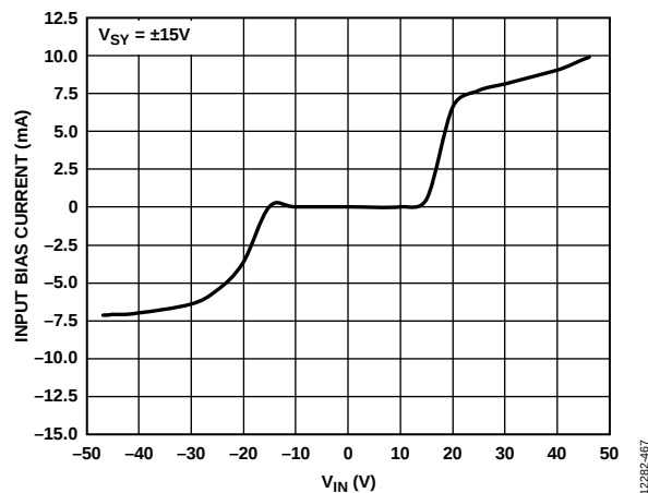
Figure 74. Input Bias Current vs. Input Voltage ( V_{IN} ) Including Input Overvoltage Range (Beyond V_{SV} = \pm 15\text{ V} )
