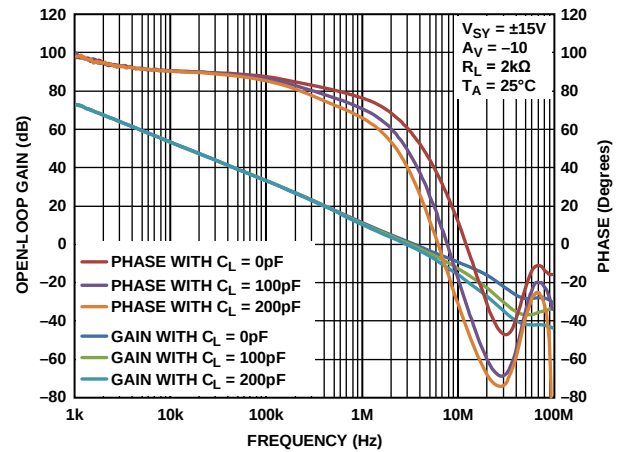
Figure 42. Open-Loop Gain and Phase vs. Frequency, V_{SY} = \pm 15\text{ V}
