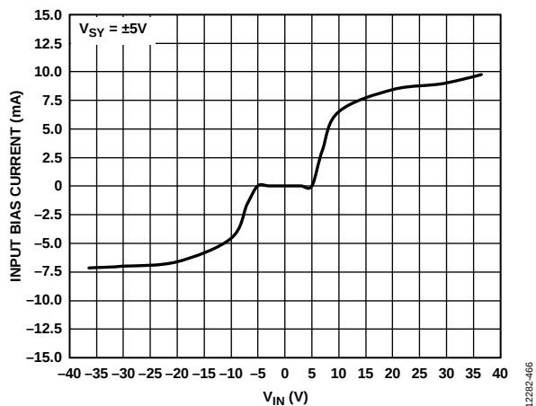
Figure 71. Input Bias Current vs. Input Voltage ( V_{IN} ) Including Input Overvoltage Range (Beyond V_{SV} = \pm 5\text{ V} )
