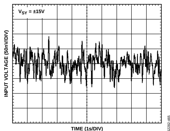
Figure 73. 0.1 Hz to 10 Hz Noise, V_{SV} = \pm 15\text{ V}
