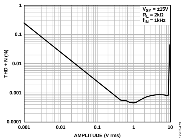
Figure 72. THD + N vs. Amplitude, V_{SV} = \pm 15\text{ V}
