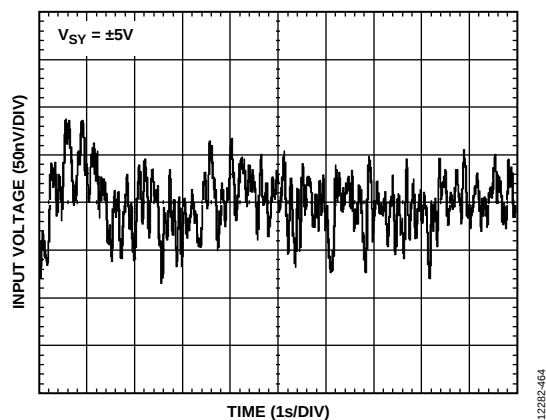
Figure 70. 0.1 Hz to 10 Hz Noise, V_{SV} = \pm 5\text{ V}
