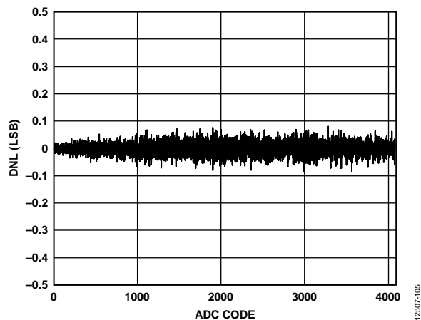
Figure 7. ADC DNL; V_{DD} = 2.7\text{ V}
