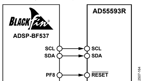
Figure 38. ADSP-BF537 Interface
