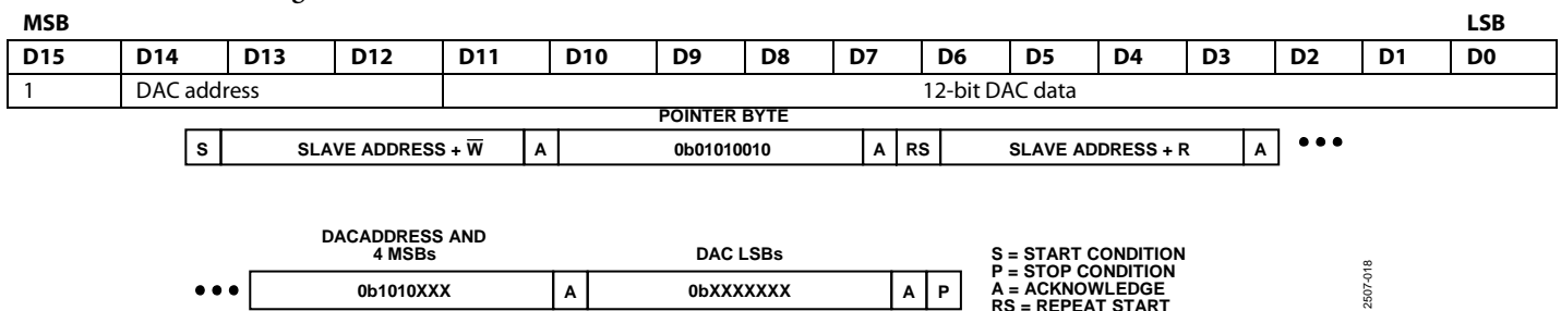
Figure 36. DAC Input Register Readback
