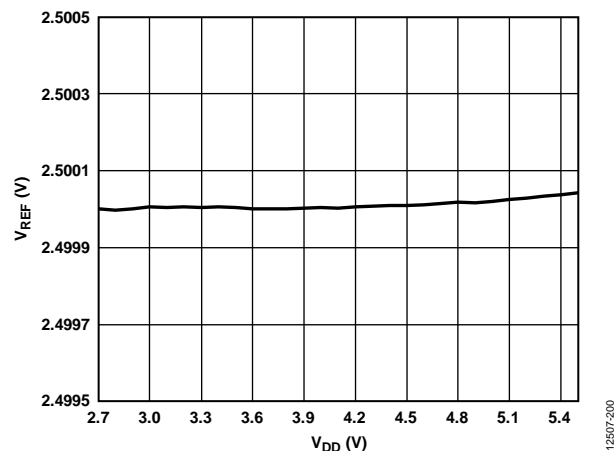
Figure 28. Reference Line Regulation
