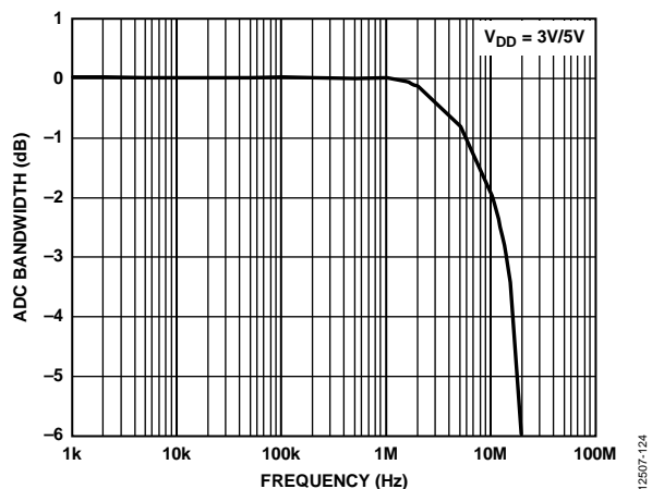
Figure 10. ADC Bandwidth
