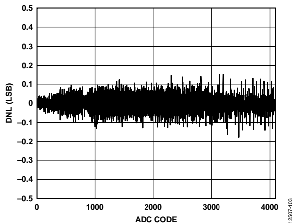
Figure 5. ADC DNL; V_{DD} = 5.5\text{ V}
