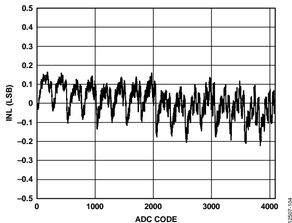
Figure 6. ADC INL; V_{DD} = 2.7\text{ V}
