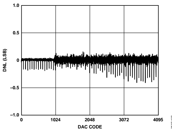
Figure 12. DAC DNL
