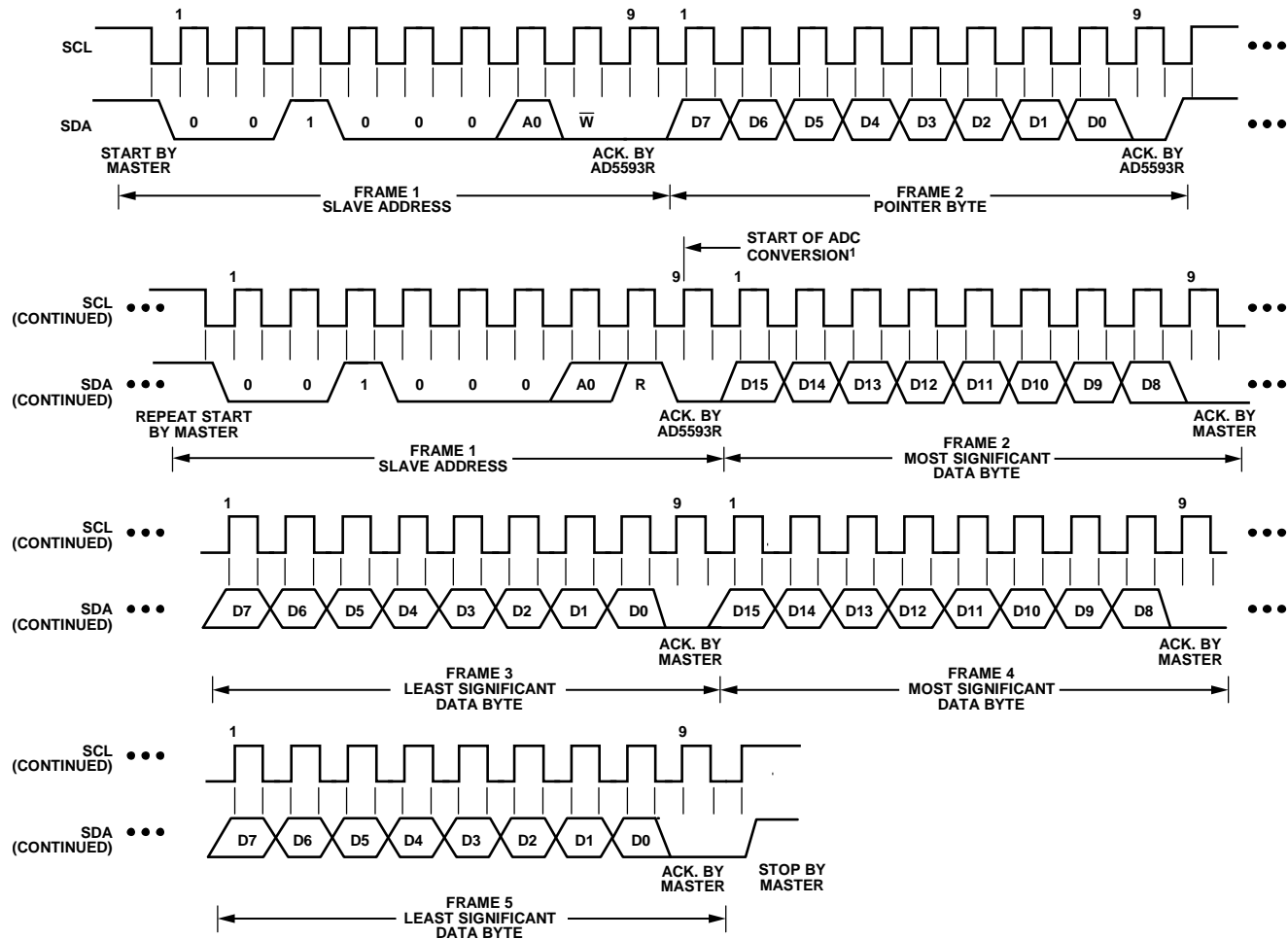
Figure 34. I²C Block Read
