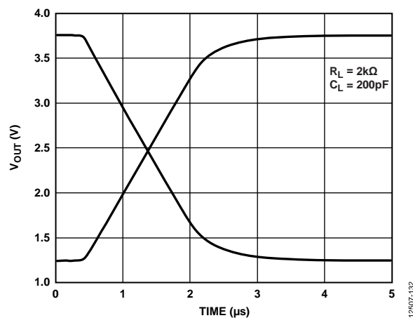
Figure 19. DAC Settling Time, Output Range = 0 V to 2 \times V_{REF}
