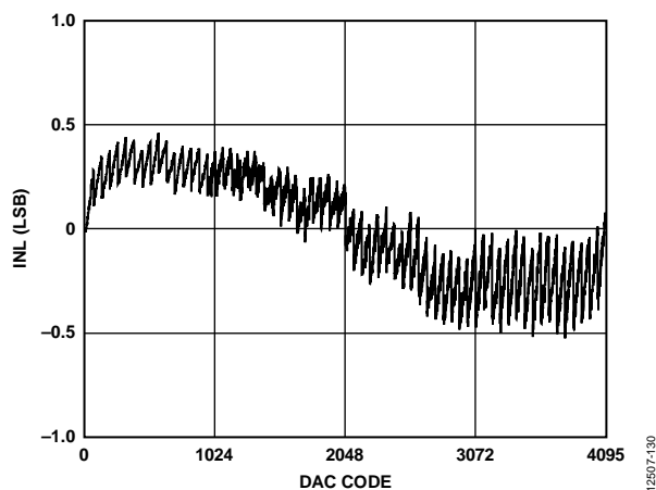
Figure 11. DAC INL
