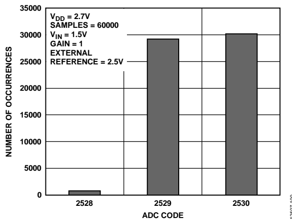
Figure 8. Histogram of ADC Codes; V_{DD} = 2.7\text{ V}
