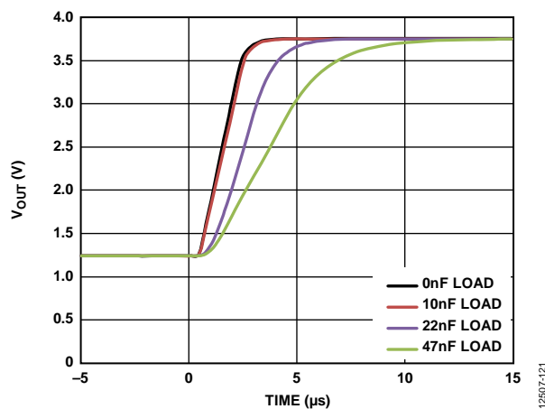
Figure 20. DAC Settling Time vs. Capacitive Load
