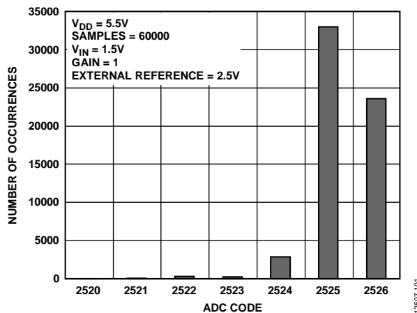
Figure 9. Histogram of Codes; V_{DD} = 5.5\text{ V}
