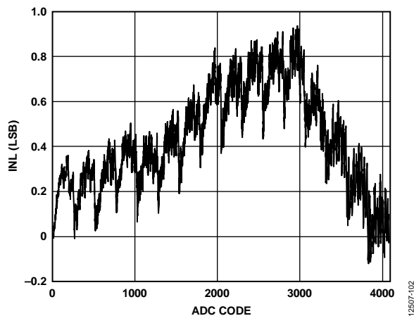
Figure 4. ADC INL; V_{DD} = 5.5\text{ V}
