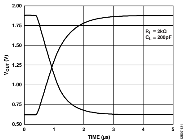
Figure 18. DAC Settling Time, Output Range = 0 V to V_{REF}
