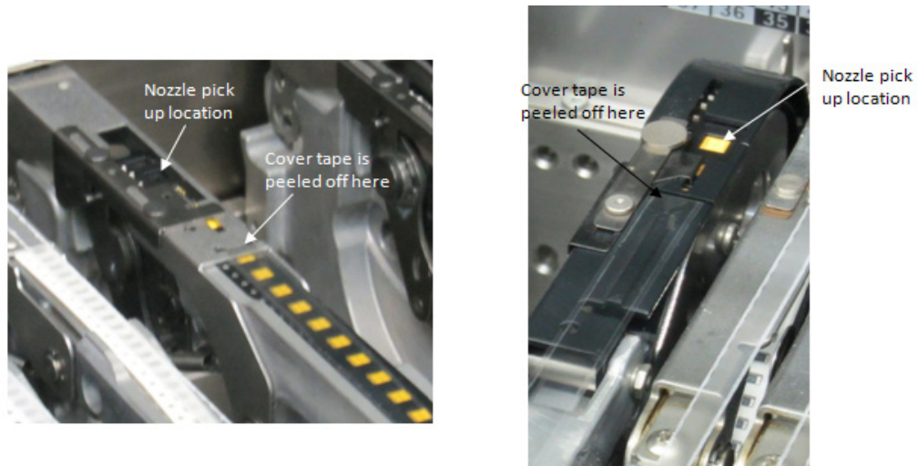
Figure 19. Examples of feeder designs used in LUXEON MZ pick and place study here. Left is Samsung SM421 and right is Juki KE-2080L pick and place feeders.
