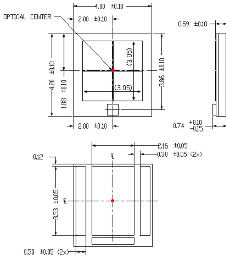
Figure 2. The theoretical optical center of LUXEON MZ is shown as red dot on both the top and bottom drawing of the emitter.
