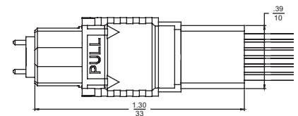
MTP Break-Out Connector
