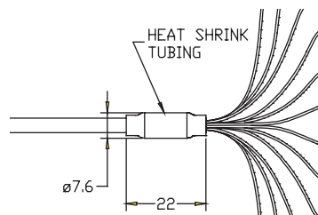
Bare-Ribbon Break-Out Tube
