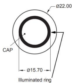
19mm bushing
