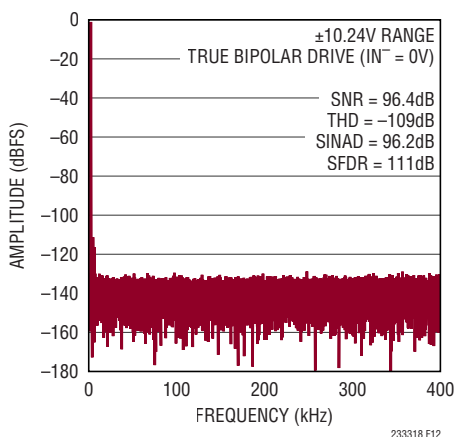
Figure 12. 32k Point FFT f_{\text{SAMPL}} = 800\text{ksps} , f_{\text{IN}} = 2\text{kHz}
