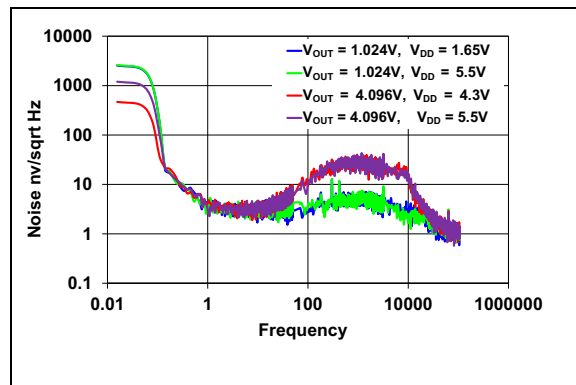
FIGURE 2-12: Noise vs. Frequency, No Load, T_A = +25^{\circ}C .
