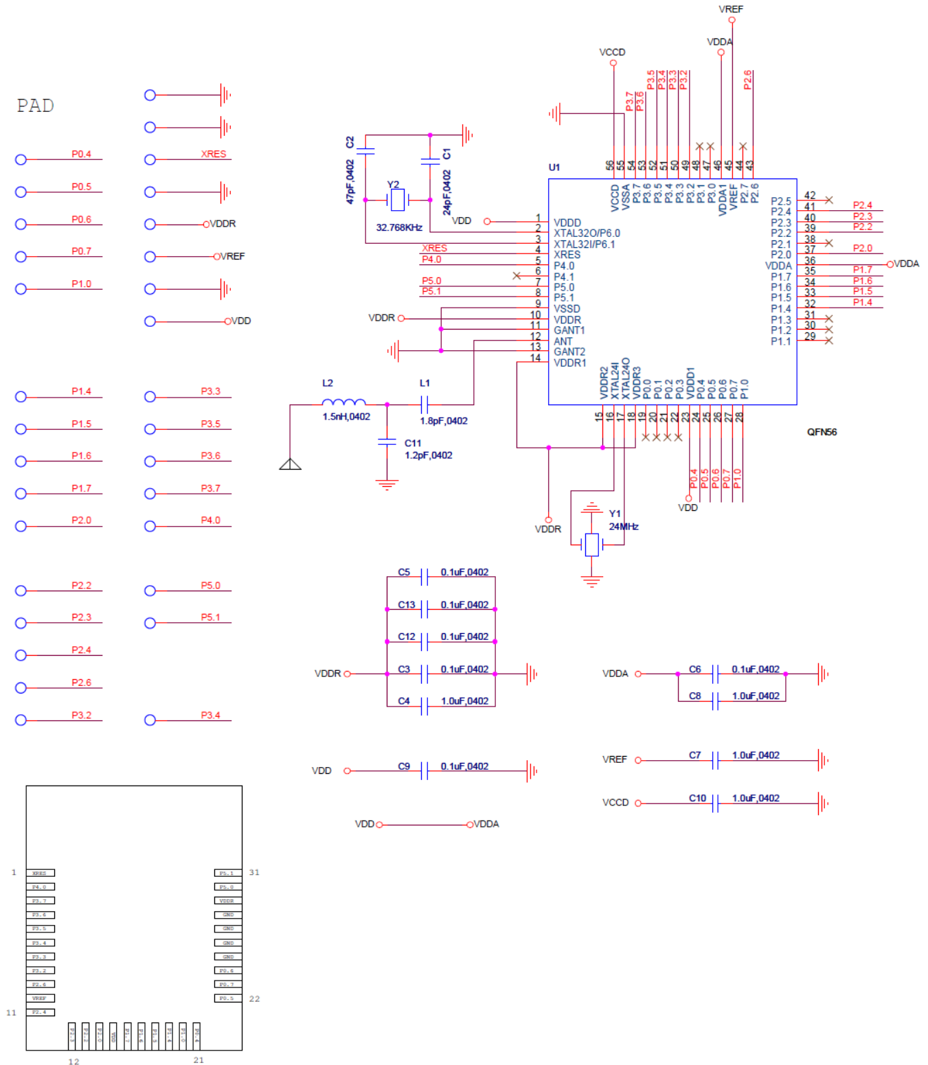
Figure 9. CYBLE-2120XX-X0 Schematic Diagram
