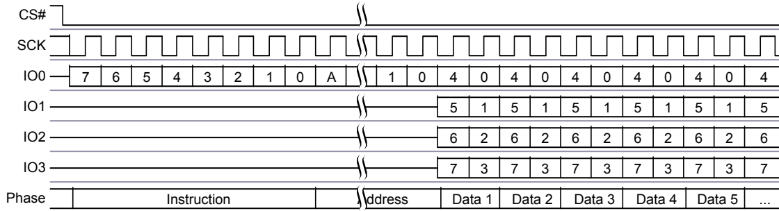
Figure 11.46 Quad Page Program Command Sequence
