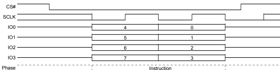
Figure 11.52 Bulk Erase Command Sequence QPI Mode
