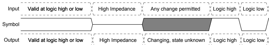
Figure 6.1 Waveform Element Meanings
