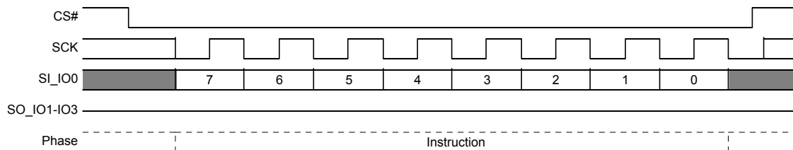
Figure 11.17 Write Disable (WRDI) Command Sequence
