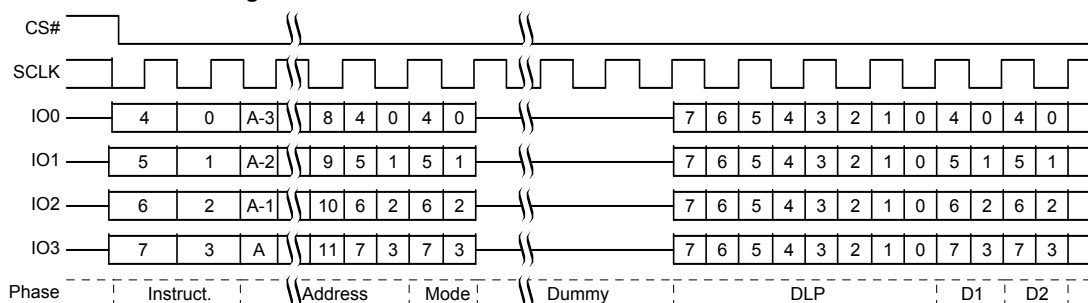
Figure 11.42 DDR Quad I/O Read Initial Access QPI Mode
