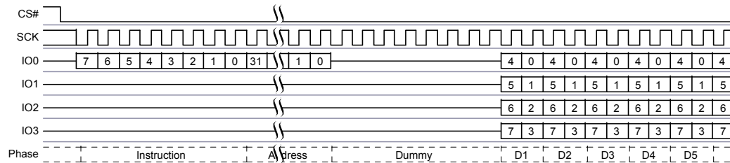
Figure 4.8 Quad Output Read Command
