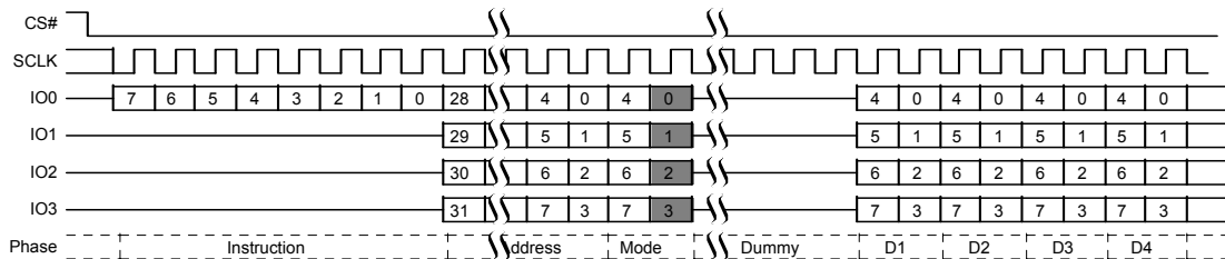
Figure 4.10 Quad I/O Command
