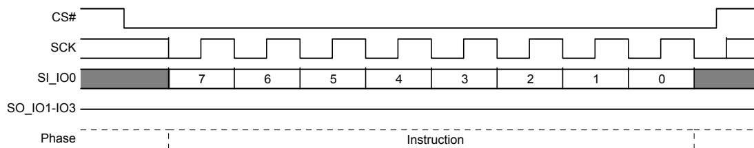
Figure 11.26 Enter 4 Byte Address Mode (4BEN B7h) Command Sequence
