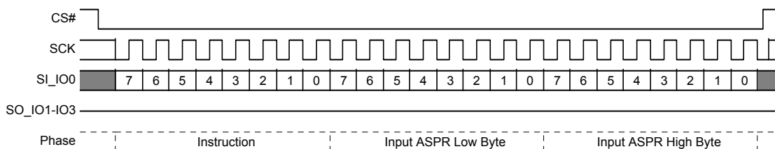
Figure 11.61 ASPP Command
