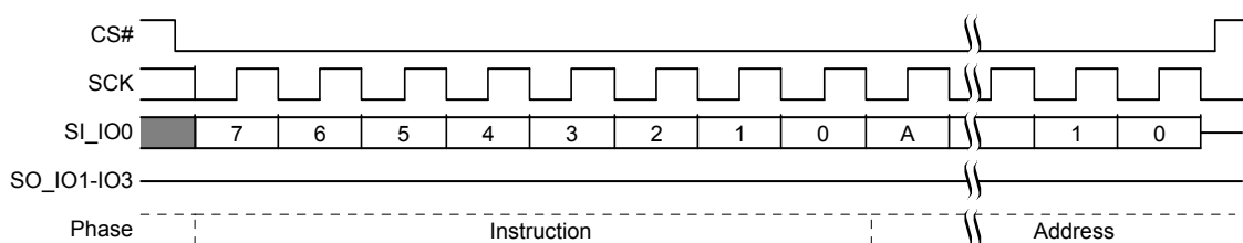
Figure 11.47 Parameter Sector Erase (P4E 20h or 4P4E 21h) Command Sequence
