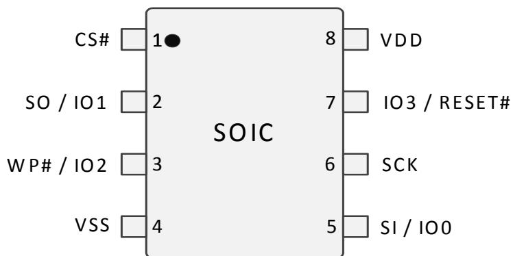
Figure 8.1 8-Pin Plastic Small Outline Package (SOIC8)
