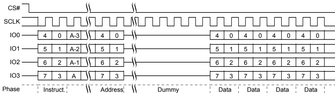
Figure 11.22 ECC Status Register Read QPI Mode, Command Sequence
