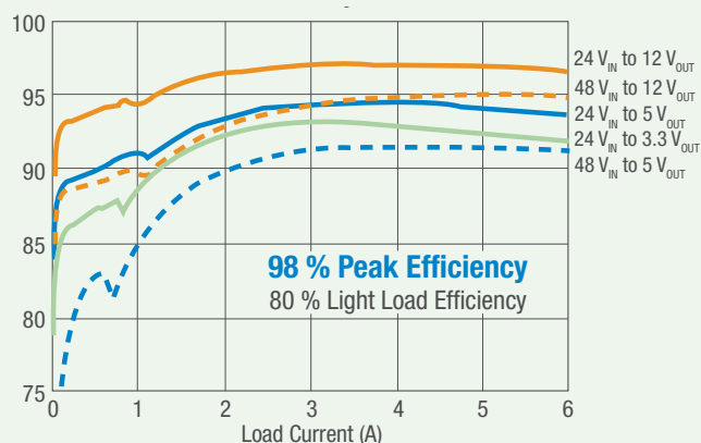
SiC462 Efficiency at 300 kHz
