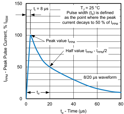
Fig. 4 - 8/20 \mu\text{s} Pulse Waveform
