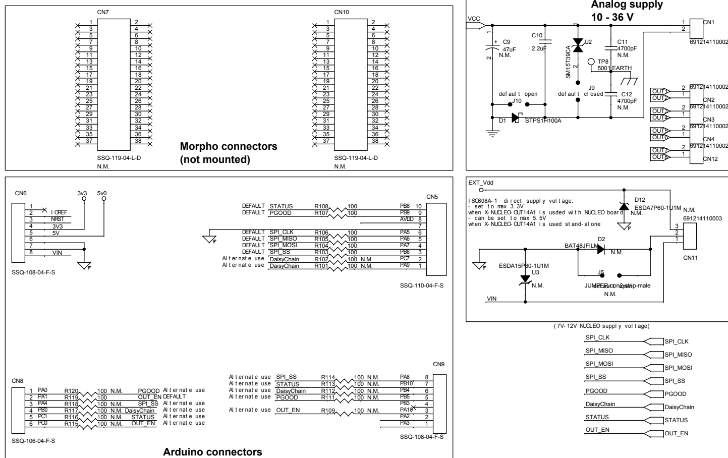
Figure 1. X-NUCLEO-OUT14A1 circuit schematic (1 of 2)
