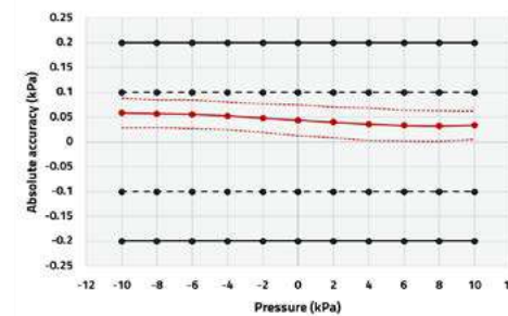
Accuracy 2513130810201 : -10 to 10 kPa Typical Pressure Curve @ Room Temperature
