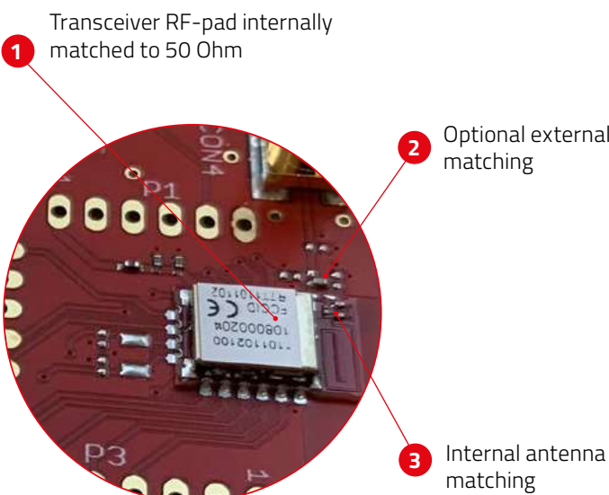
Picture: Evaluation board Thyone-I
