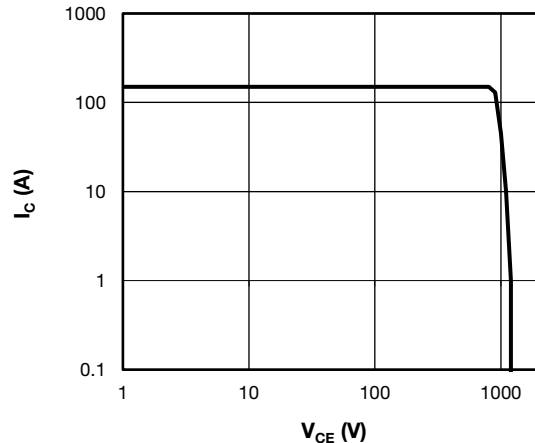
Fig. 16 - Trench IGBT Reverse BIAS SOA T_J = 150\text{ }^{\circ}\text{C} , I_C = 150\text{ A} , R_g = 4.7\text{ }\Omega , V_{GE} = +15\text{ V} / 0\text{ V} , V_{CC} = 800\text{ V} , V_p = 1200\text{ V}
