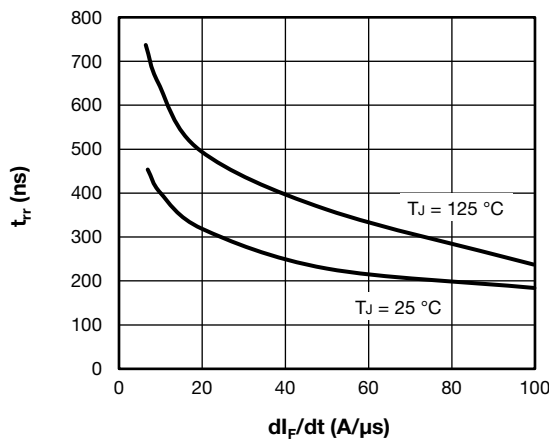
Fig. 13 - Typical Diode Reverse Recovery Time vs. dl_F/dt
