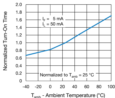
Fig. 8 - Normalized Turn-On Time vs. Ambient Temperature
