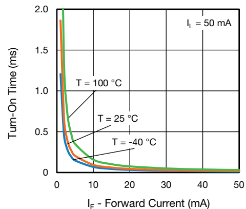
Fig. 10 - Turn-On Time vs. Forward Current
