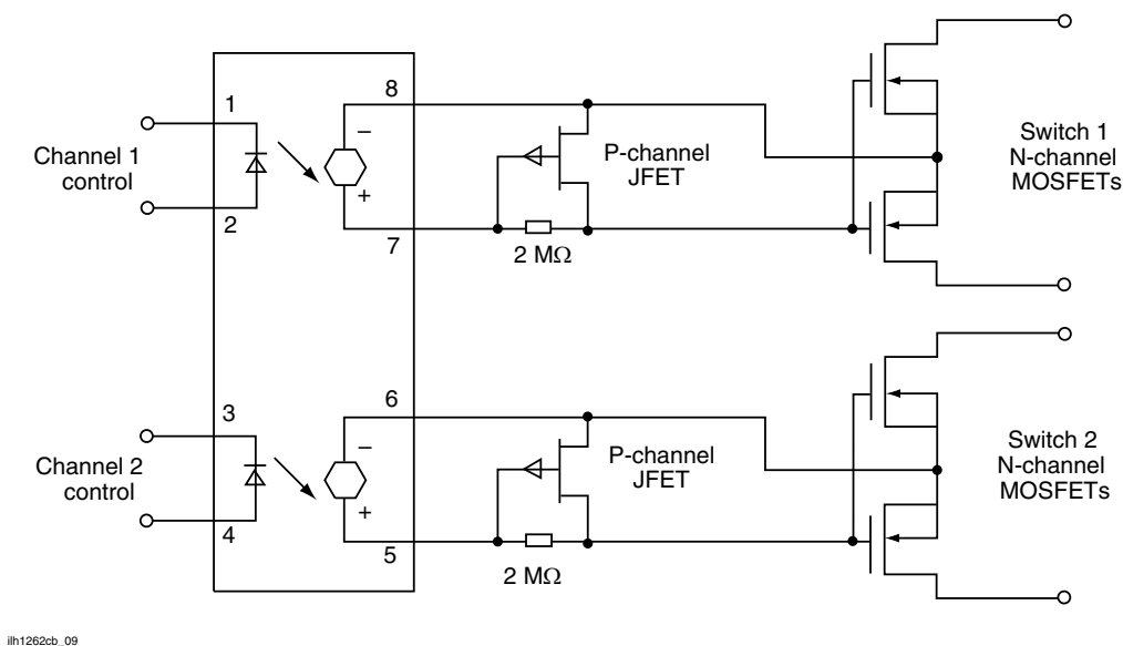
Fig. 12 - Typical Dual Form A Solid-State Relay Application
