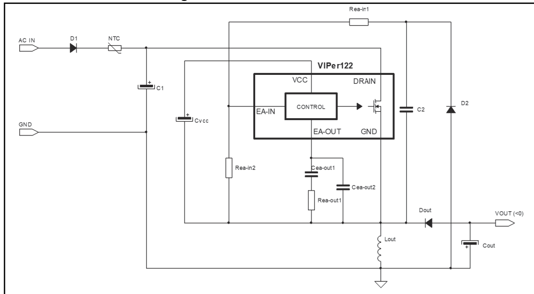
Figure 14. Buck-boost converter
