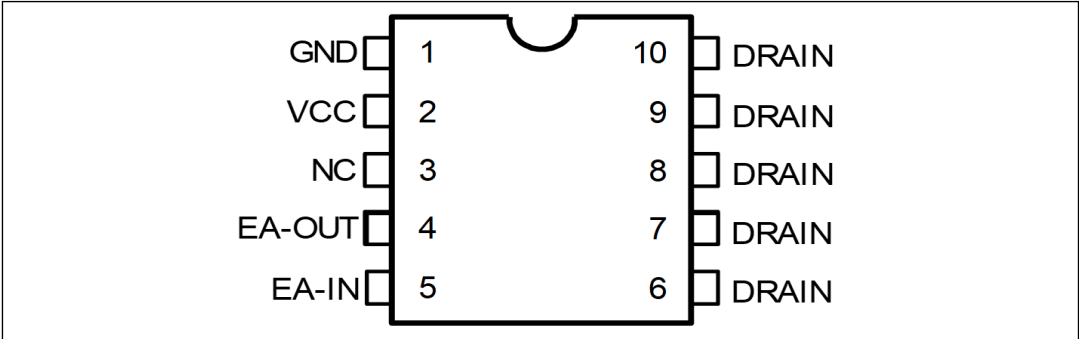
Figure 2. Connection diagram
