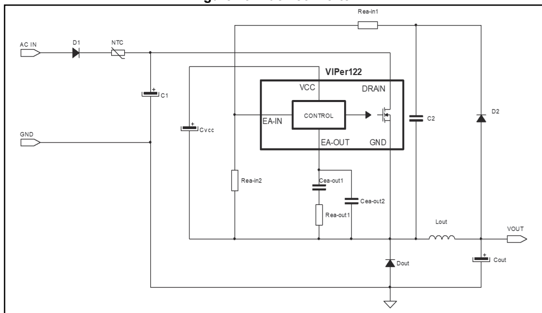
Figure 13. Buck converter
