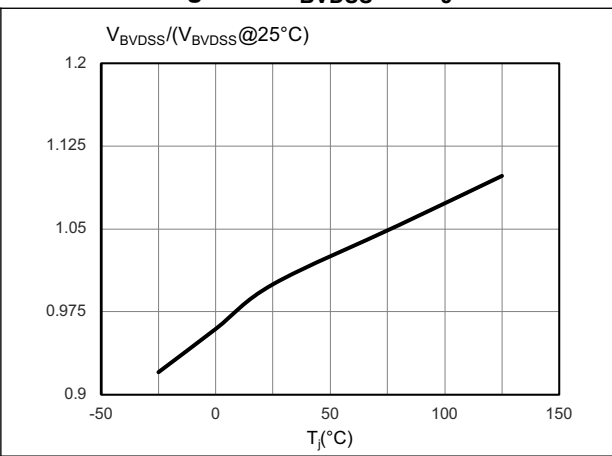
Figure 9. V_{BVDSS} vs. T_J
