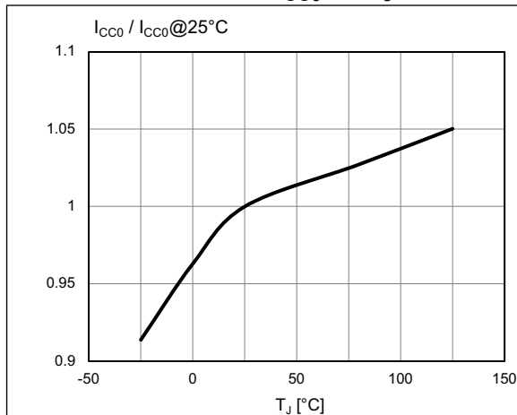
Figure 6. I_{CC0} vs. T_J
