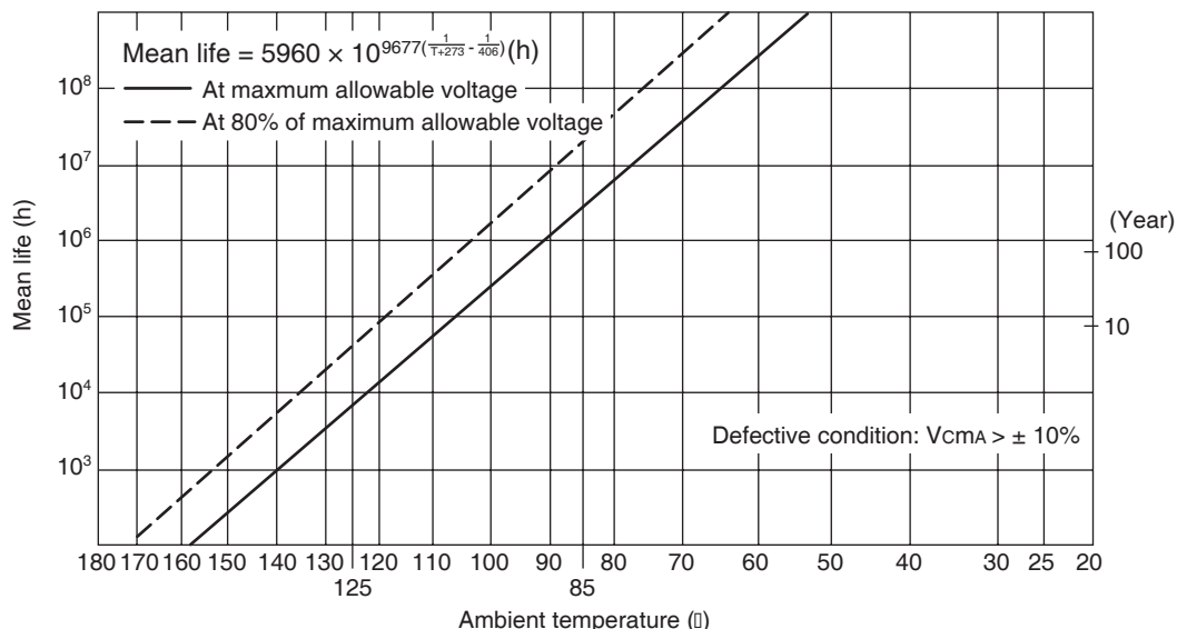
Fig. 4 Relationship between mean life Varistor and ambient temperature
