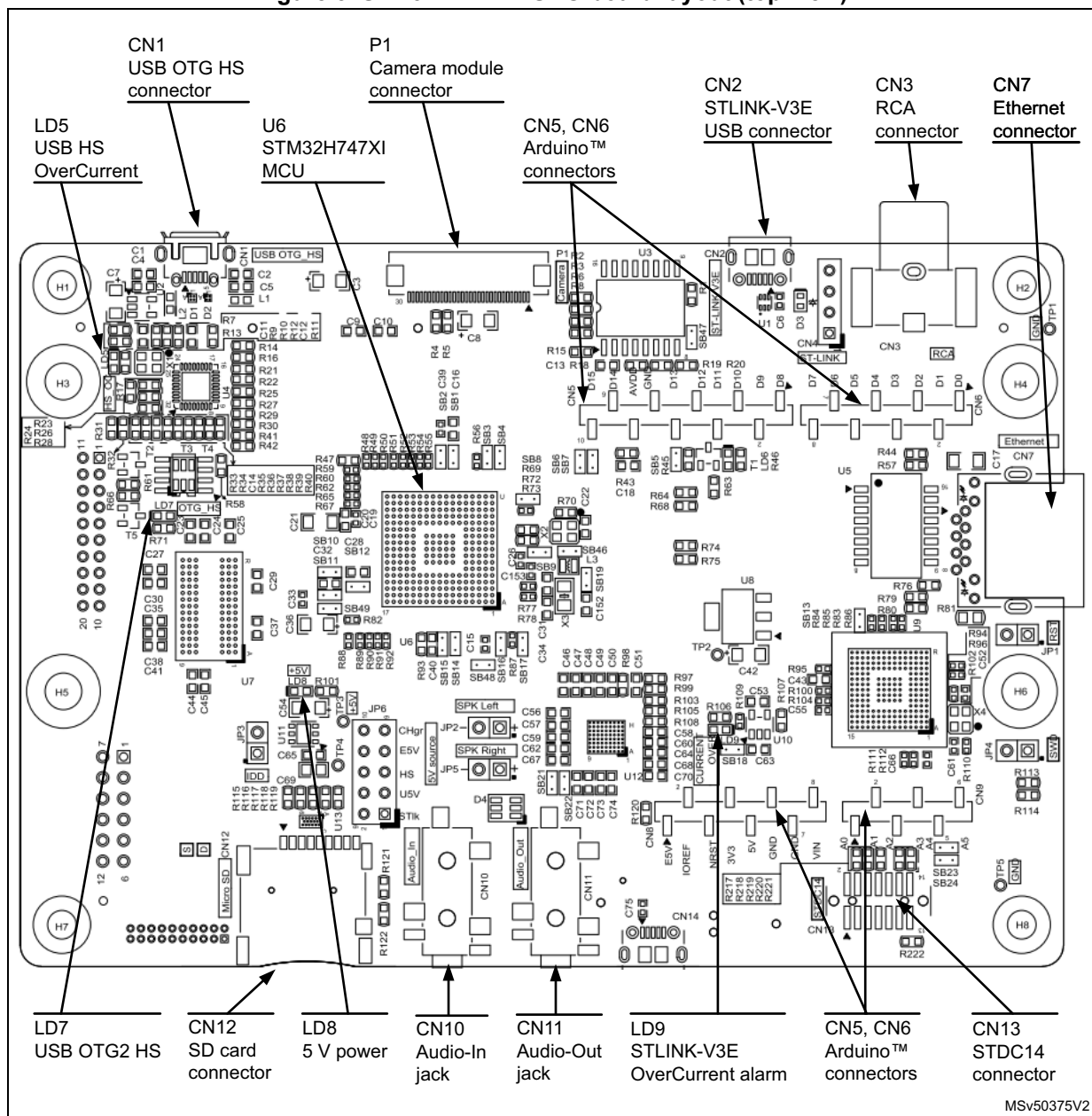
Figure 5. STM32H747I-DISCO board layout (top view)
