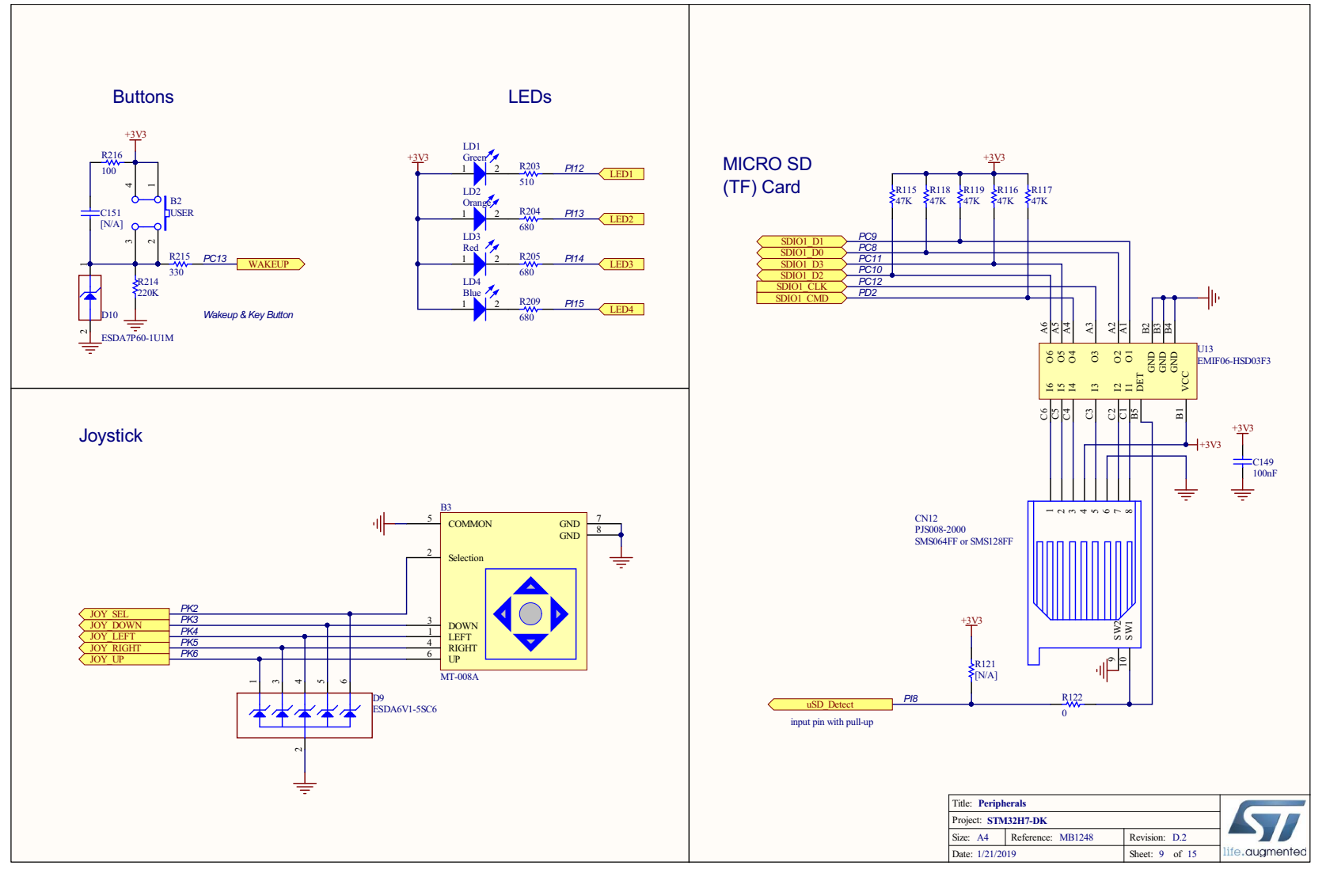
Figure 28. Physical control peripherals and microSD™ card
