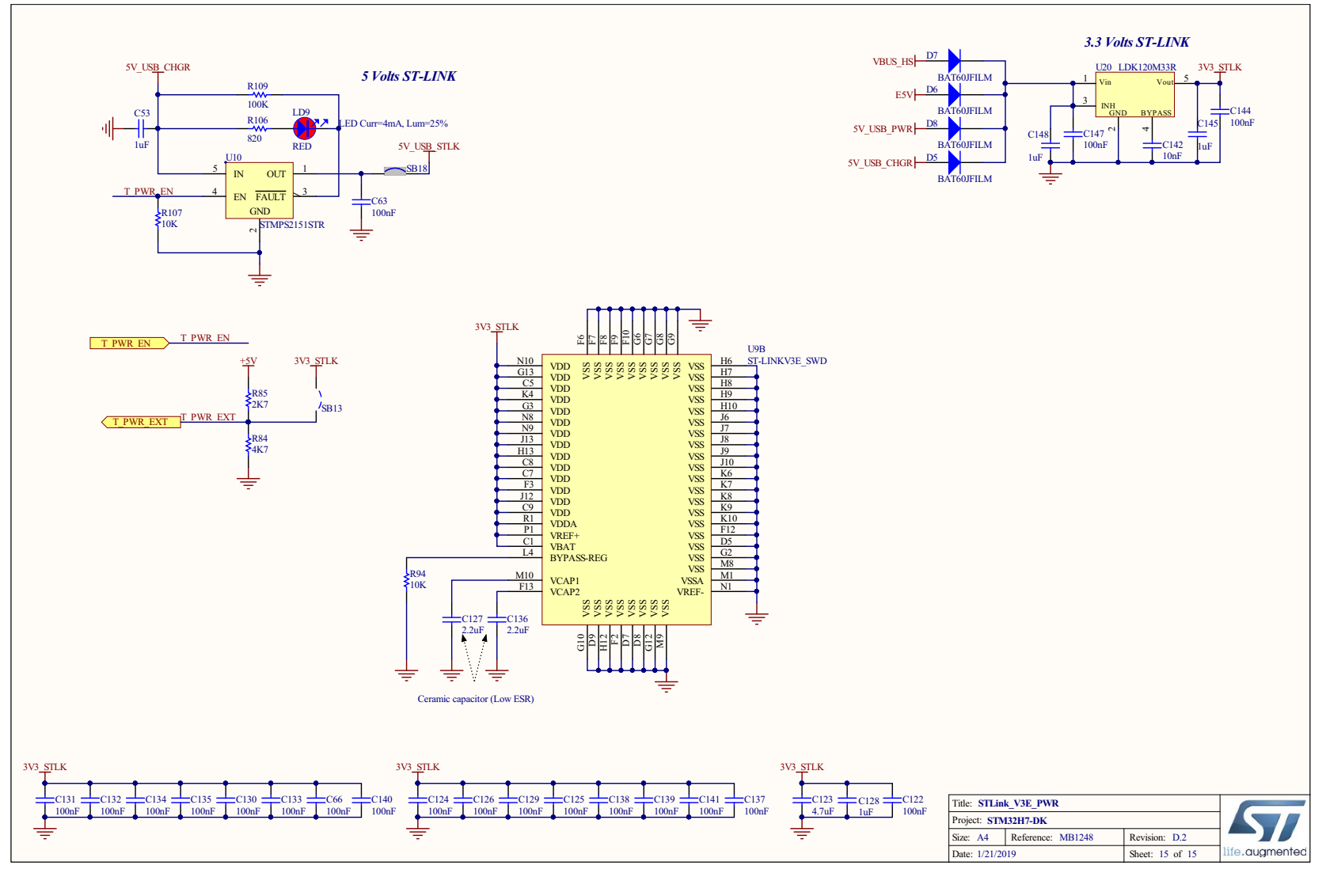
Figure 33. STLINK-V3E power
