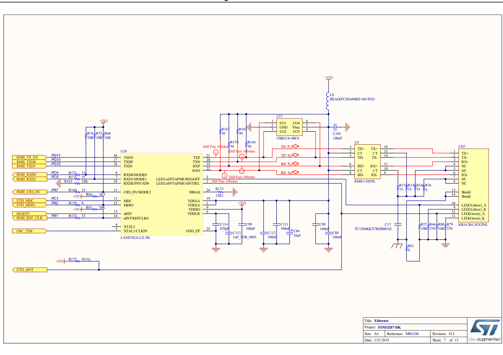
Figure 26. Ethernet
