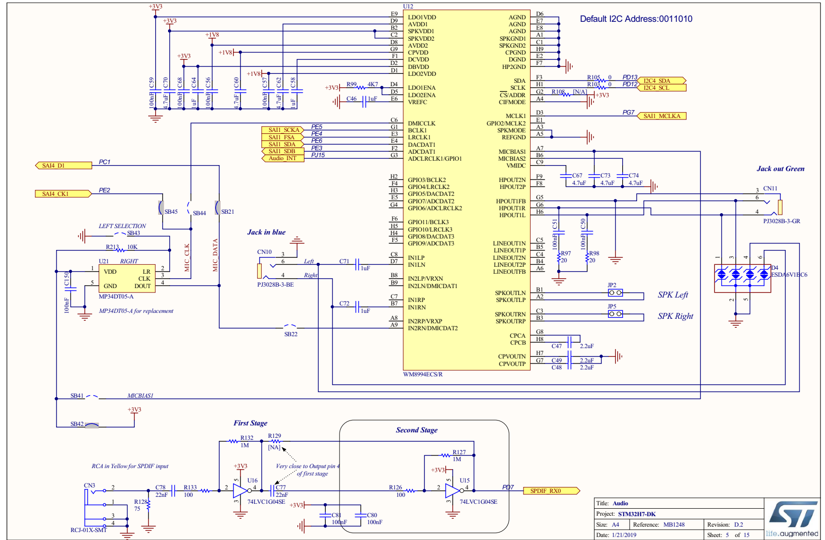
Figure 24. Audio codec device
