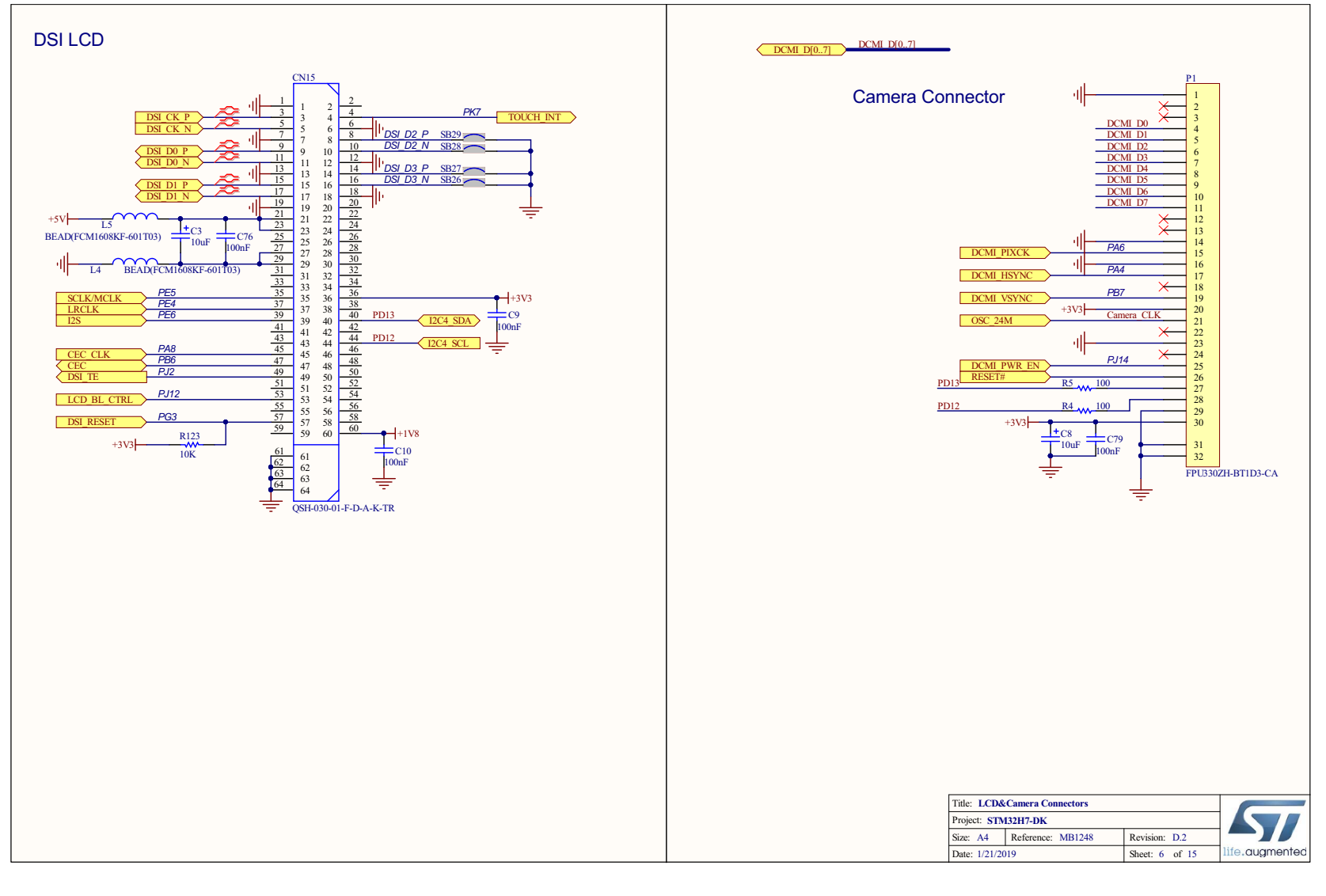
Figure 25. DSI LCD and camera connector
