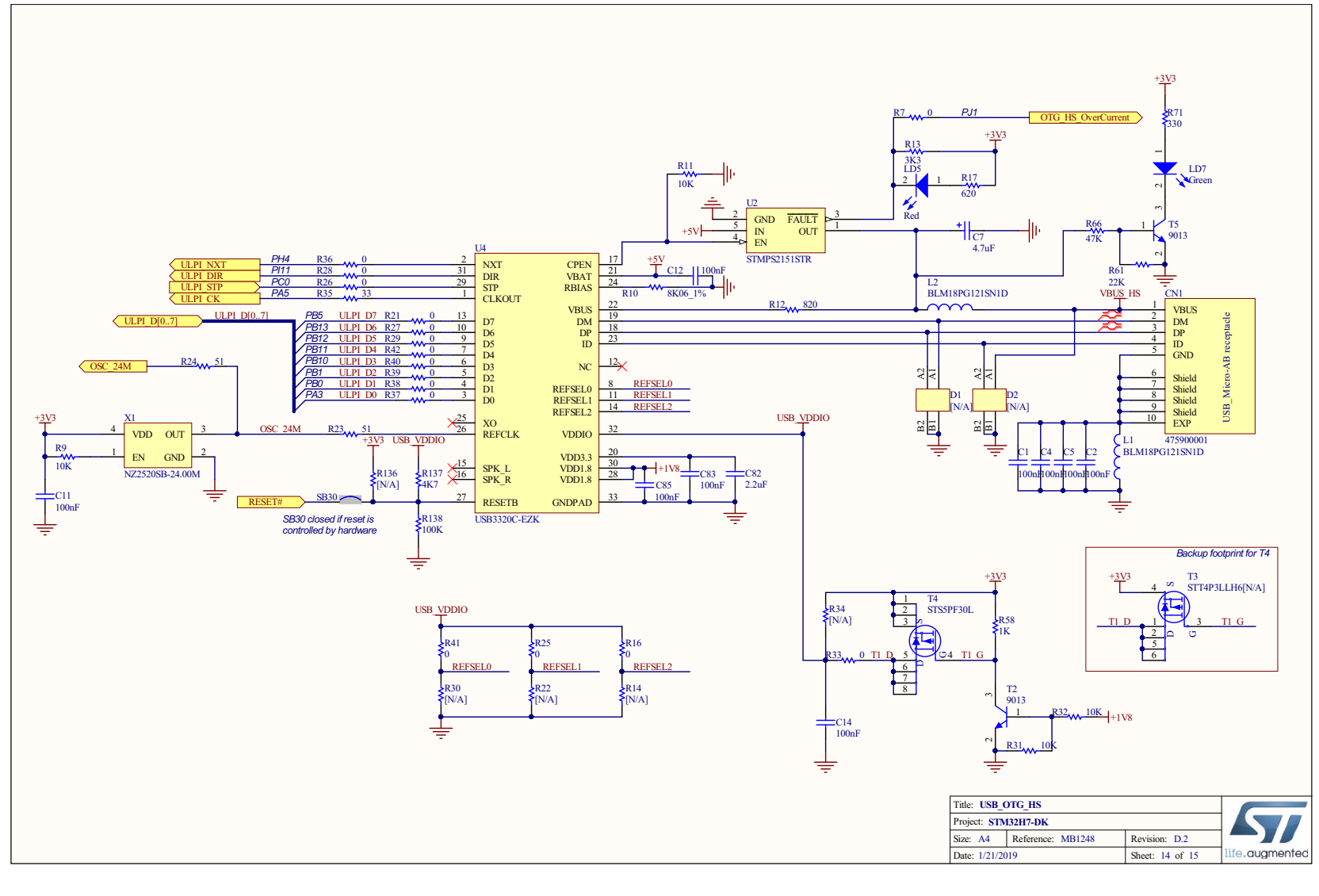
Figure 34. USB_OTG_HS port
