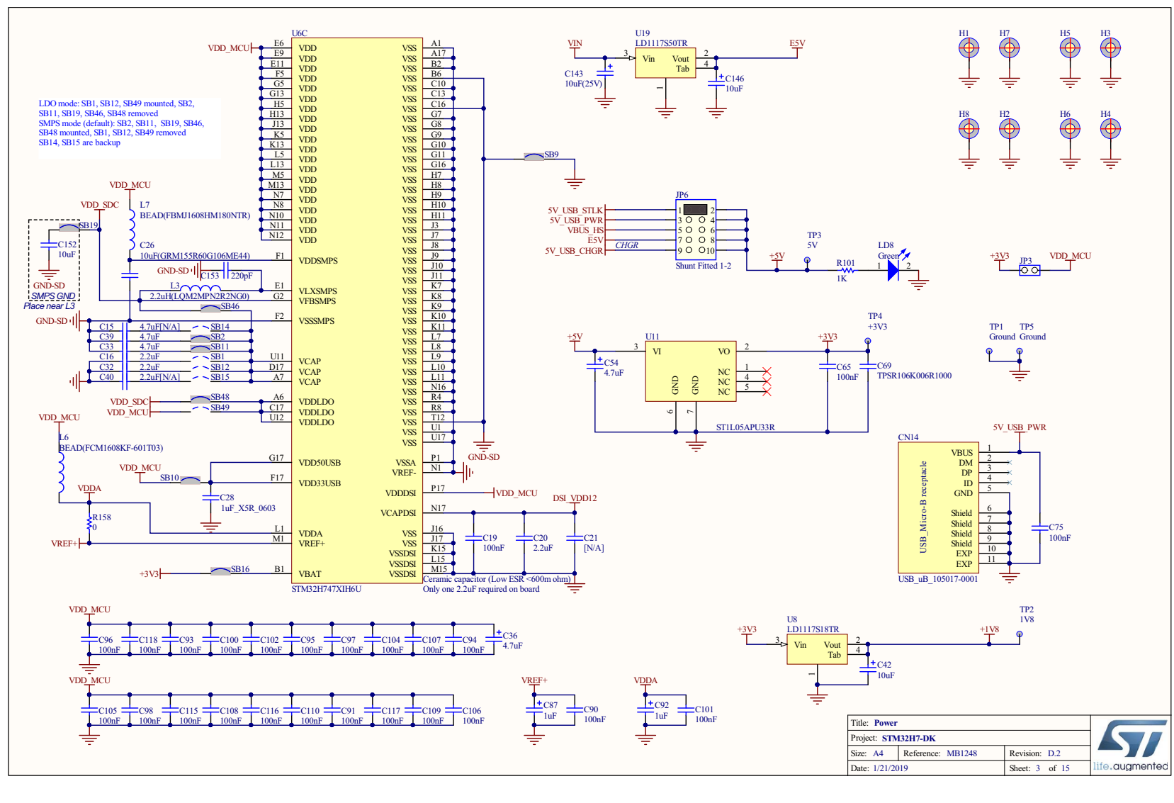
Figure 22. Power supply
