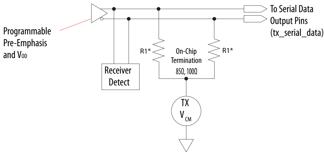
Figure 227. Transmitter Buffer
