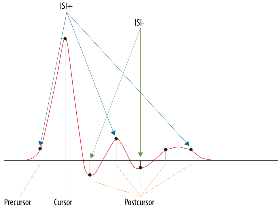
Figure 233. Signal ISI
