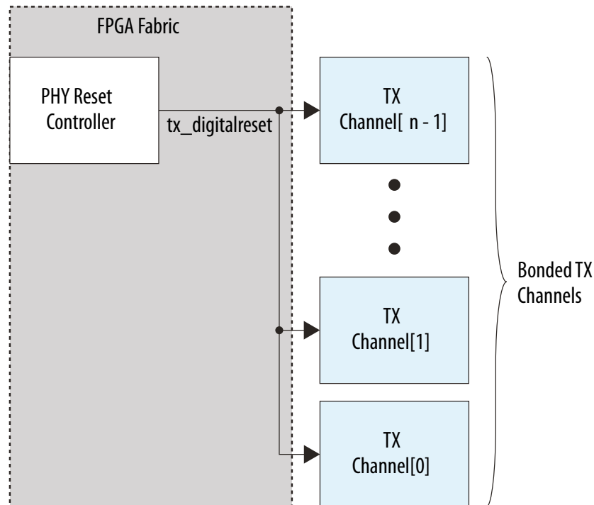
Figure 224. Physical Routing Delay Skew in Bonded Channels
