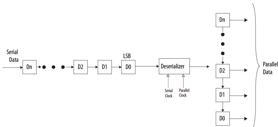
Figure 236. Deserializer Block Diagram
