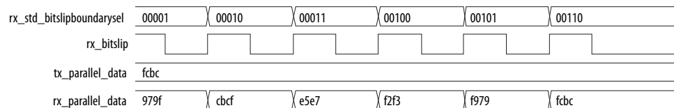
Figure 142. RX Bit Slip in 20-bit Mode
