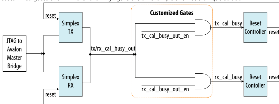
Figure 285. An Example of an AND Gate used as Customized Logic
