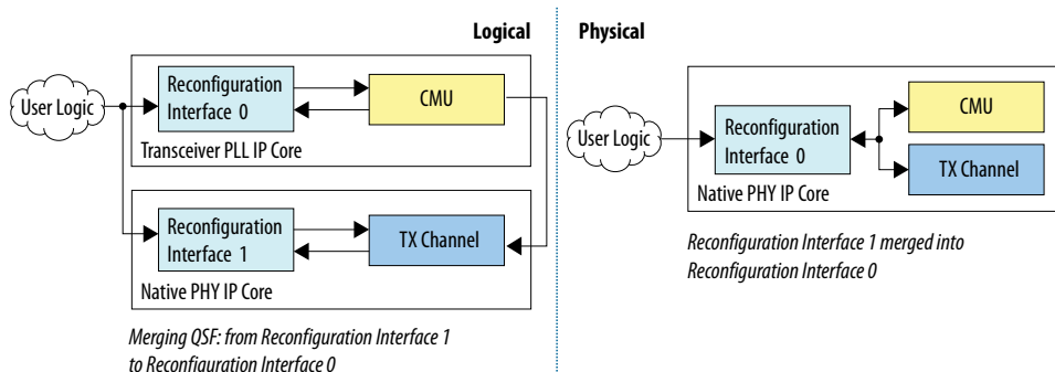
Figure 283. Separate CMU PLL and TX Channel in the Same Physical Location
