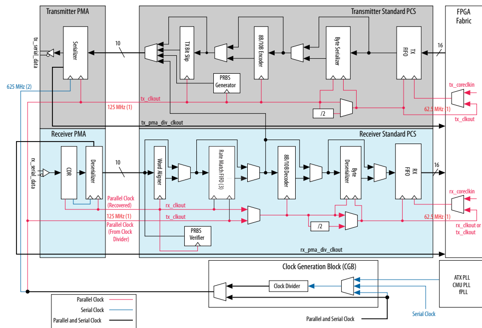
Figure 132. Transceiver Channel Datapath and Clocking for the Basic and Basic with Rate Match Configurations
