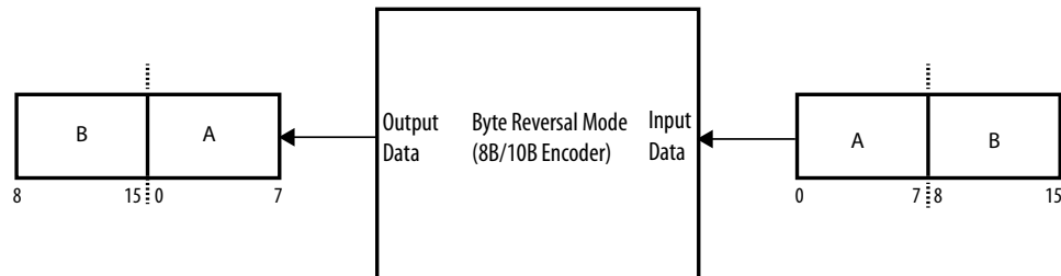
Figure 262. 8B/10B Encoder Byte Reversal Feature
