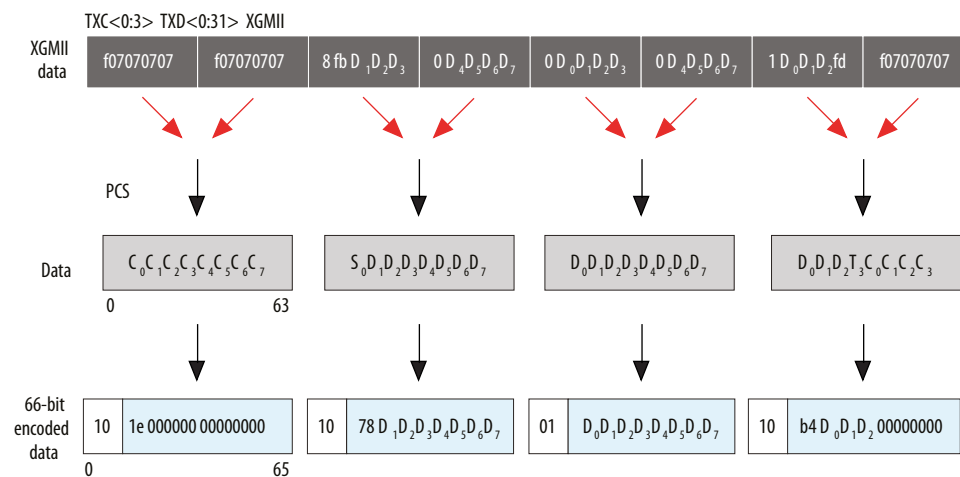
Figure 243. Example Data Pattern for 64B/66B Encoding
