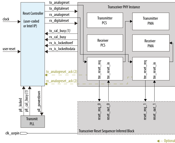
Figure 203. Typical Transceiver PHY Implementation
