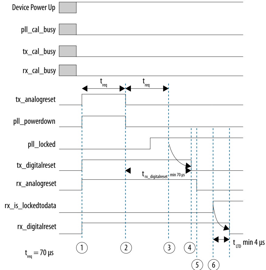
Figure 209. Resetting the Transceiver Channel During Device Operation
