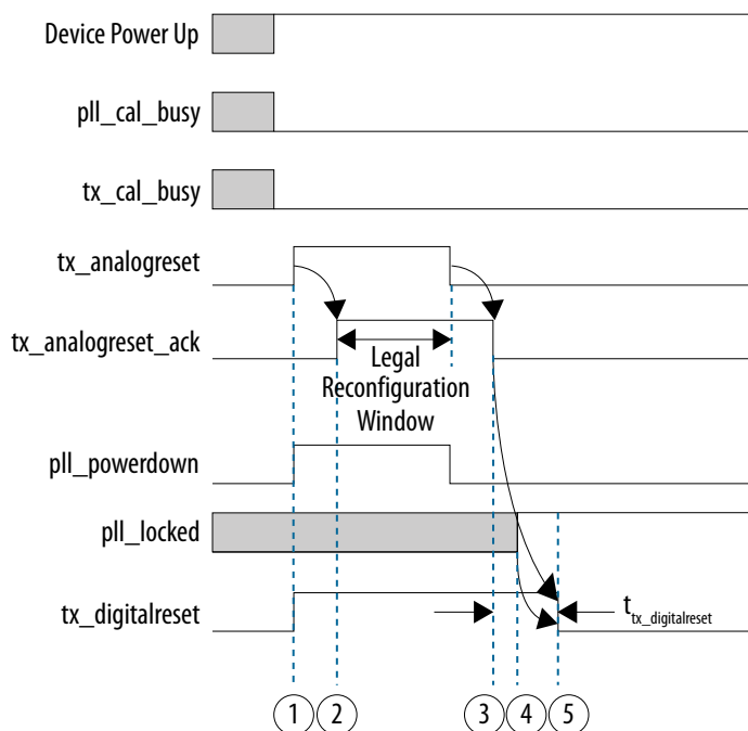
Figure 216. Dynamic Reconfiguration of Transmitter Channel During Device Operation
