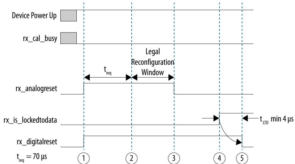
Figure 211. Dynamic Reconfiguration of Receiver Channel During Device Operation
