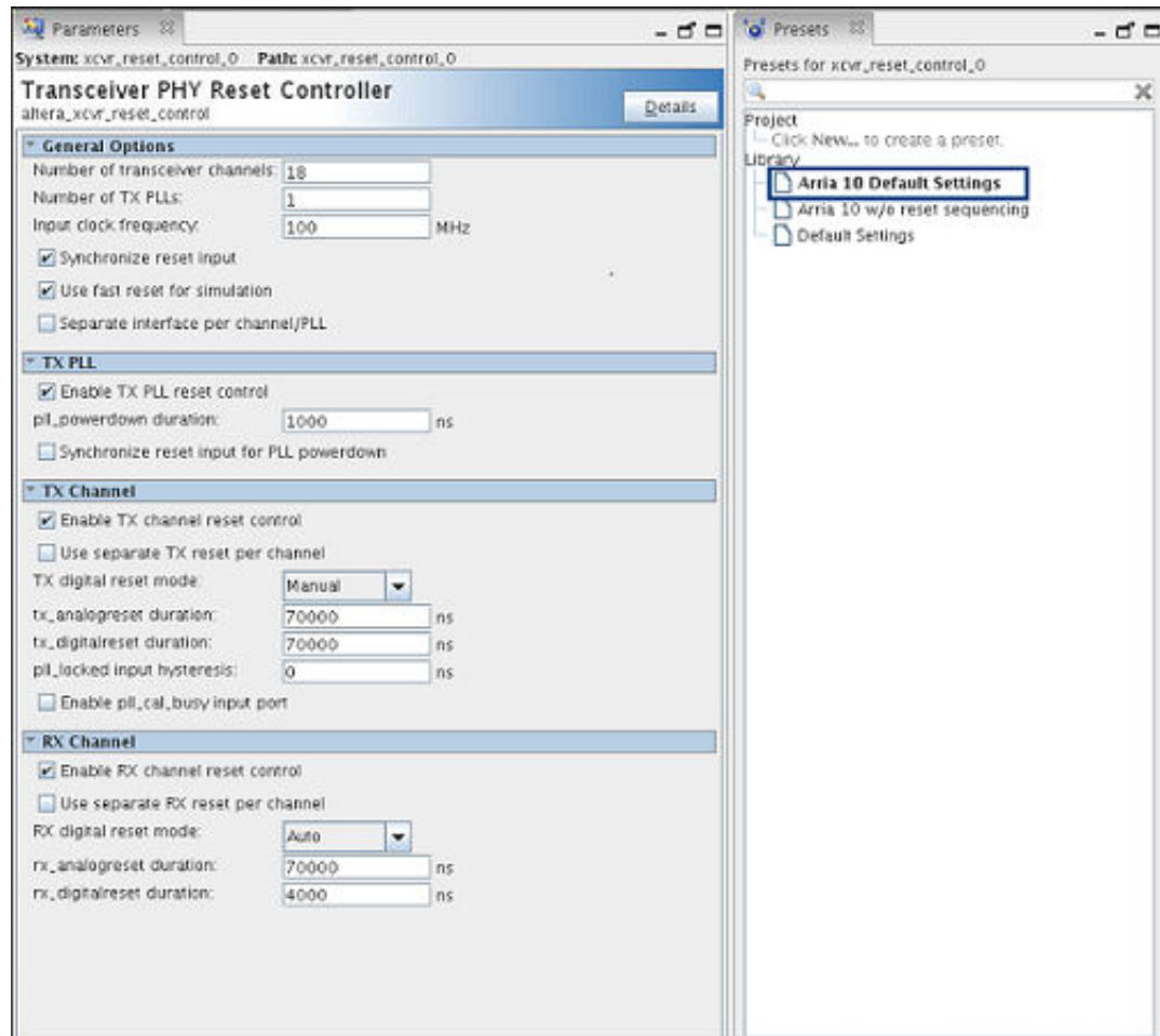
Figure 204. Arria 10 Default Settings Preset
