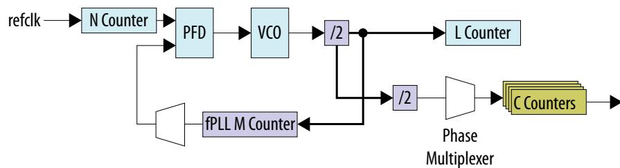
Figure 192. Integer and Phase Aligned
