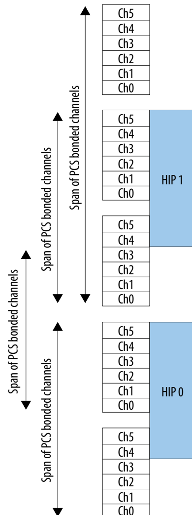
Figure 188. Hard PCS Bonding Channels Span Across Channels Adjacent to PCIe HIP and Channels Not Adjacent to PCIe HIP
