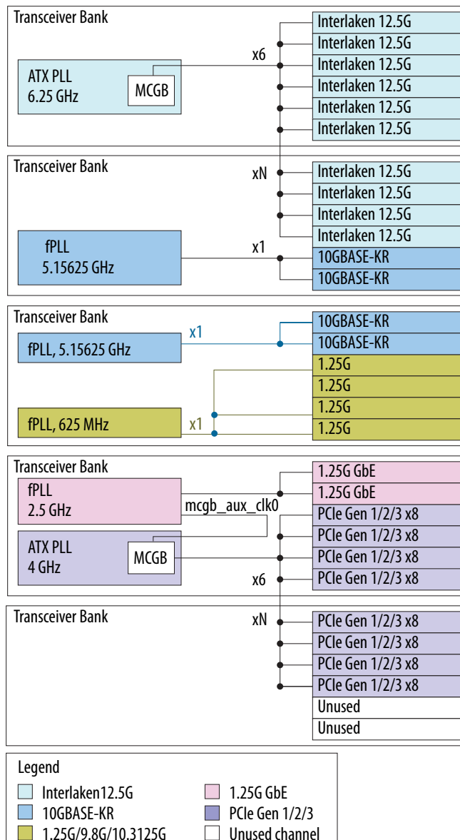
Figure 202. Mix and Match Design Example
