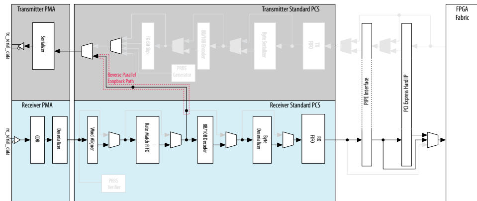
Figure 98. PCIe Reverse Parallel Loopback Mode Datapath
