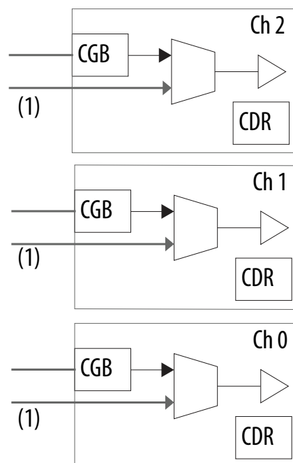
Figure 199. x6/xN Bonding Mode —Internal Channel Connections
