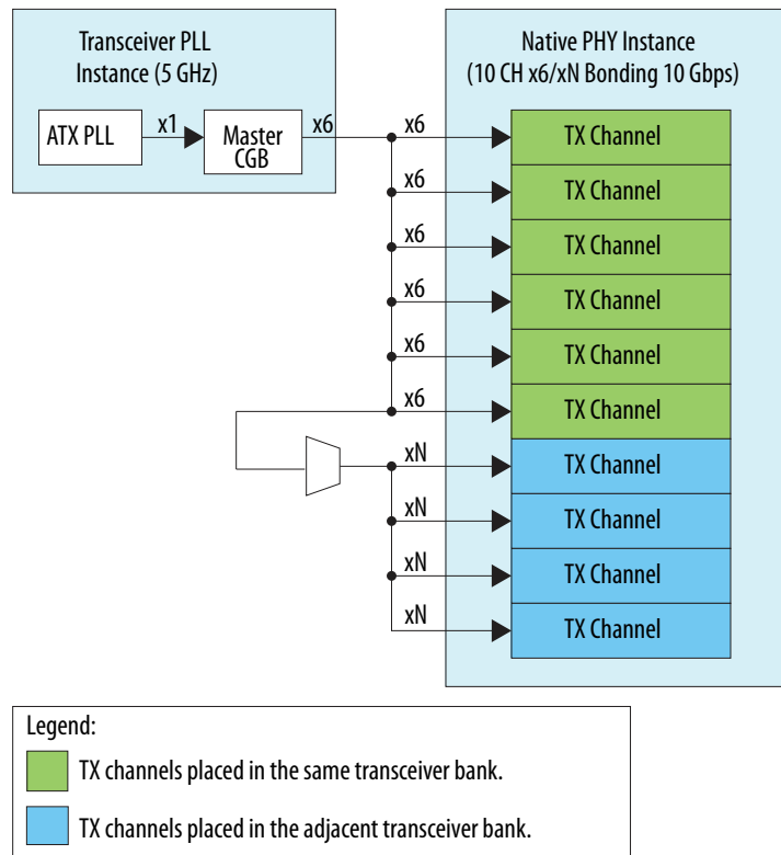
Figure 198. PHY IP Core and PLL IP Core Connection for x6/xN Bonding Mode
