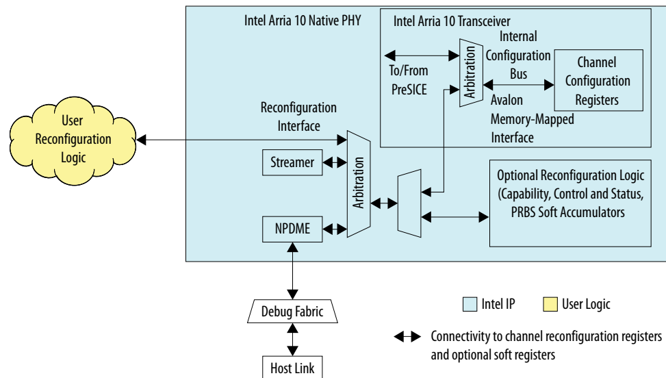
Figure 275. Arria 10 Native PHY with Embedded Streamer
