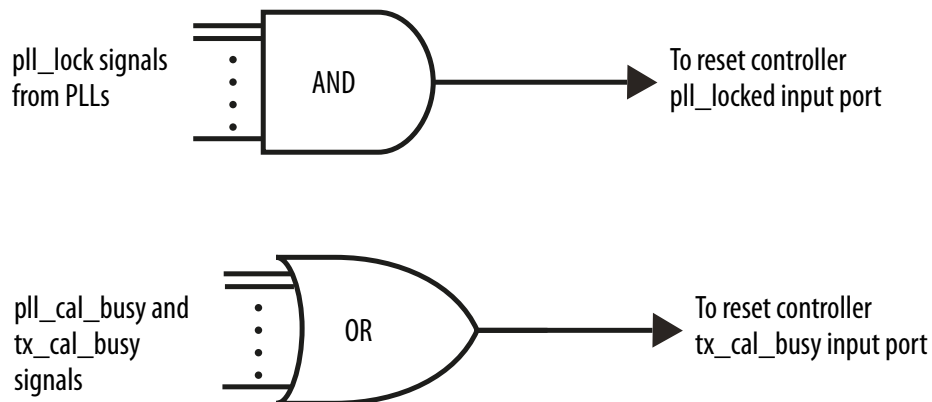
Figure 223. Multiple PLL Configuration
