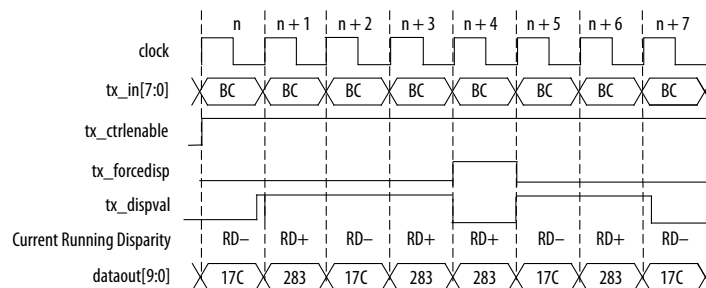
Figure 154. 8B/10B TX Disparity Control
