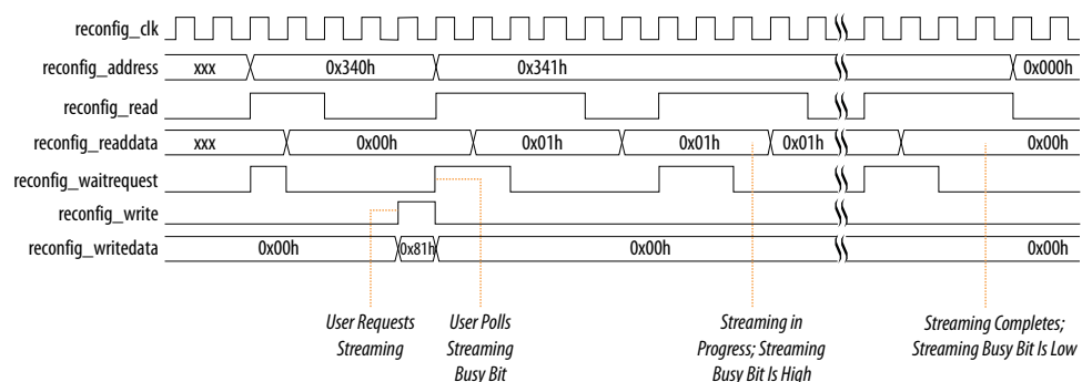
Figure 276. Timing Diagram for Embedded Streamer Reconfiguration
