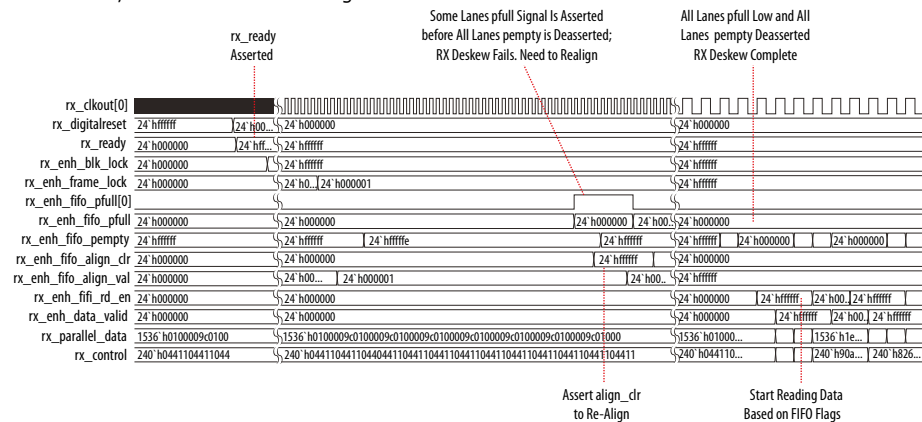
Figure 41. 24 Lanes Bonded Interlaken Link, RX Direction
