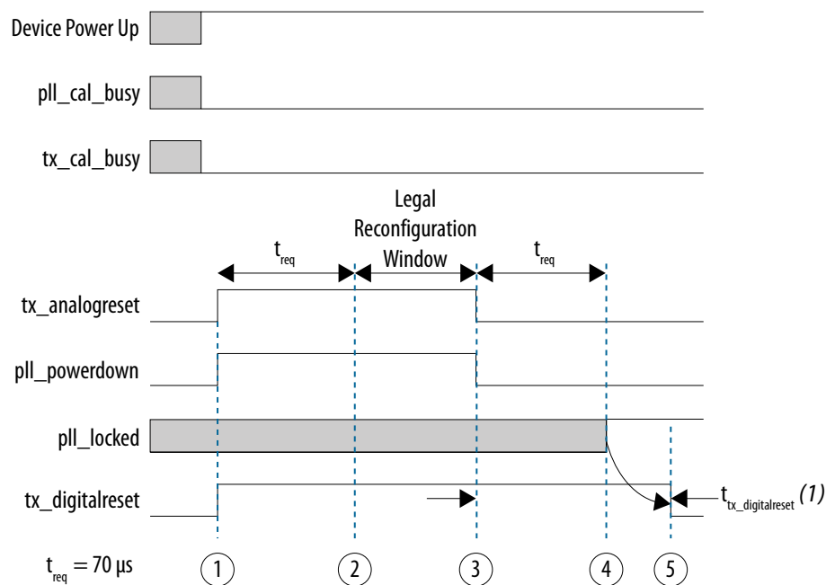
Figure 210. Dynamic Reconfiguration of Transmitter Channel During Device Operation
