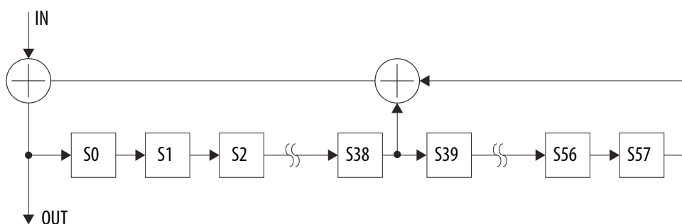
Figure 245. Asynchronous Scrambler in Serial Implementation
