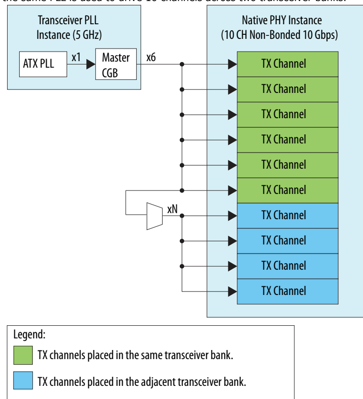
Figure 196. PHY IP Core and PLL IP Core Connection for Multi-Channel xN Non-Bonded Configuration
