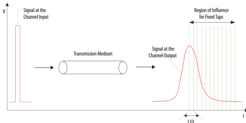
Figure 234. Channel Pulse Response
