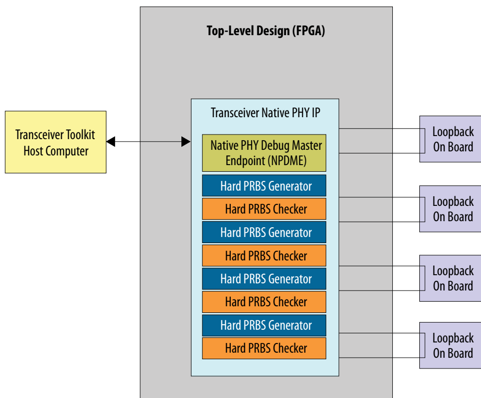
Figure 301. Four Channels Loopback Mode for Intel Arria 10 GX Devices
