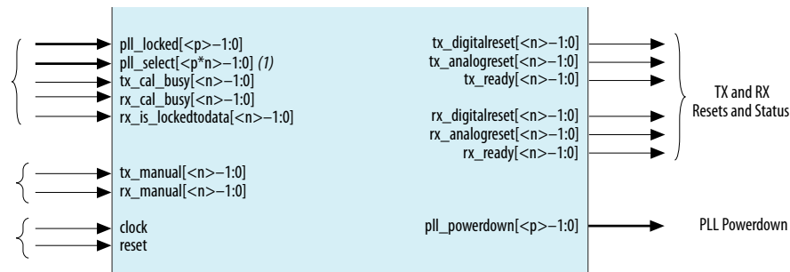
Figure 220. Transceiver PHY Reset Controller IP Core Top-Level Signals
