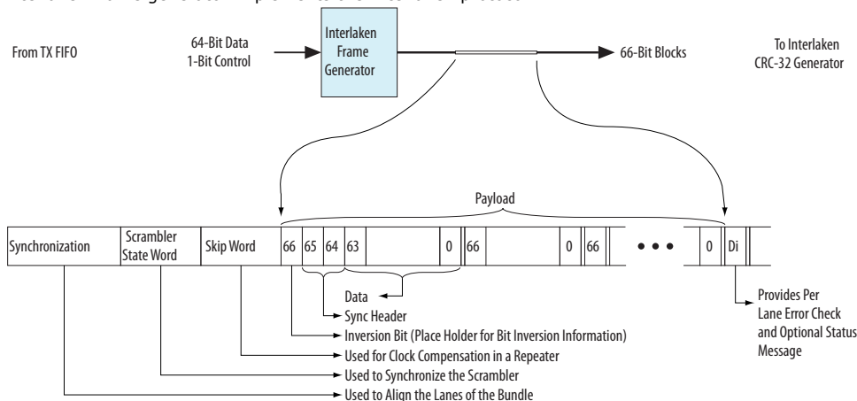
Figure 241. Interlaken Frame Generator
