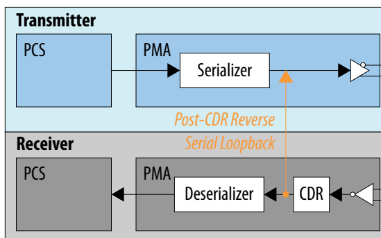
Figure 279. Reverse Serial Loopback Mode (Post-CDR)
