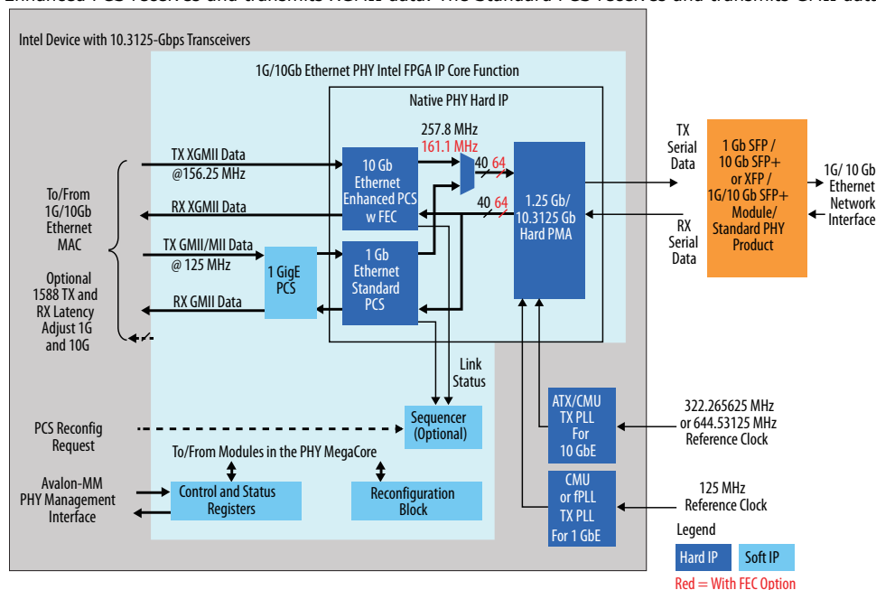
Figure 72. Top Level Modules of the 1G/10GbE PHY IP Function
