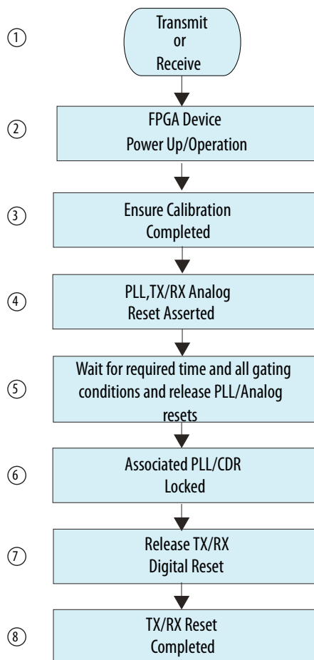
Figure 205. Transmitter and Receiver Reset Sequence
