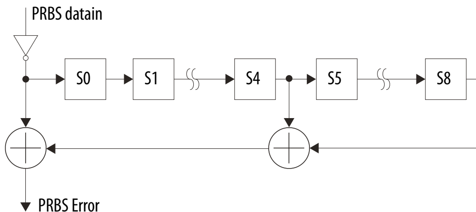
Figure 250. PRBS9 Verify Serial Implementation
