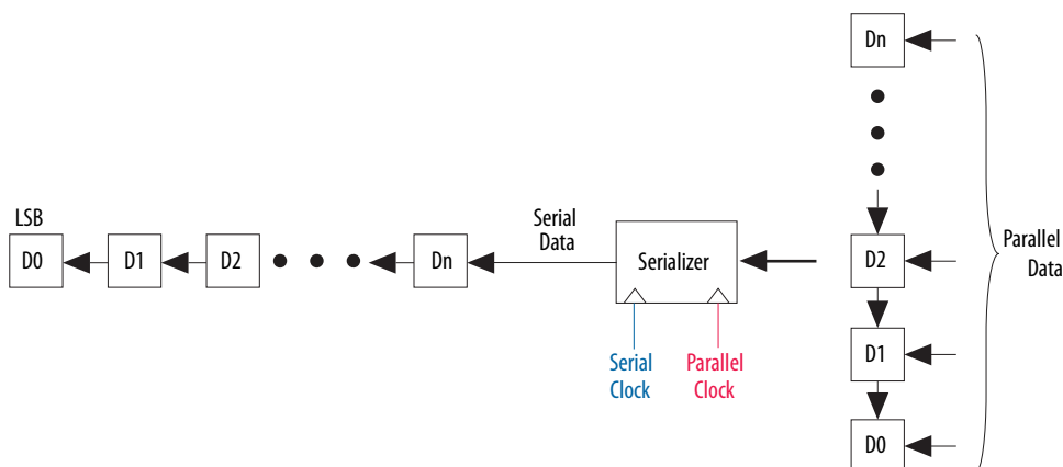
Figure 226. Serializer Block
