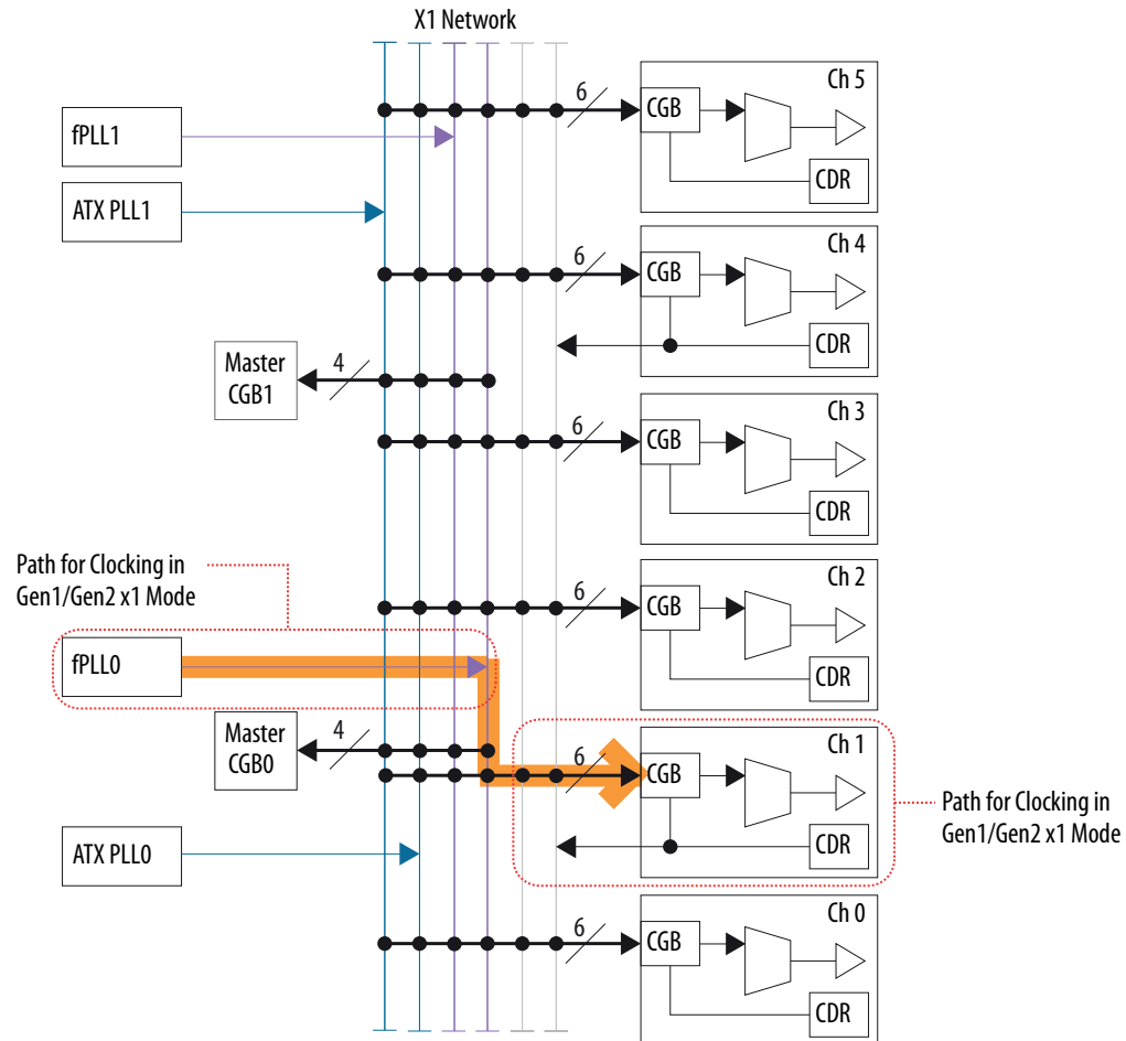
Figure 103. Use ATX PLL or fPLL for Gen1/Gen2 x1 Mode
