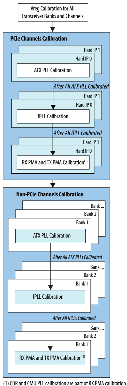
Figure 287. Power-up Calibration Sequence for PCIe Hard IP and non-PCIE Channels
