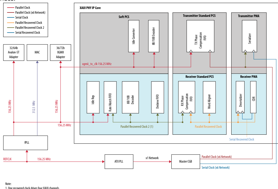
Figure 88. Transceiver Clocking for XAUI Configuration With Phase Compensation FIFO Enabled
