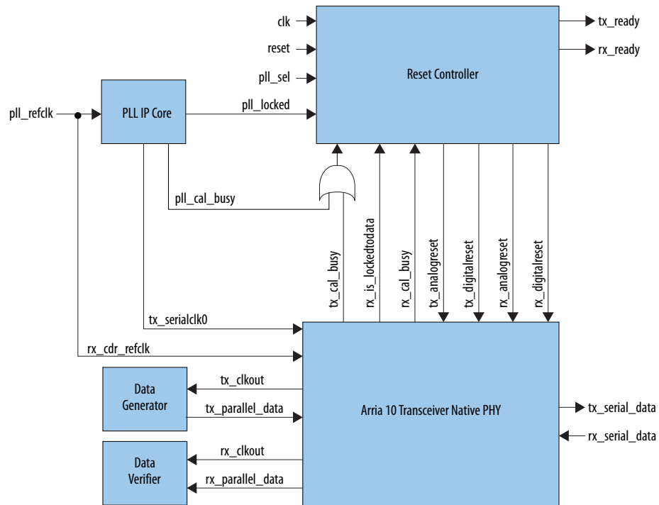
Figure 122. Connection Guidelines for a CPRI PHY Design
