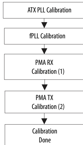
Figure 288. Recalibration Sequence when the Transceiver Reference Clock or Data Rate Changes
