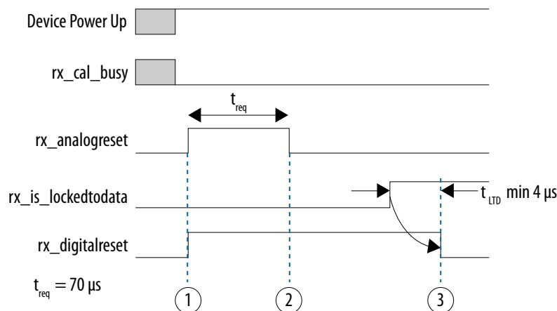
Figure 207. Resetting the Receiver During Device Operation (Auto Mode)
