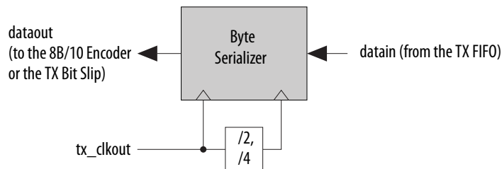
Figure 258. Byte Serializer Block Diagram
