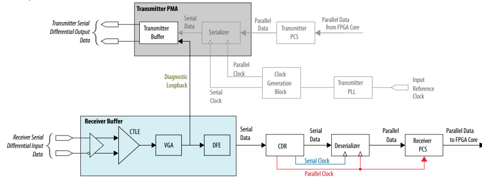
Figure 239. Reverse Serial Loopback Path/Post CDR
