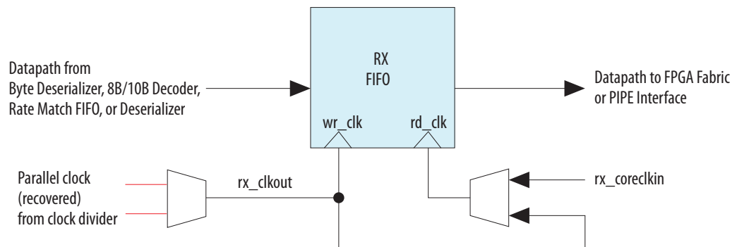
Figure 267. RX FIFO Block Diagram
