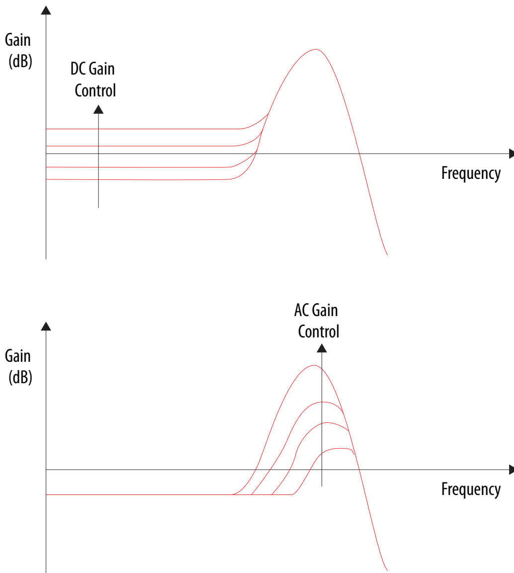
Figure 231. CTLE DC and AC Gain Conceptualization
