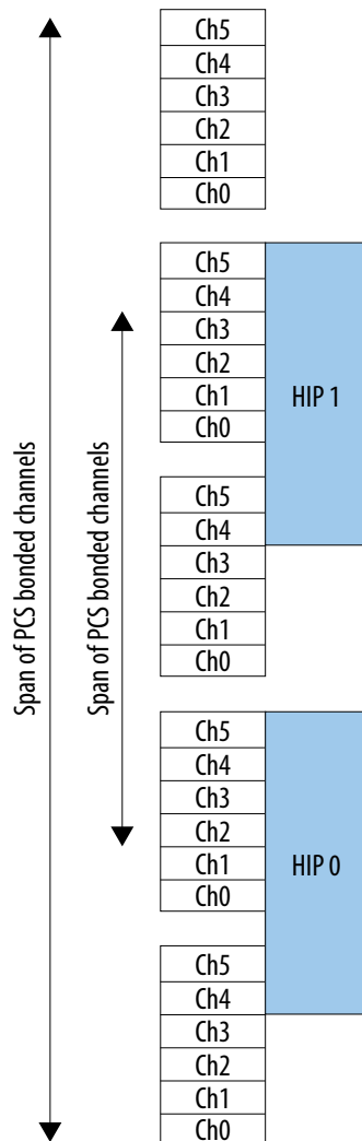
Figure 189. Hard PCS Bonding Channels are Not Allowed to Span Across Two HIPs
