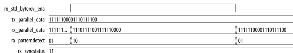
Figure 145. RX Byte Reversal
