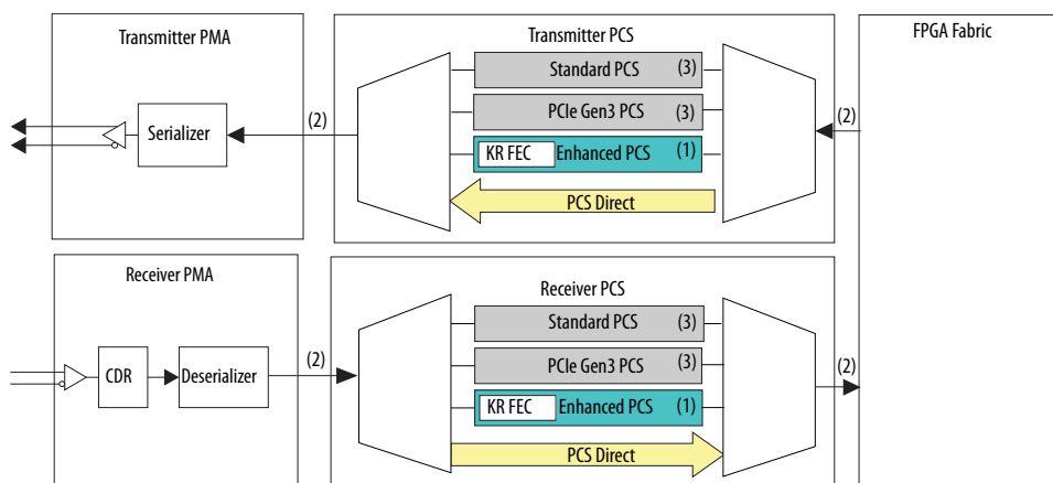
Figure 17. GT Transceiver Channel in Full Duplex Mode Operating Between 17.4 Gbps and 25.8 Gbps
