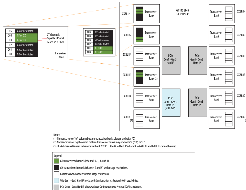
Figure 8. Intel Arria 10 GT Device with 72 Transceiver Channels and Four PCIe Hard IP Blocks
