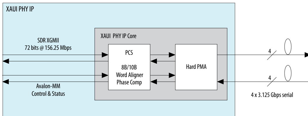
Figure 84. XAUI PHY IP Core
