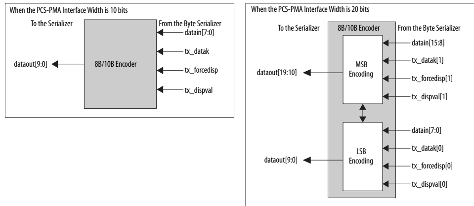
Figure 259. 8B/10B Encoder Block Diagrams
