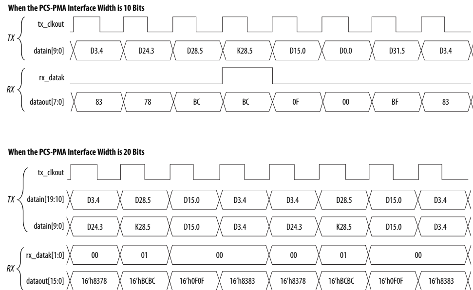
Figure 265. 8B/10B Decoder in Control Code Group Detection
