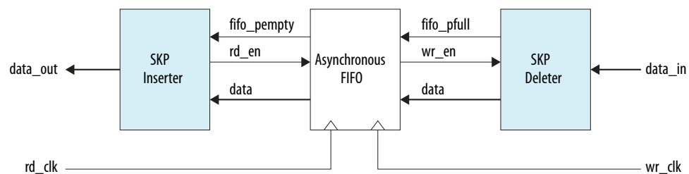
Figure 269. Rate Match FIFO
