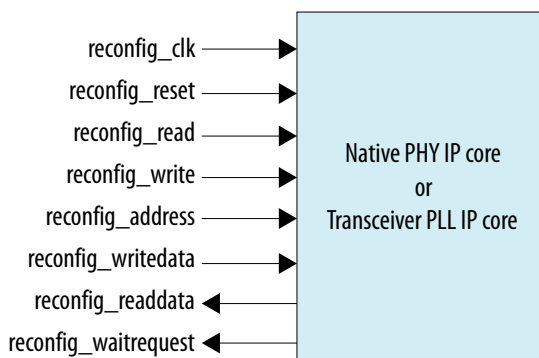
Figure 271. Top-Level Signals of the Reconfiguration Interface
