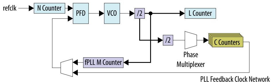
Figure 192. Integer and Phase Aligned
