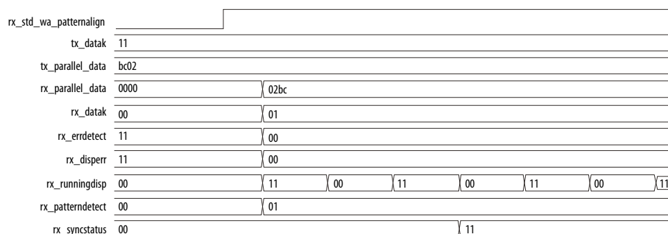
Figure 138. Synchronization State Machine Mode when the PCS-PMA Interface Width is 20 Bits
