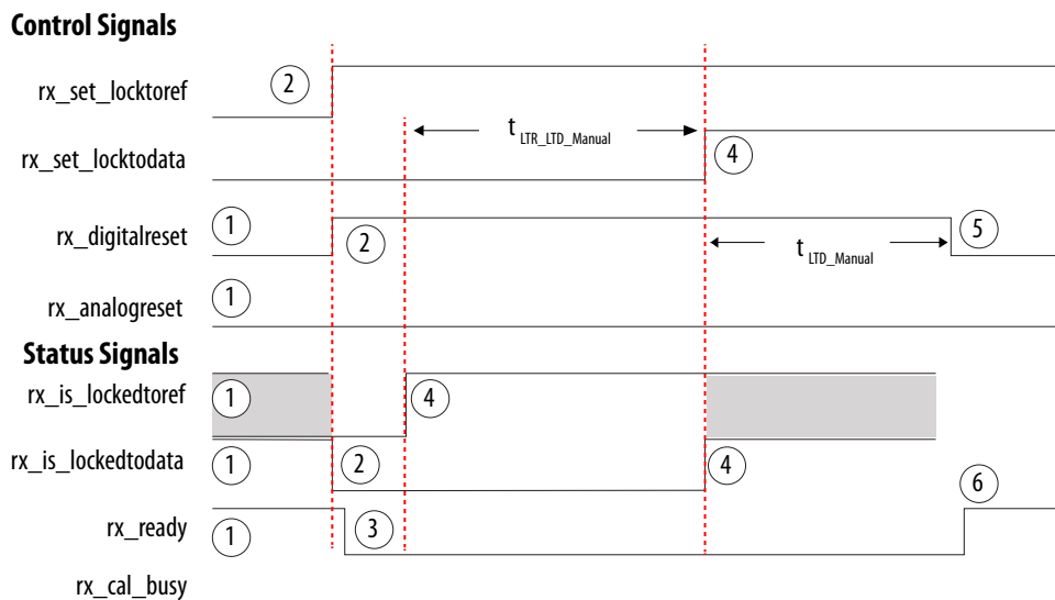
Figure 218. Reset Sequence Timing Diagram for Receiver when CDR is in Manual Lock Mode
