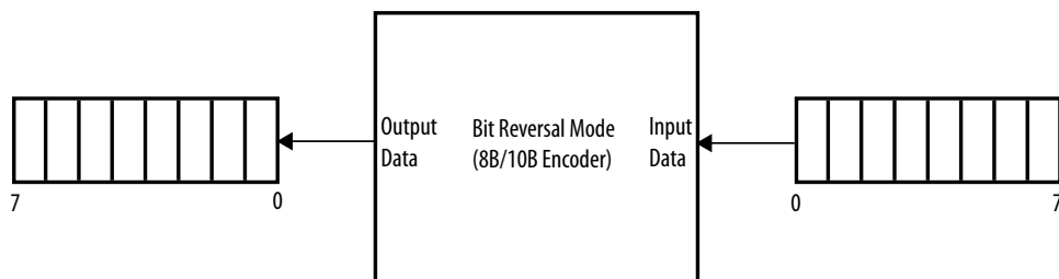
Figure 261. 8B/10B Encoder Bit Reversal Feature
