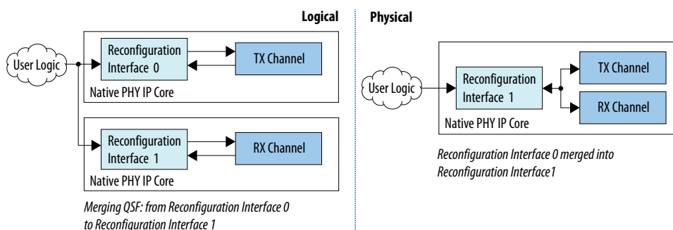
Figure 282. Independent Instances of Simplex TX/RX in the Same Physical Location
