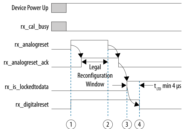
Figure 217. Dynamic Reconfiguration of Receiver Channel During Device Operation
