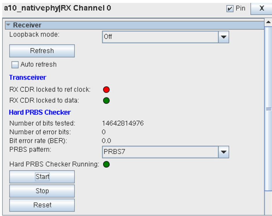
Figure 296. RX CDR Locked to Data
