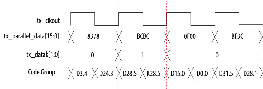
Figure 260. Control Code Encoding Diagram
