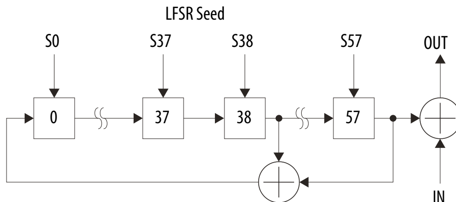
Figure 246. Synchronous Scrambler Showing Different Programmable Seeds
