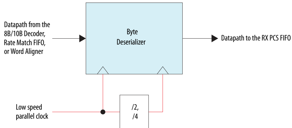
Figure 266. Byte Deserializer Block Diagram
