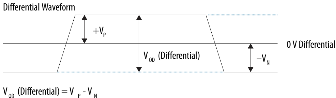
Figure 228. V OD (Differential) Signal Level
