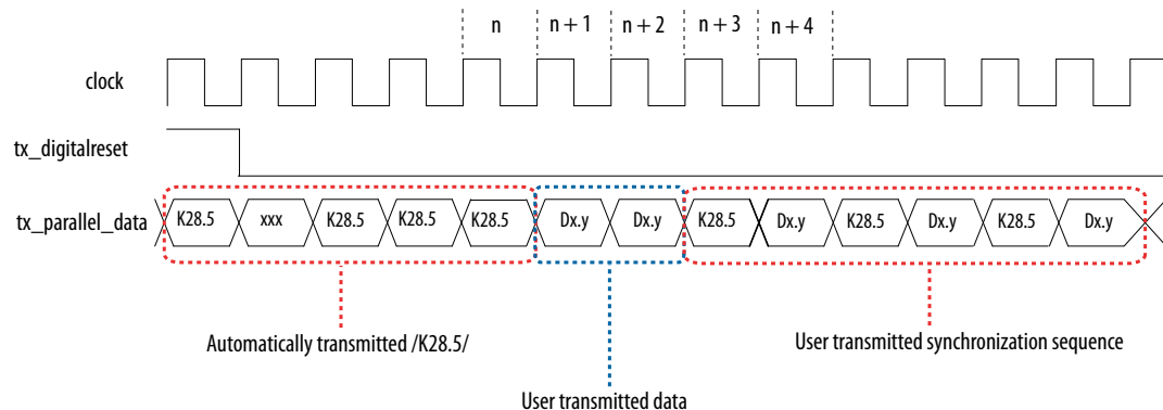
Figure 45. Reset Condition
