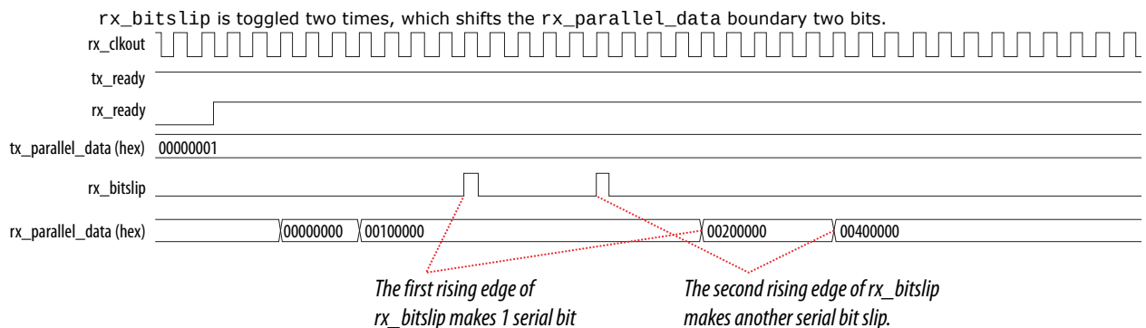
Figure 249. RX Bitflip
