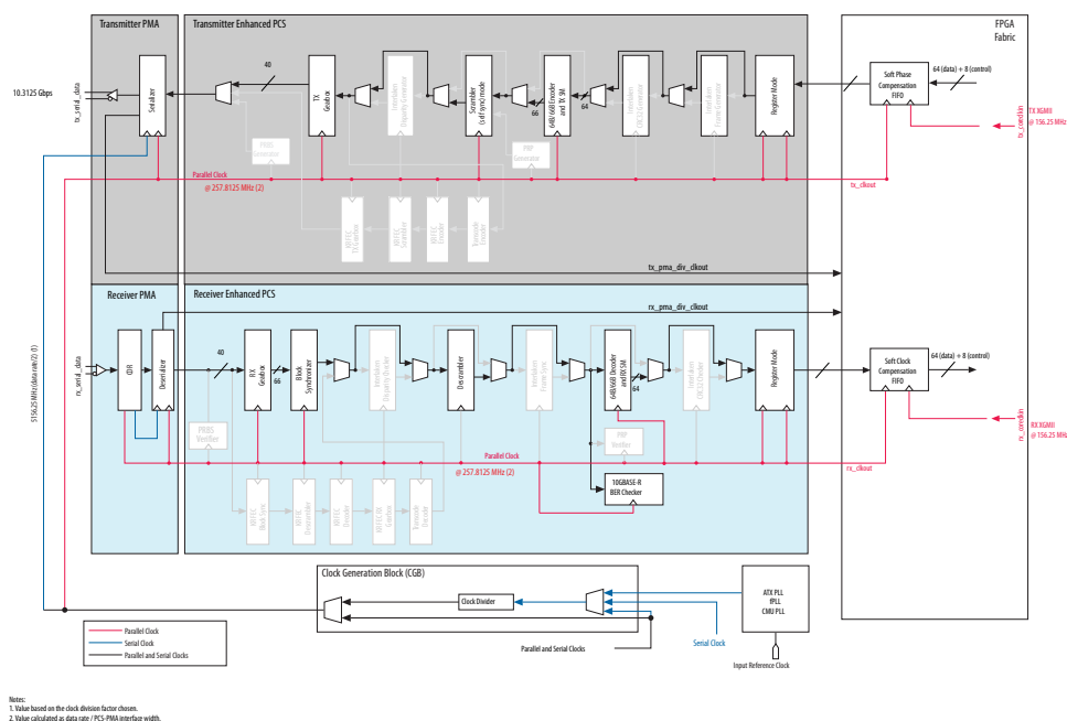
Figure 56. Transceiver Channel Datapath and Clocking for 10GBASE-R with IEEE 1588v2
