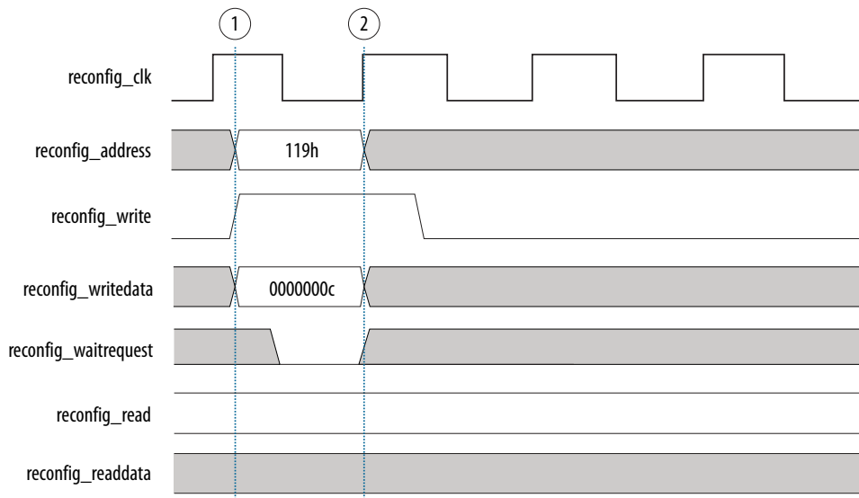
Figure 273. Writing to the Reconfiguration Interface
