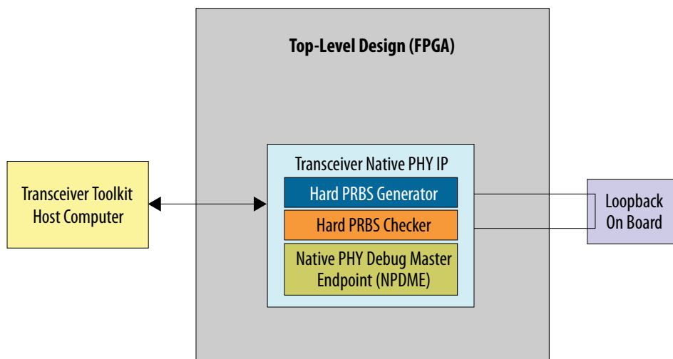
Figure 300. One Channel Loopback Mode for Intel Arria 10 GX Devices
