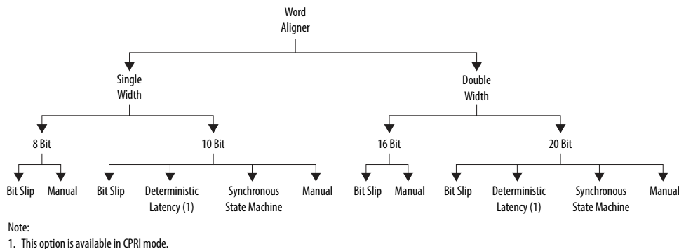
Figure 263. Word Aligner Conditions and Modes
