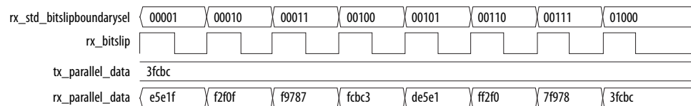
Figure 142. RX Bit Slip in 20-bit Mode
