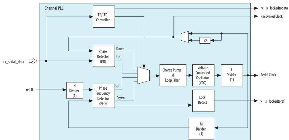
Figure 235. Channel PLL Configured as CDR
