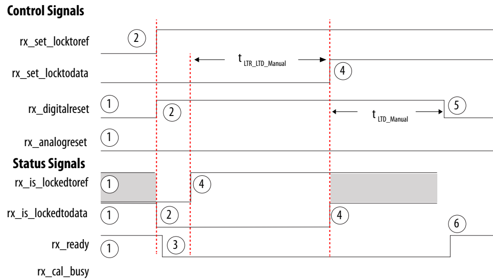
Figure 208. Reset Sequence Timing Diagram for Receiver when CDR is in Manual Lock Mode
