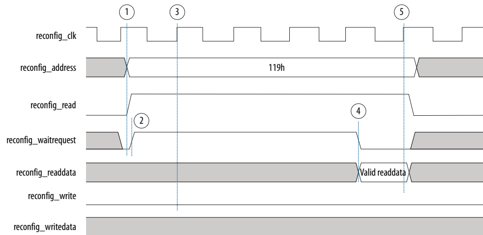
Figure 272. Reading from the Reconfiguration Interface
