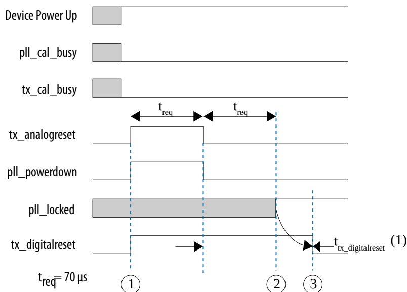
Figure 206. Transmitter Reset Sequence During Device Operation
