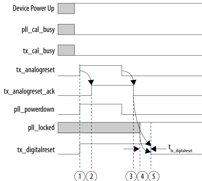
Figure 214. Transmitter Reset Sequence During Device Operation
