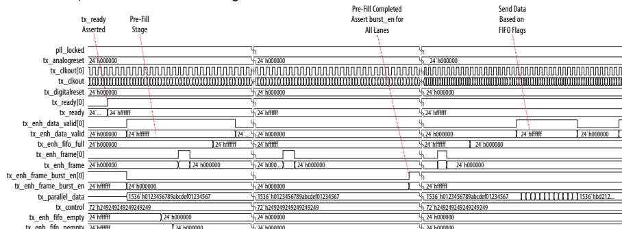
Figure 40. 24 Lanes Bonded Interlaken Link, TX Direction
