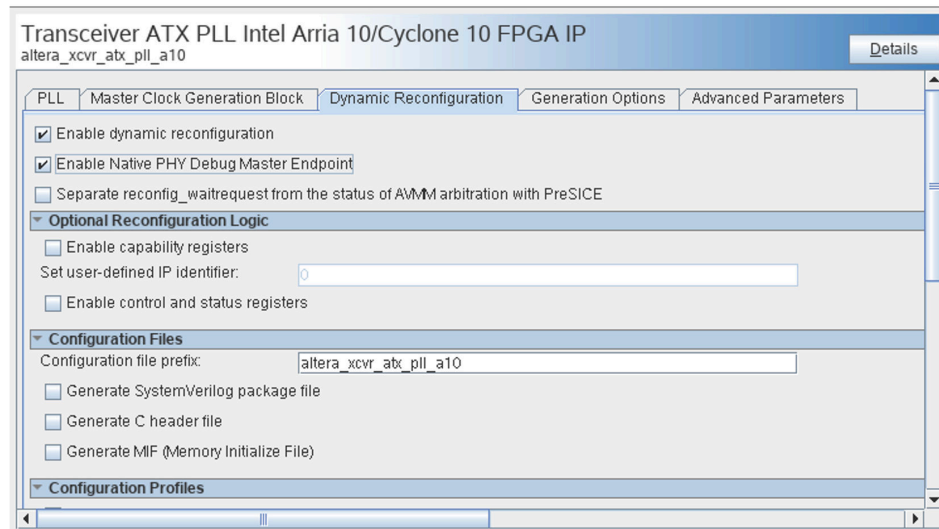
Figure 292. Dynamic Reconfiguration Parameters in Intel Arria 10 GX Transceiver ATX PLL IP Core
