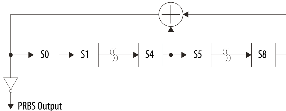
Figure 244. PRBS Generator for Serial Implementation of PRBS9 Pattern
