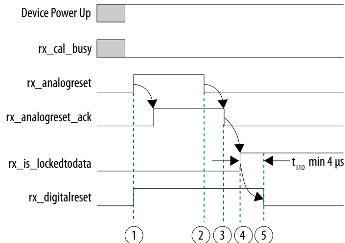
Figure 215. Receiver Reset Sequence During Device Operation
