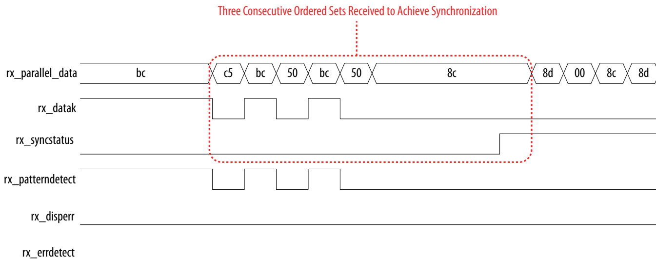
Figure 46. rx_syncstatus High
