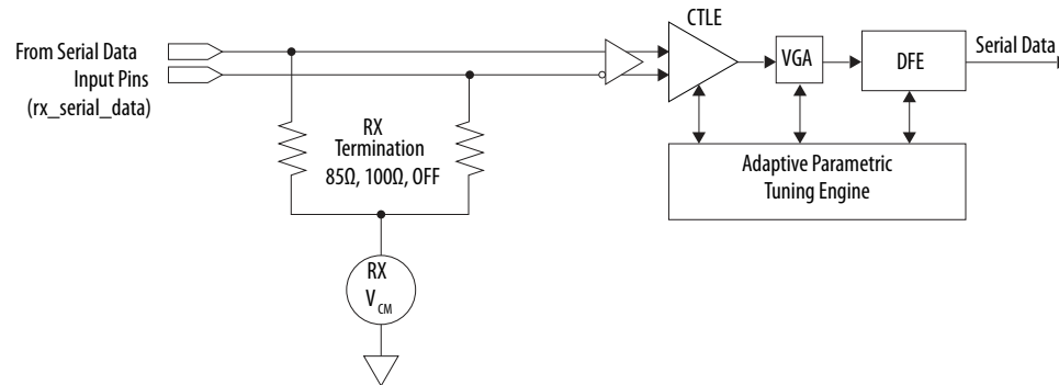
Figure 230. Receiver Buffer
