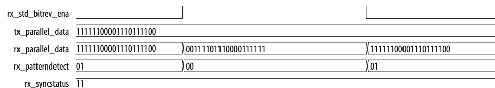
Figure 144. RX Bit Reversal
