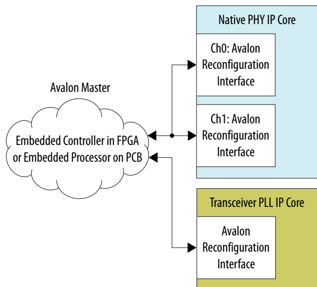
Figure 270. Reconfiguration Interface in Arria 10 Transceiver IP Cores
