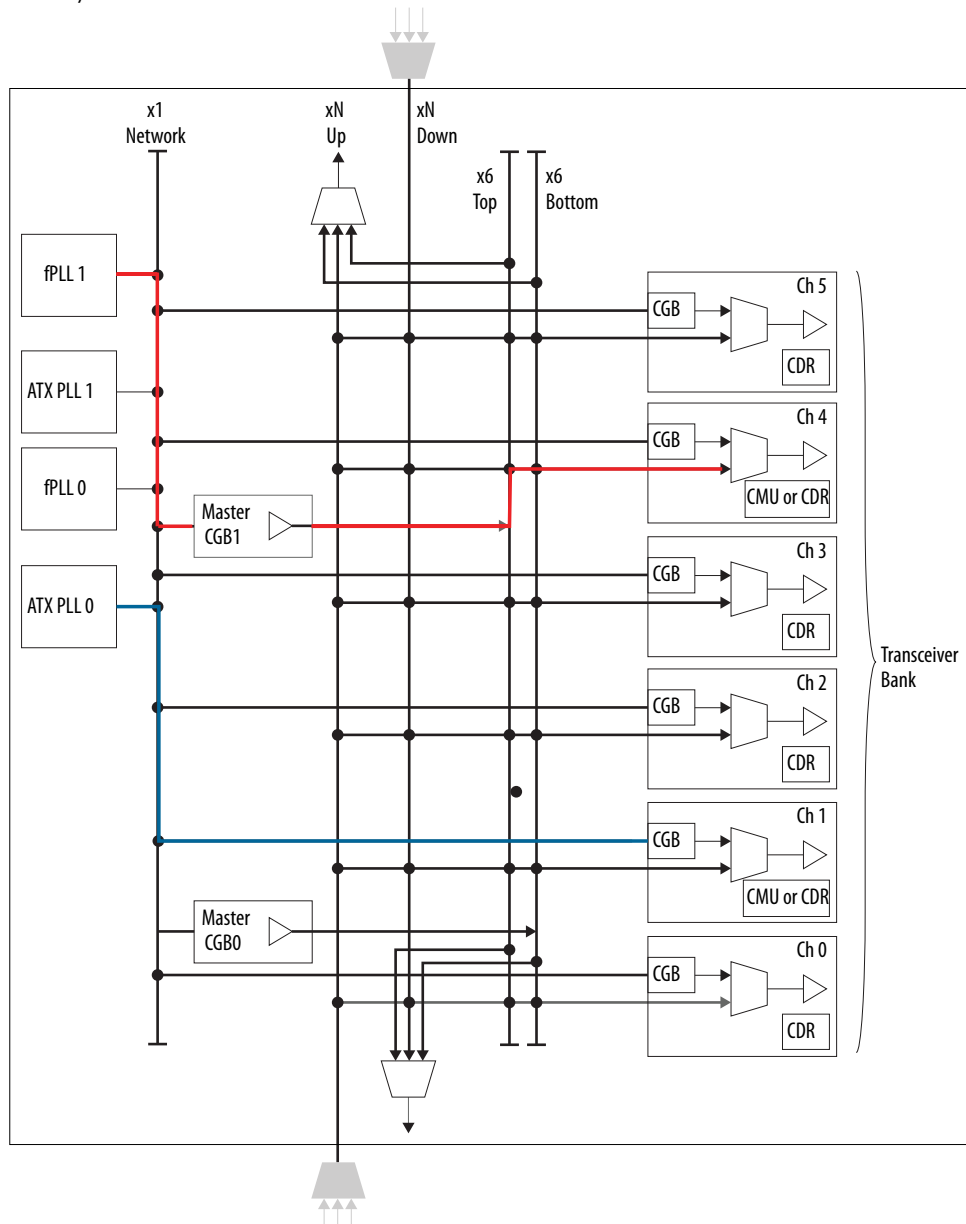
The local clock for each transceiver channel can be sourced from either the local CGB via the x1 network, or the master CGB via the x6/xN network. For example, as shown by the red highlighted path, the fPLL 1 drives the x1 network which in turn drives the master CGB. The master CGB then drives the x6 clock network which routes the clocks to the local channels. As shown by the blue highlighted path, the ATX PLL 0 can also drive the x1 clock network which can directly feed a channel's local CGB. In this case, the low speed parallel clock is generated by the local CGB.
