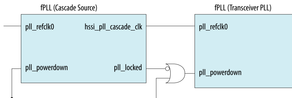
Figure 201. PLL Cascading
