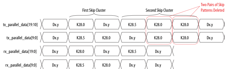
Figure 150. Rate Match FIFO Deletion with Four Skip Patterns Required for Deletion
