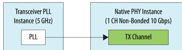
Figure 194. PHY IP Core and PLL IP Core Connection for Single Channel x1 Non-Bonded Configuration Example
