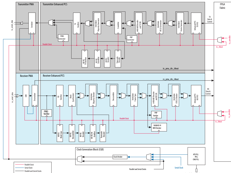
Figure 240. Enhanced PCS Datapath Diagram
