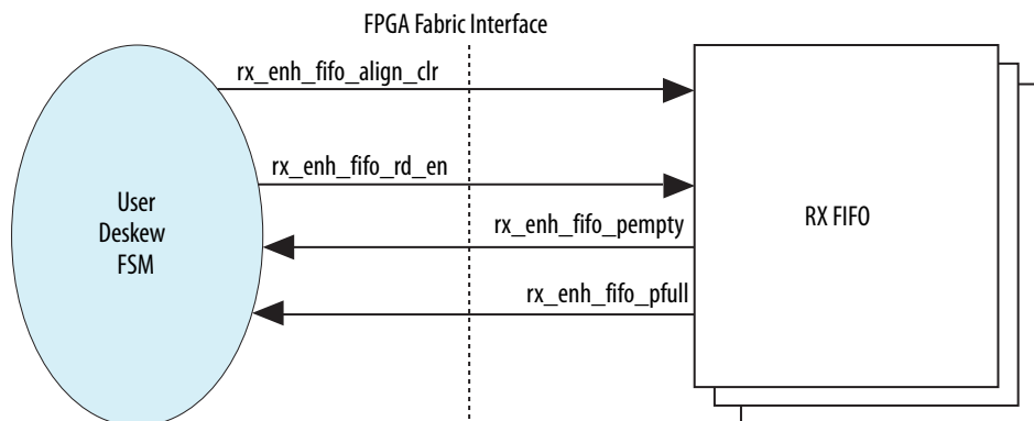
Figure 252. RX FIFO as Interlaken Deskew FIFO
