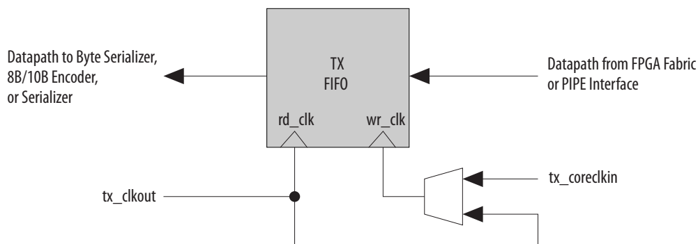
Figure 257. TX FIFO Block Diagram
