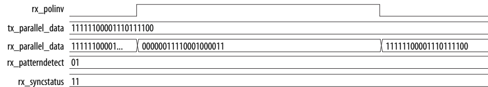
Figure 143. RX Polarity Inversion
