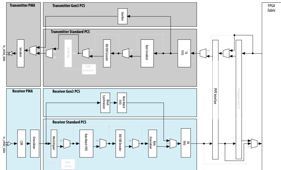
Figure 93. Transceiver Channel Datapath for PIPE Gen1/Gen2/Gen3 Configurations
