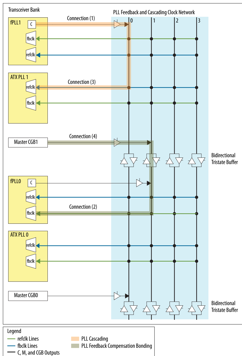
Figure 190. PLL Feedback and Cascading Clock Network
