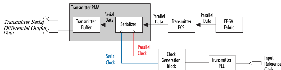
Figure 225. Transmitter PMA Block Diagram
