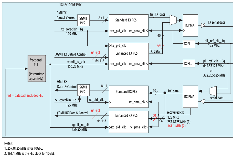
Figure 75. Clocks for Standard and 10G PCS and TX PLLs
