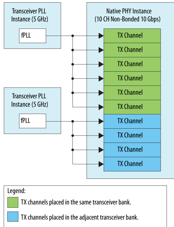
Figure 195. PHY IP Core and PLL IP Core Connection for Multi-Channel x1 Non-Bonded Configuration
