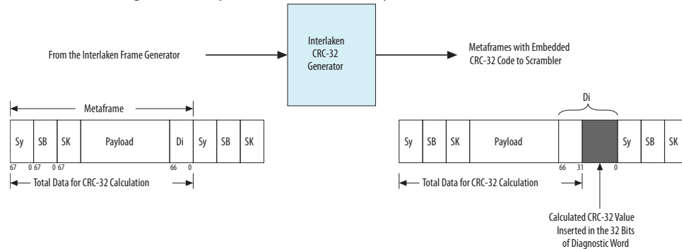
Figure 242. Interlaken CRC-32 Generator
