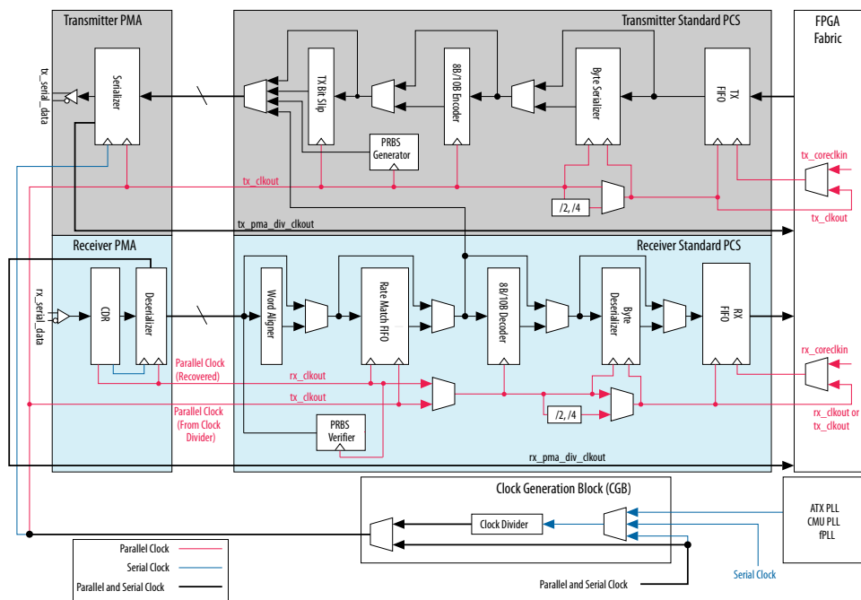
Figure 256. Standard PCS Datapath Diagram
