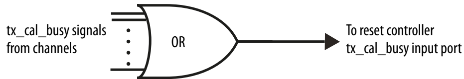
Figure 222. Combining Multiple PHY Status Signals
