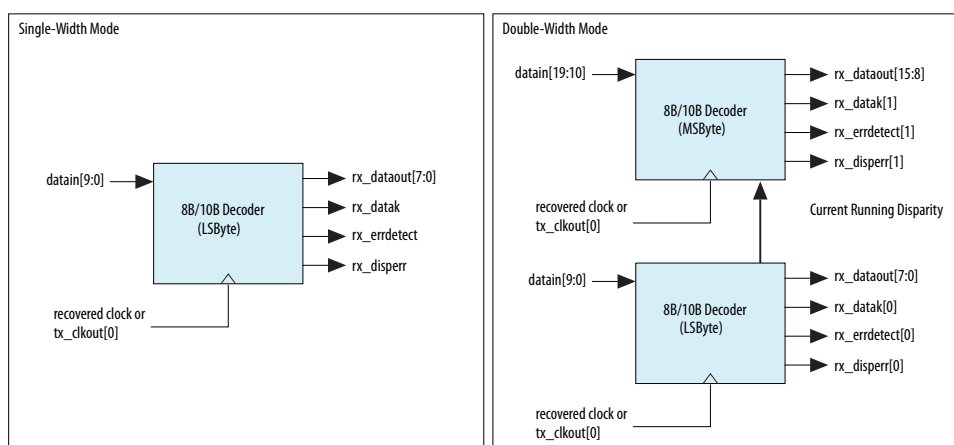
Figure 264. 8B/10B Decoder in Single-Width and Double-Width Mode
