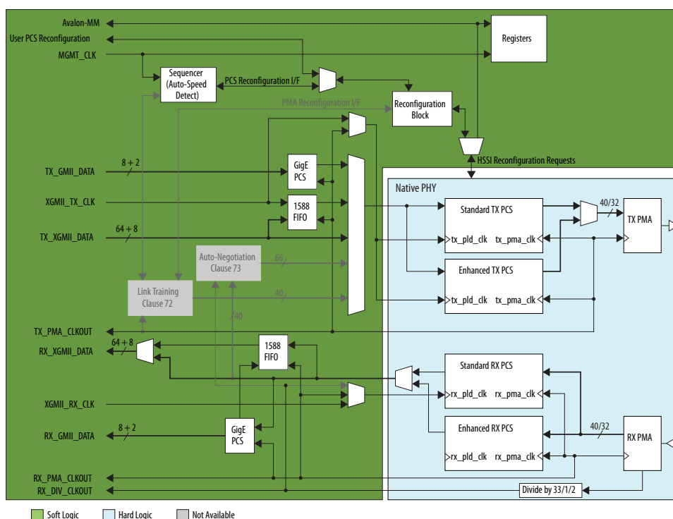
Figure 73. 1G/10GbE PHY Block Diagram
