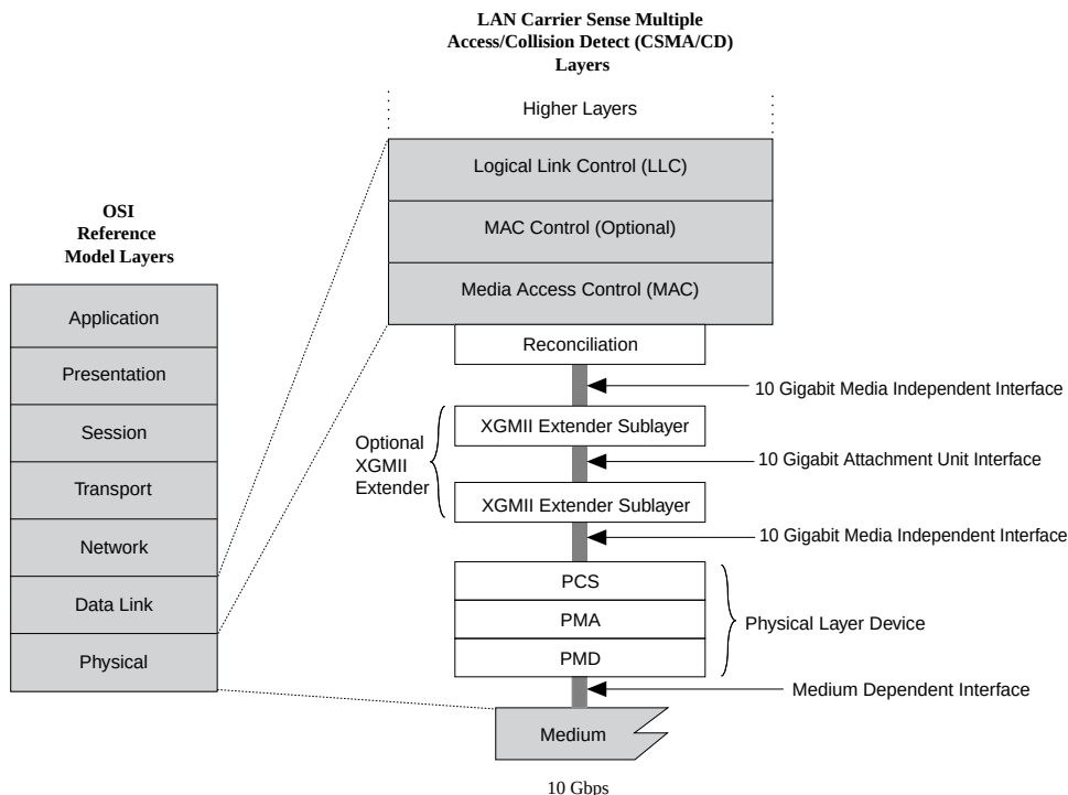
Figure 83. XAUI and XGMII Layers
