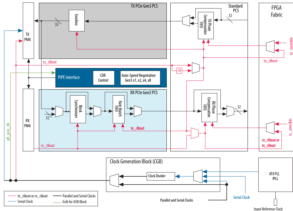
Figure 268. Gen3 PCS Block Diagram
