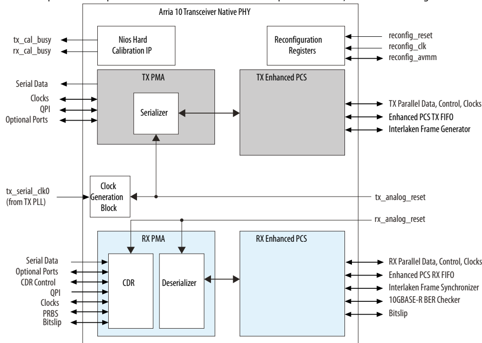
Figure 24. Enhanced PCS Interfaces
