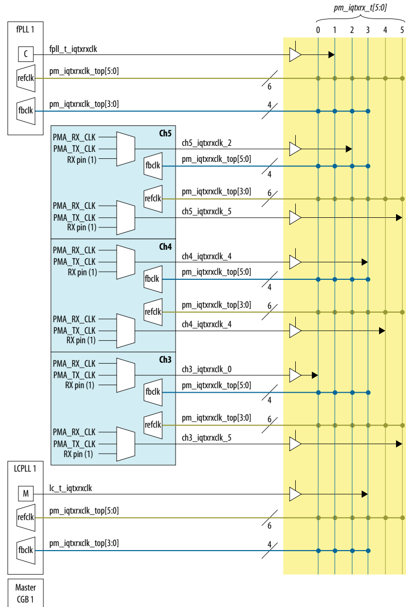
Figure 193. Integer Mode phase aligned and external feedback
