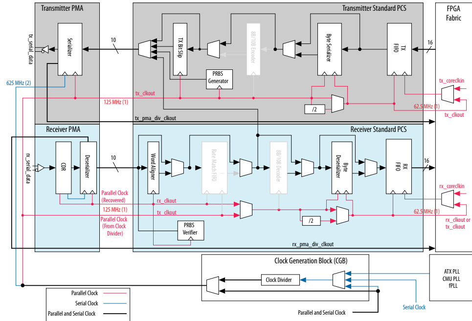
Figure 133. Transceiver Channel Datapath and Clocking for Basic Configuration with Low Latency Enabled
