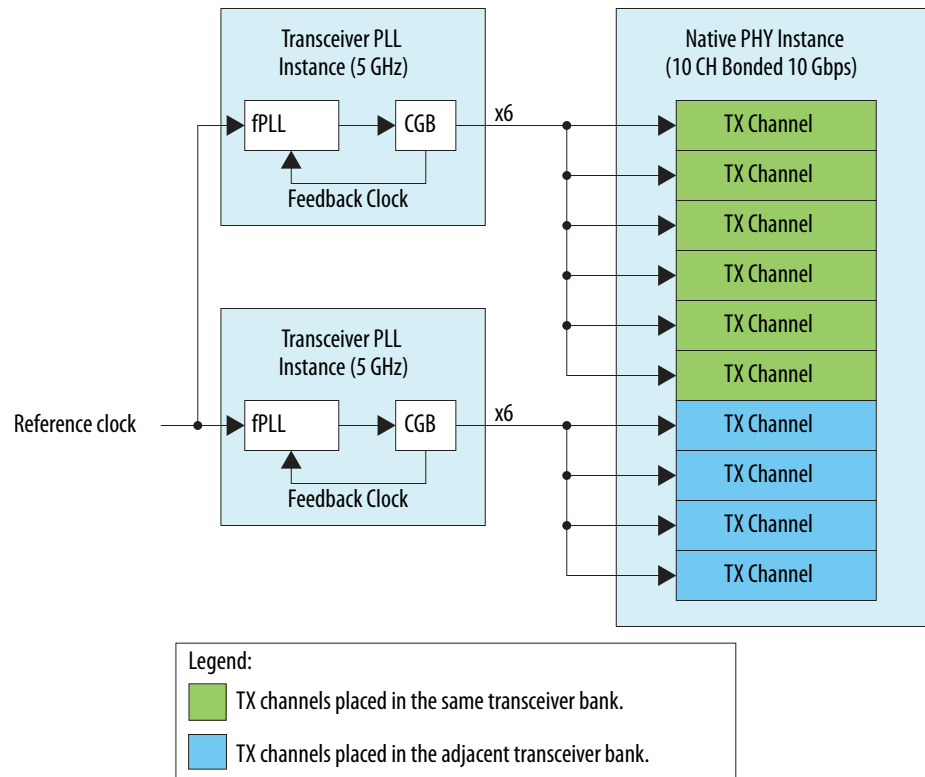
Figure 200. PHY IP Core and PLL IP Core Connection for PLL Feedback Compensation Bonding
