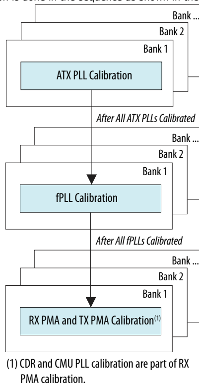
Figure 286. Power-up Calibration Sequence for Non-PCIe Hard IP (HIP) Channels
