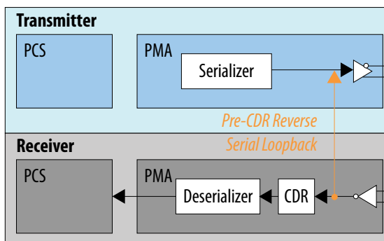
Figure 278. Reverse Serial Loopback Mode (Pre-CDR)
