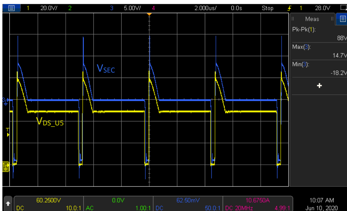
Figure 10.1. Si34071-FW-5V-C8 Output Short Protection Mechanism
