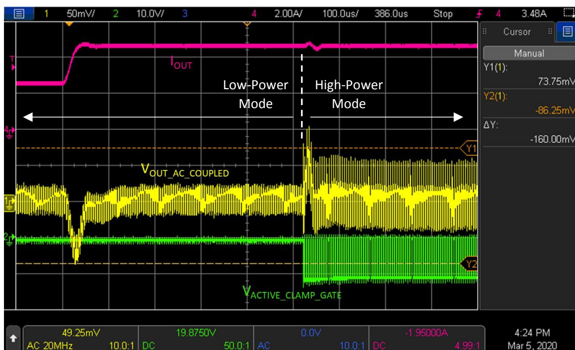
Figure 12.2. Low-Power Mode to High-Power mode transition ( I_{\text{OUT}} changes from 2.6 A to 4.7 A)
