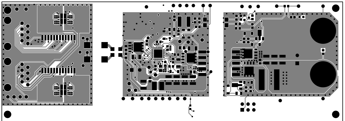
Figure 19.2. Top Layer
