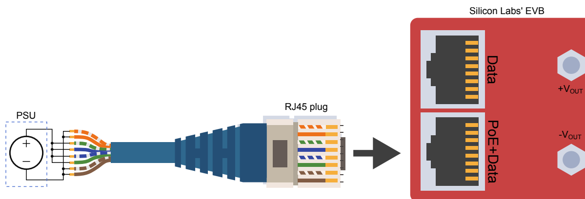
Figure 3.1. Four Pair Connection Using Laboratory Power Supply
