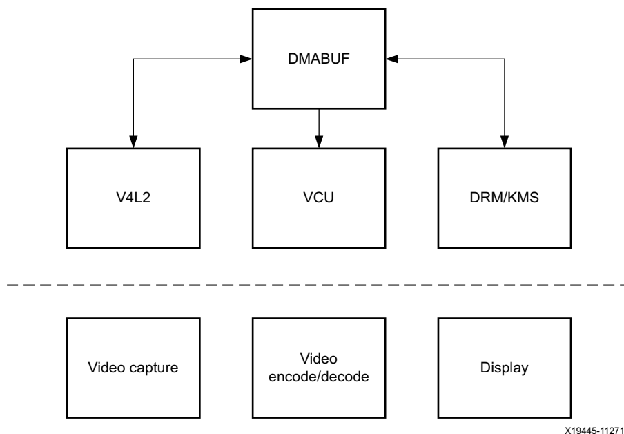
Figure 3-20: Buffer Sharing
