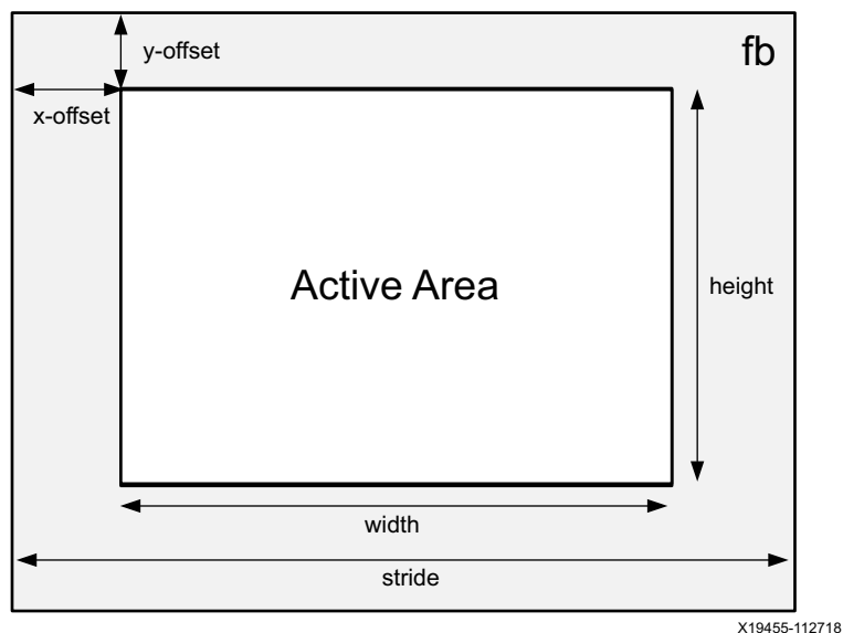
Figure 4-2: Video Buffer Area
