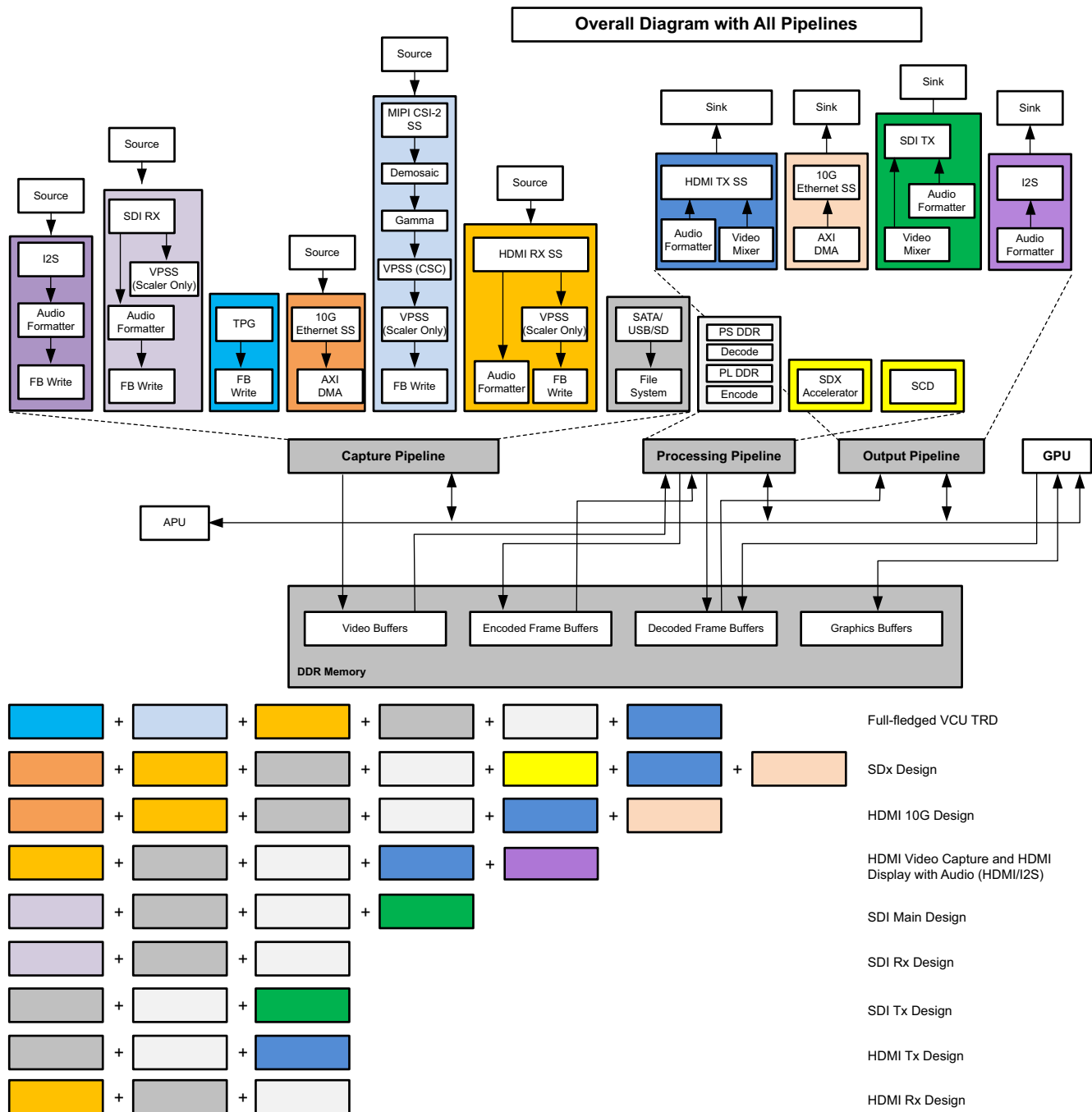
Figure 1-3: VCU TRD Block Diagram
