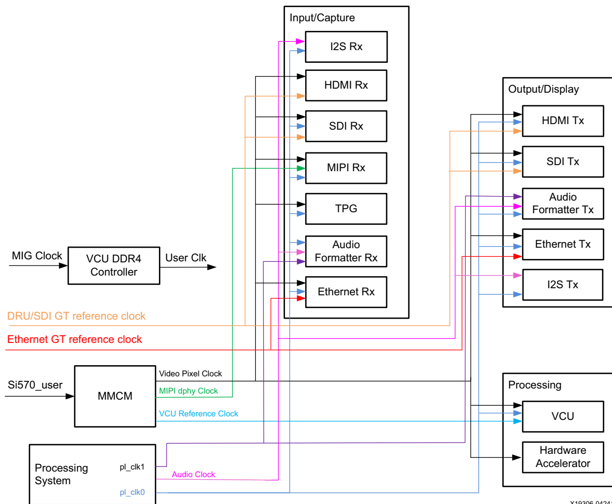
Figure 5-2: Clocking Mechanism for the TRD
