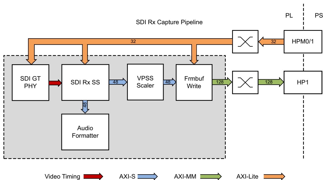
Figure 5-6: SDI RX Capture Pipeline
