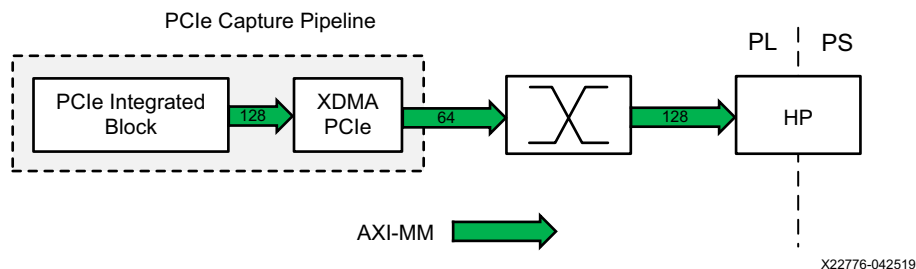
Figure 5-14: PCIe Capture Pipeline
