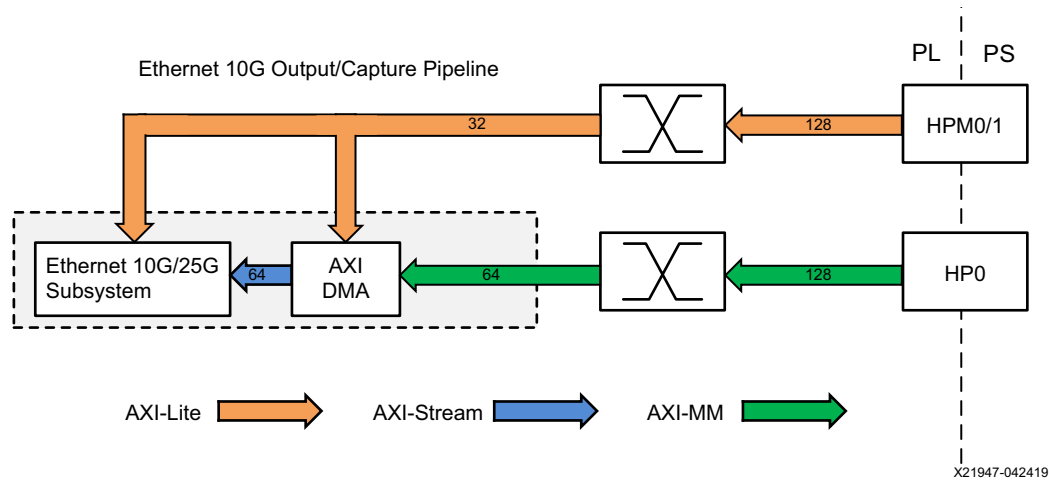
Figure 5-11: Ethernet 10G Output Pipeline
