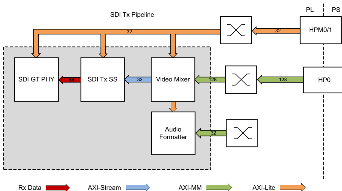
Figure 5-9: SDI TX Display Pipeline
