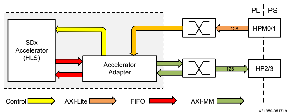
Figure 5-13: Accelerator Processing Pipeline
