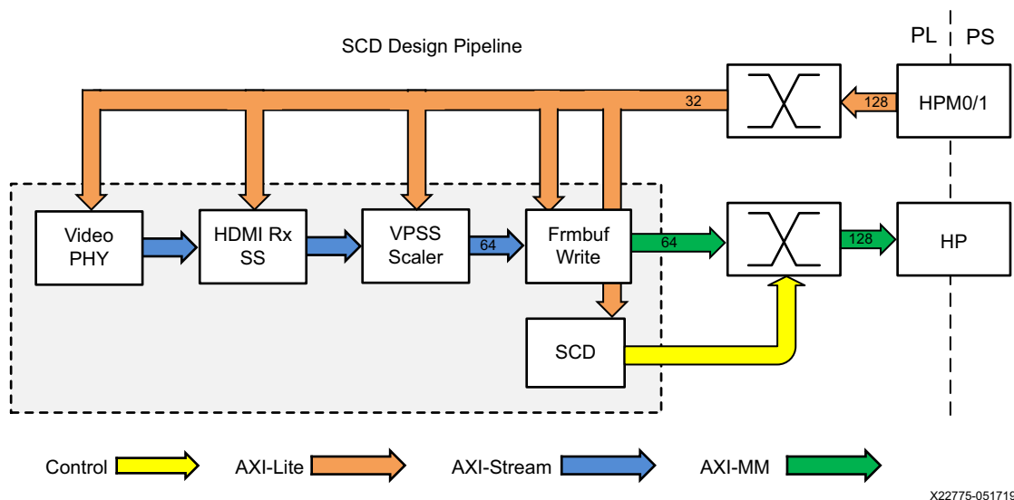
Figure 5-15: SCD Pipeline
