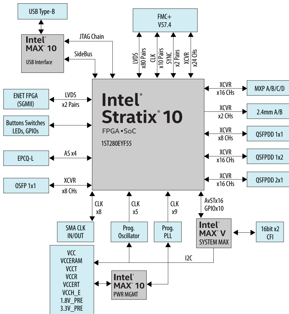
Figure 1. Intel Stratix 10 TX Development Kit Block Diagram
