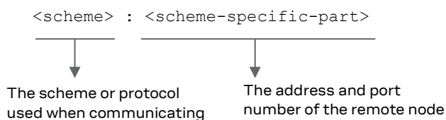
Figure 21: URL example
