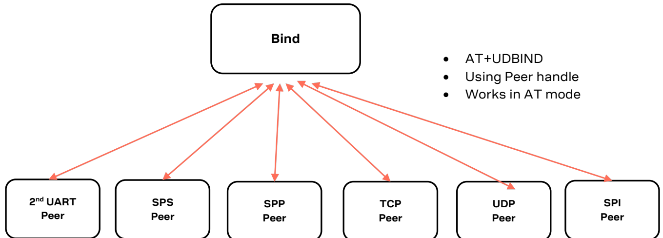
Figure 24: Bind functionality
