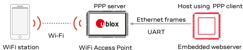
Figure 41: Example of a u-blox short range module acting as a Wi-Fi access point to provide network connectivity
