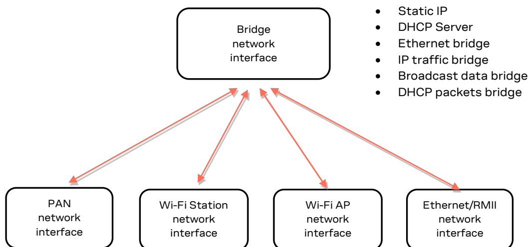
Figure 23: Bridge functionality
